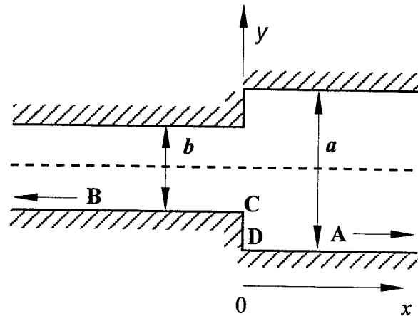
Figure 2.11 Section of a rectangular duct with sudden change of width in the y direction.
