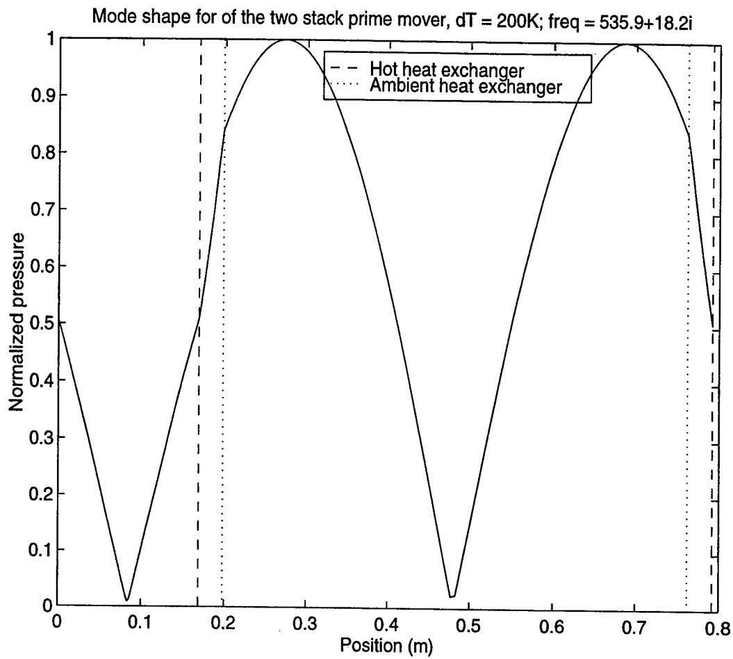
Figure 4.20 The calculated mode shape of the low mode of the two stack annular prime mover at \Delta T = 200\text{ K} . Case 2: The duct between the two hot heat exchangers is held at T_h = 493\text{ K} .
