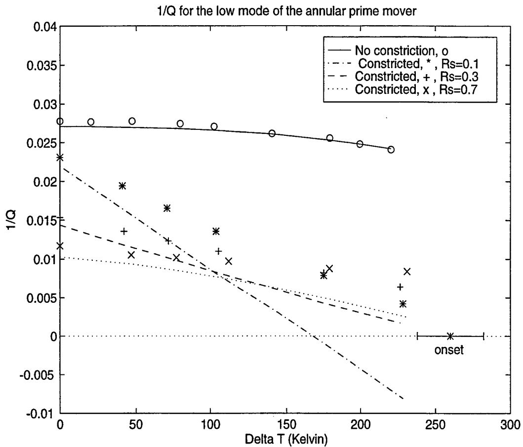
Figure 4.11 Comparisons of the measured and predicted 1/Q of the low mode for the unstricted and constricted prime mover. Symbol \circ represents the measured 1/Q of unstricted prime mover. Symbols * , + , and \times represent the measured 1/Q for the constricted prime mover with porosities of 0:1, 0.3, and 0.7, respectively. The lines represent the predicted values. No end corrections are included in the predicted values for the unstricted prime mover.
