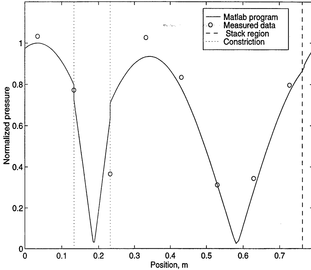
Figure F.1-22 Mode shape of the low mode of the constricted prime mover ( R_s=0.3 ) when the driver is located 45^\circ from the stack and \Delta T=0 K. The calculated results are based on the higher order mode method and the end corrections of the stack are included. The frequency is the calculated value.
