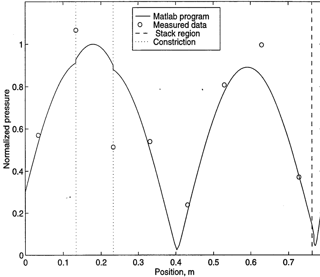
Figure F.1-24 Mode shape of the high mode of the constricted prime mover ( R_s=0.3 ) when the driver is located 45^\circ from the stack and \Delta T=0 K. The calculated results are based on the higher order mode method and the end corrections of the stack are included. The frequency is the calculated value.
