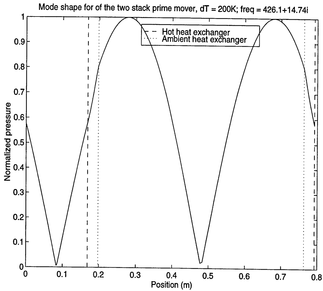
Figure 4.18 The calculated mode shape of the low mode of the two stack annular prime mover at \Delta T = 200\text{ K} . Case 1: The duct between the two hot heat exchangers is held at T_a = 293\text{ K} .
