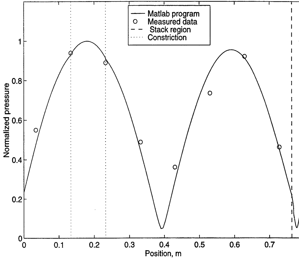
Figure F.1-28 Mode shape of the high mode of the constricted prime mover ( R_s=0.7 ) when the driver is located 45^\circ from the stack and \Delta T=0 K. The calculated results are based on the higher order mode method and the end corrections of the stack are included. The frequency is the calculated value.
