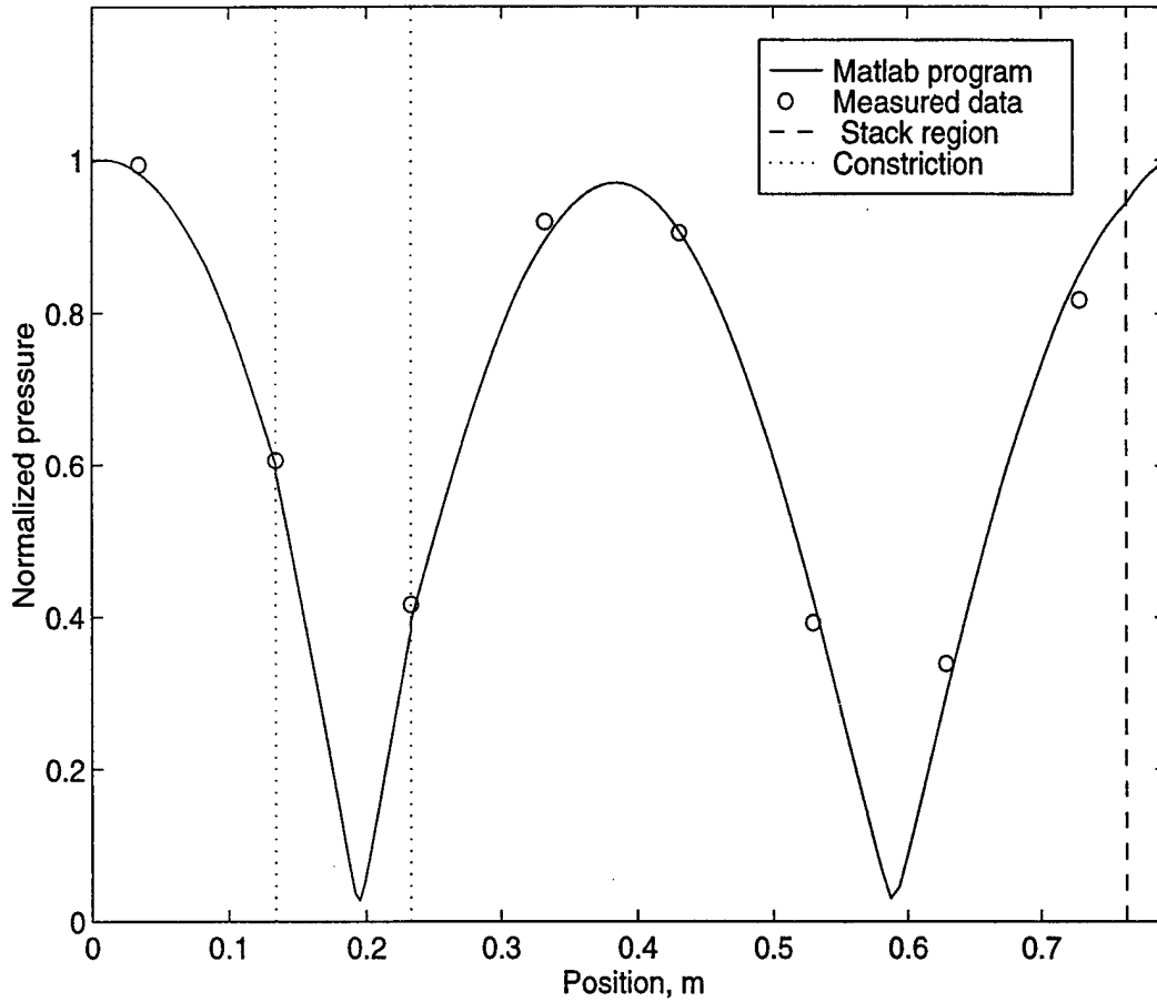
Figure F.1-6 Mode shape of the low mode of the constricted prime mover ( R_s=0.7 ) when the driver is located 45^\circ from the stack and \Delta T=77 K. The calculated results are based on the higher order mode method. The frequency is the calculated value.
