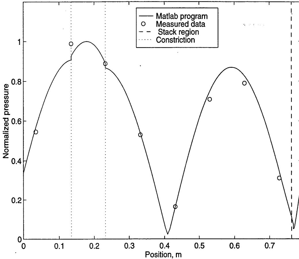
Figure F.1-20 Mode shape of the high mode of the constricted prime mover ( R_s=0.1 ) when the driver is located 45^\circ from the stack and \Delta T=0 K. The calculated results are based on the higher order mode method and the end corrections of the stack are included. The frequency is the calculated value.
