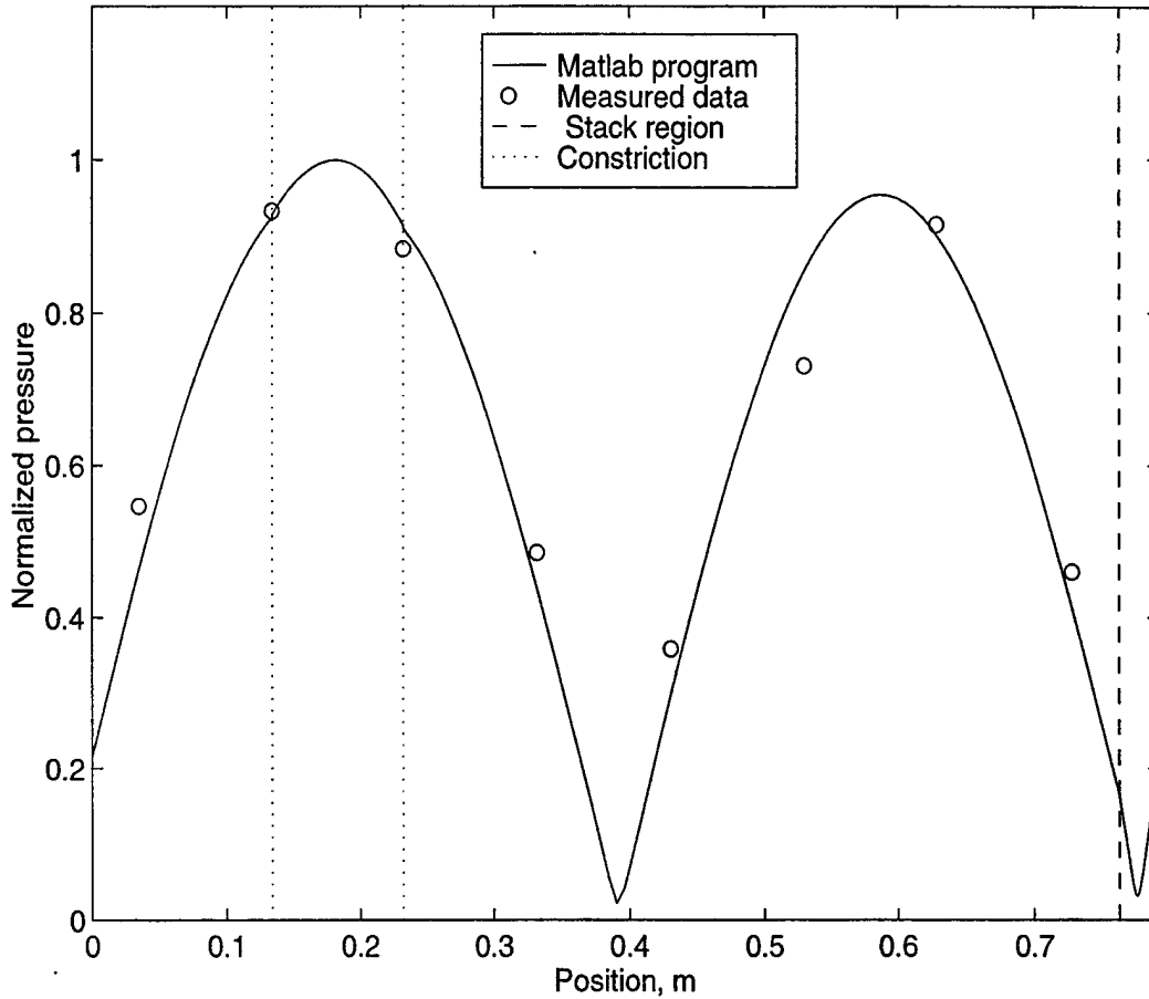
Figure F.1-8 Mode shape of the high mode of the constricted prime mover ( R_s=0.7 ) when the driver is located 45^\circ from the stack and \Delta T=0 K. The calculated results are based on the higher order mode method. The frequency is the calculated value.
