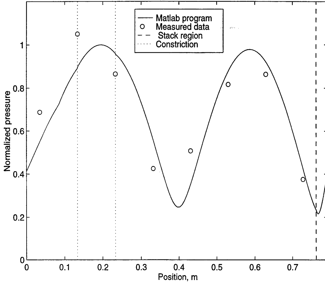
Figure F.1-10 Mode shape of the high mode of the constricted prime mover ( R_s=0.7 ) when the driver is located 45^\circ from the stack and \Delta T=231 K. The calculated results are based on the higher order mode method. The frequency is the calculated value.
