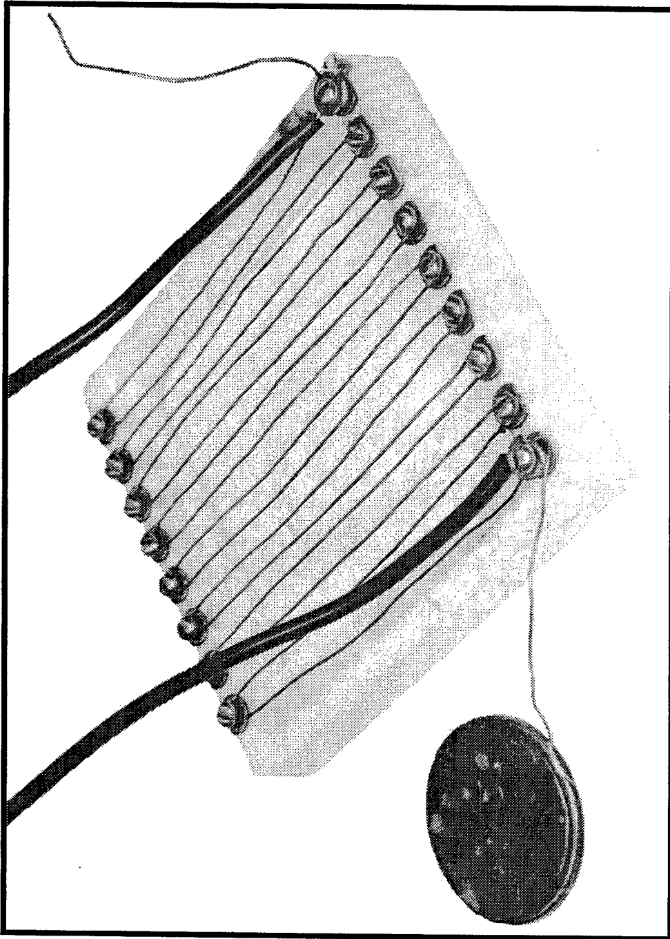
Figure 3.6 The hot heat exchanger assembly.
