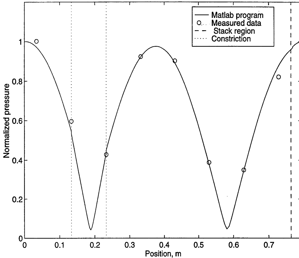
Figure F.1-26 Mode shape of the low mode of the constricted prime mover ( R_s=0.7 ) when the driver is located 45^\circ from the stack and \Delta T=0 K. The calculated results are based on the higher order mode method and the end corrections of the stack are included. The frequency is the calculated value.
