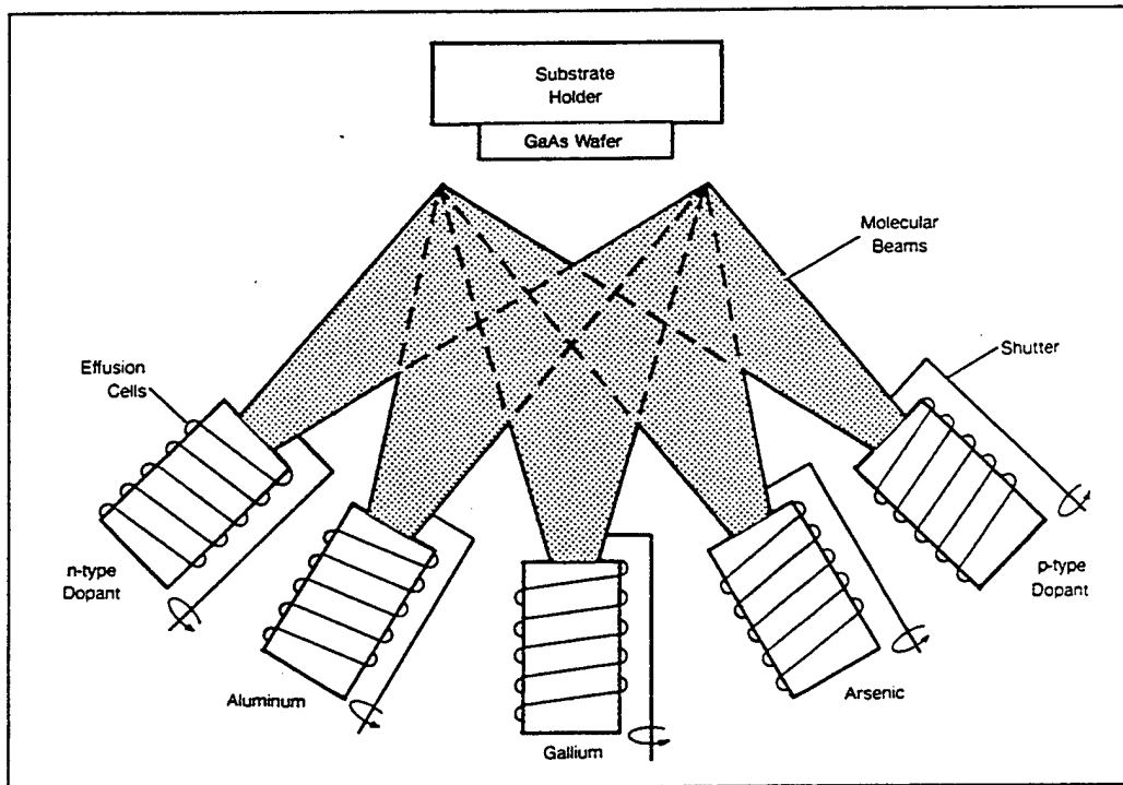
Figure 5 - Schematic of a molecular beam epitaxy system (MBE). From Ref. [5].
