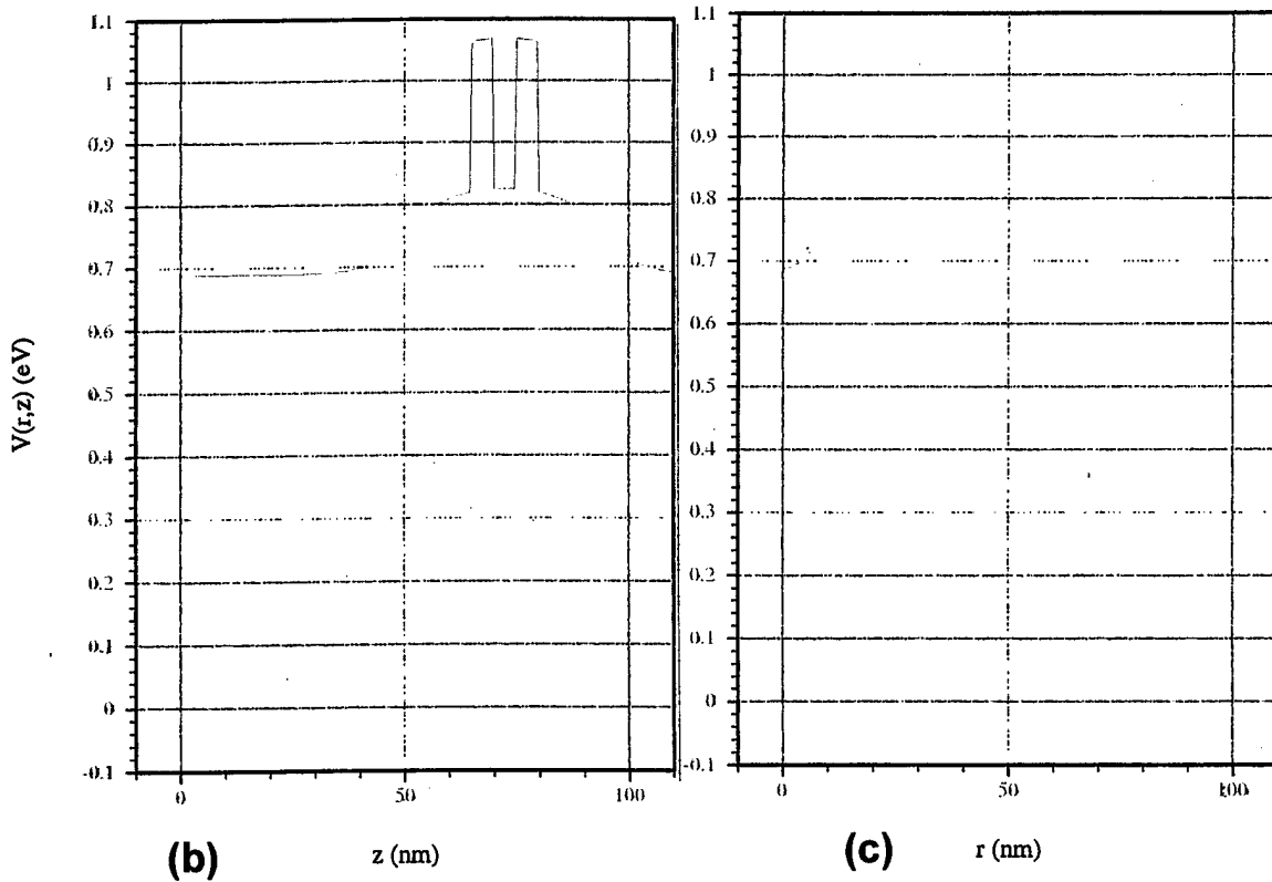
Figure 11 - Plot of a quantum dot with a radius of 10nm. All other variables are the same as Figure 10.
