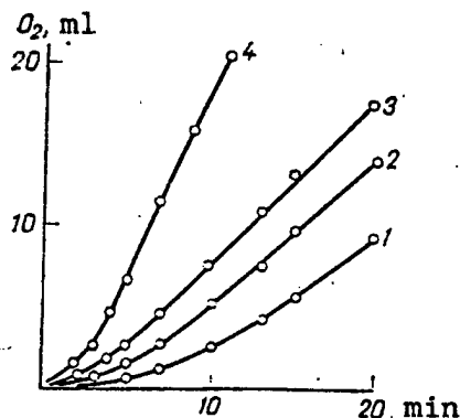
Figure 1. Kinetics of Oxygen Release in the H 2 O-HCl-H 2 O 2 -Siderite System: 1,2,3,4—solution pH values of 1.7, 2.02, 2.54 and 3.0 in the presence of 1.5 M H 2 O 2 and 0.5 g siderite.
