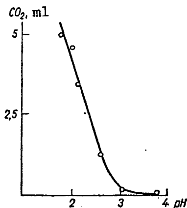
Figure 2. Effect of pH on Release of Carbon Dioxide in the H 2 O-HCl-H 2 O 2 -Siderite System: Content of components—1.5 M H 2 O 2 and 0.5 g siderite; reaction time—30 min.
