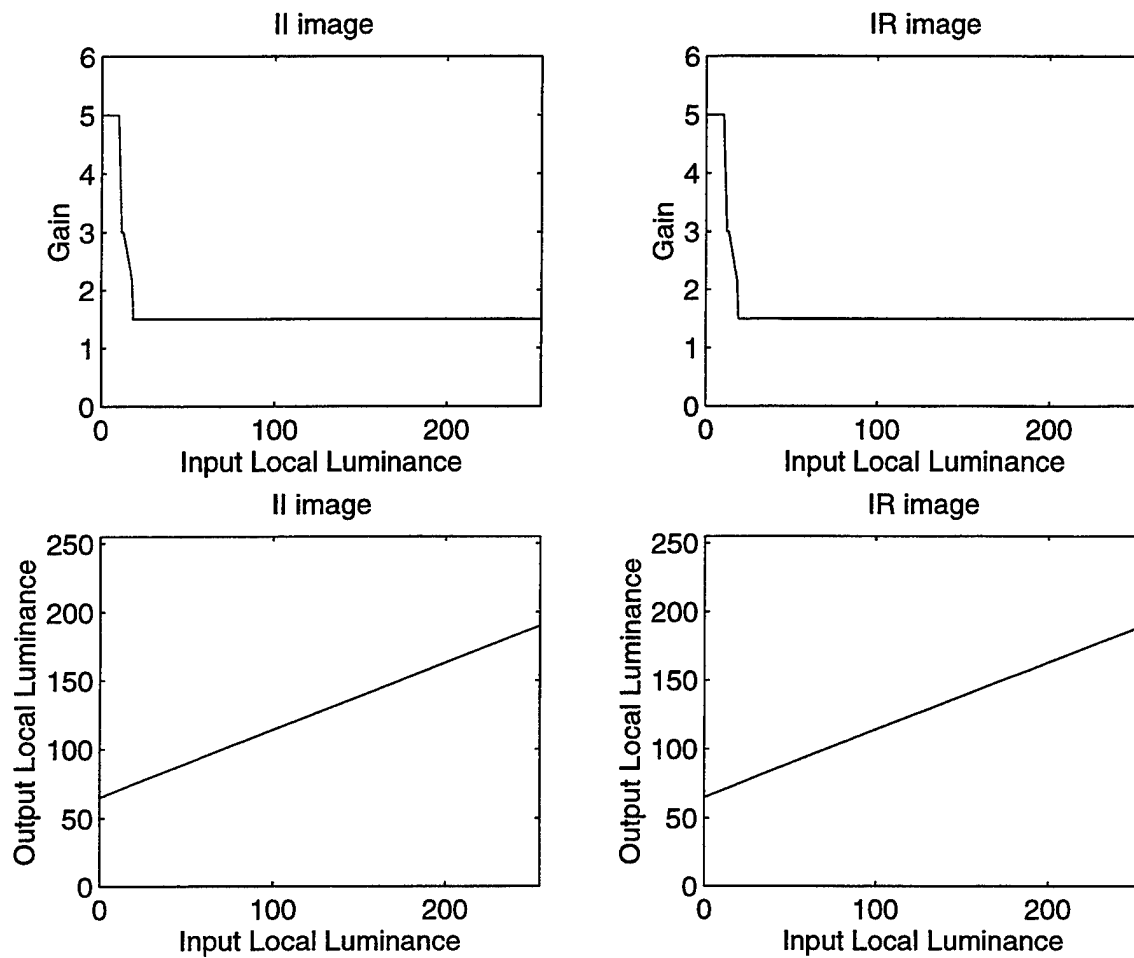
Figure 41. Gain and Local Luminance Transformation Curves for Scene 5
