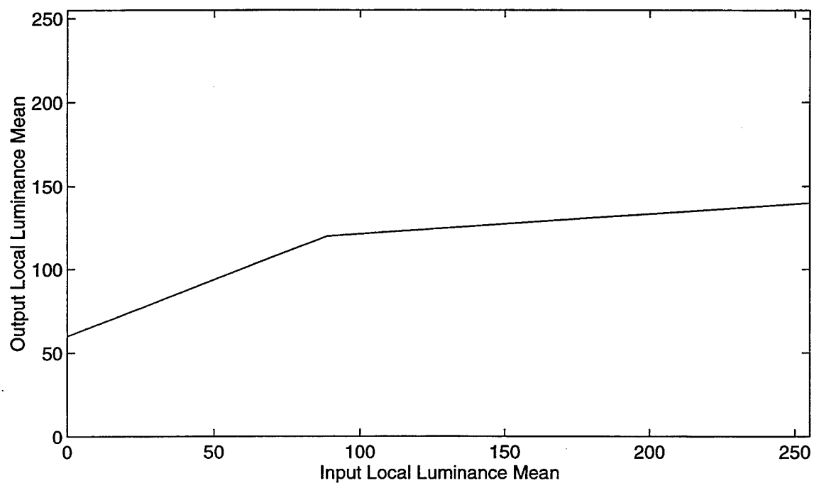
Figure 14. Gain ( K ) and Local Luminance Transformation ( NL ) Curves for Enhancement of an Image Degraded by Cloud Cover [Ref. 8]
