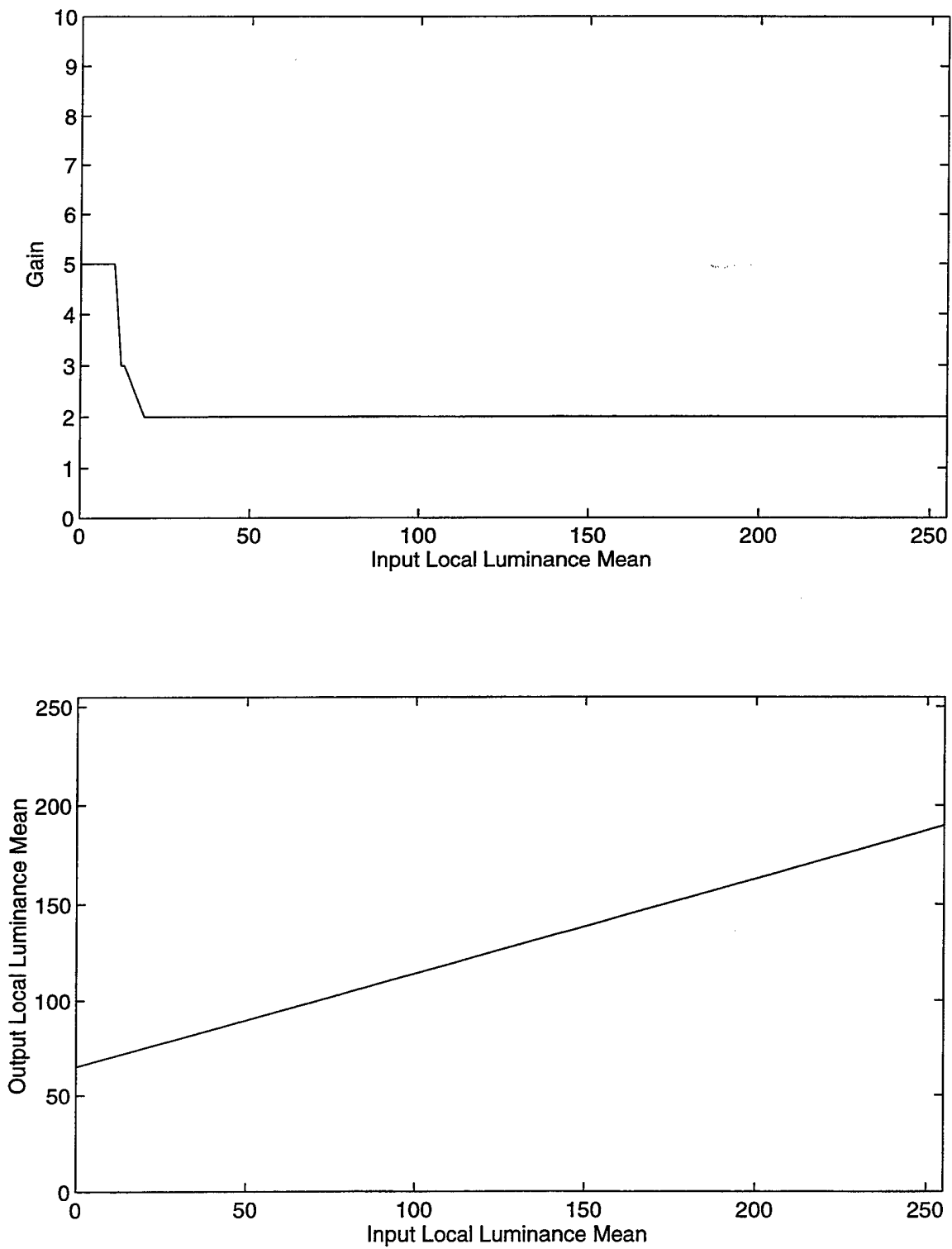
Figure 15. Gain ( K ) and Local Luminance Transformation ( NL ) Curves for Enhancement of an Image Degraded by Shadow Regions [Ref. 8]
