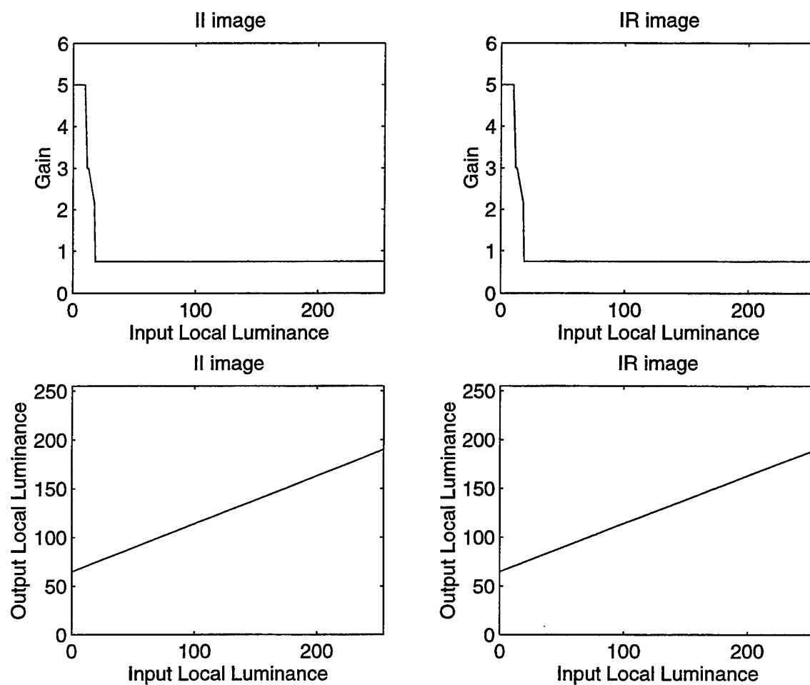
Figure 39. Gain and Local Luminance Transformation Curves for Scene 3
