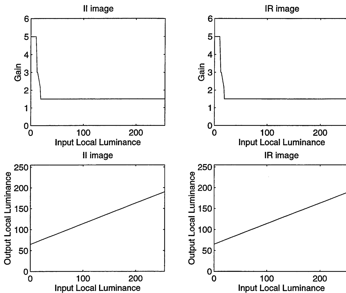
Figure 37. Gain and Local Luminance Transformation Curves for Scene 1
