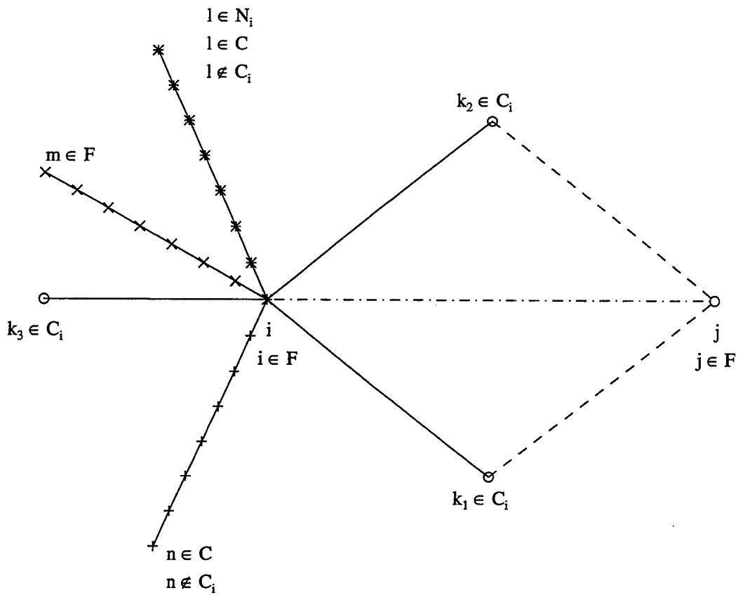
Figure 13. Illustration of the neighborhood ( N_i ) of a fine grid point i and its relationship to other fine and coarse-grid points in the matrix. For each point i , N_i is divided into four distinct groups.
