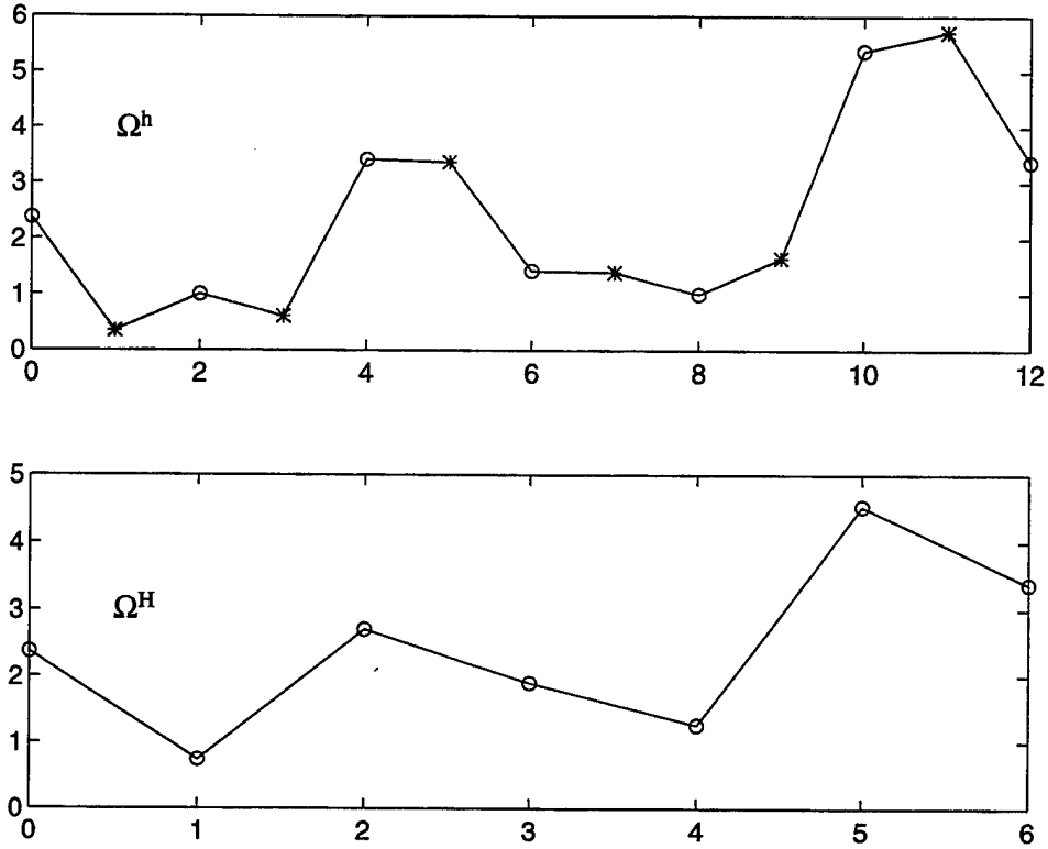
Figure 7. Restriction by full weighting on a arbitrary vector from \Omega^h to \Omega^H . The circles (o) on \Omega^H are the coarse-grid points and are weighted averages of neighboring fine grid point values.
