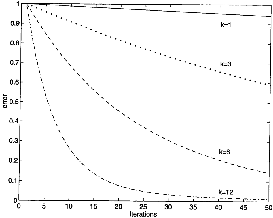
Figure 4. The weighted Jacobi iteration with \omega = 2/3 applied to the 1-D “model” problem with N = 64 and with initial guesses v_1, v_3, v_6, v_{12} . \|e\|_\infty is plotted against the iteration number for 50 iterations.
