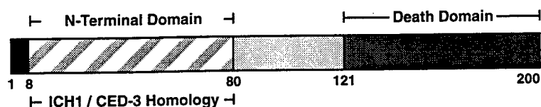
Deduced amino-acid sequence of RAIDD and schematic representation of the domain structure.
