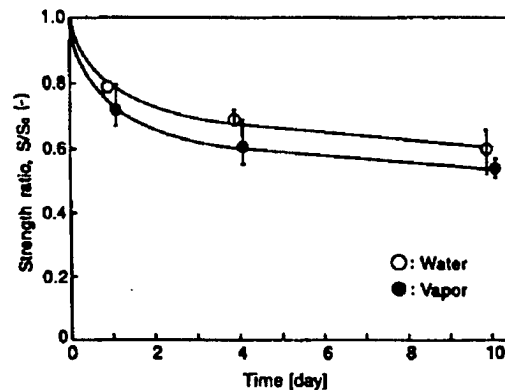
Figure 2. Bending Strength Vs. Exposure Time for \text{Si}_3\text{N}_4 Corroded in Water and Steam at 300°C
