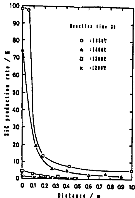
Figure 1. SiC Gradient of SiC/C Materials
