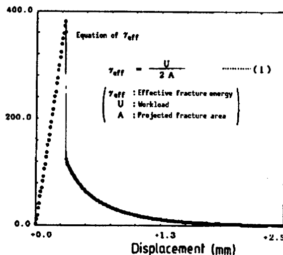
Figure 1. Typical P-u Relation of Tensile Test
