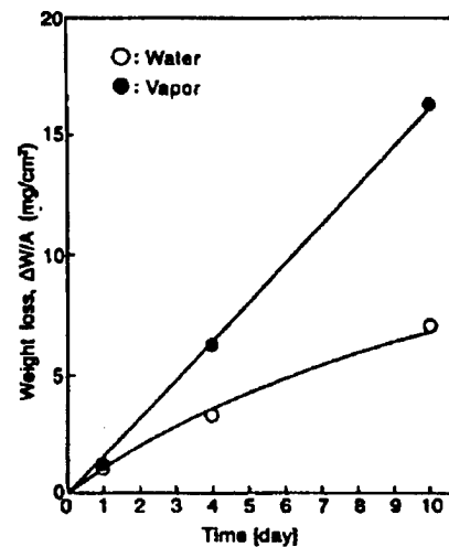
Figure 1. Weight Loss Vs. Exposure Time for \text{Si}_3\text{N}_4 Exposed to Water and Steam at 300°C
