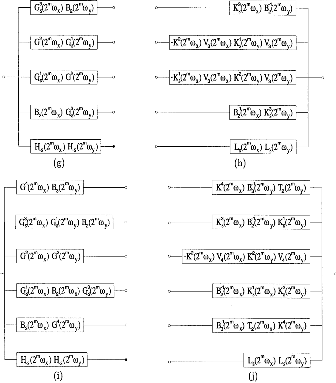
Figure 12: Continued: (g) Decomposition and (h) reconstruction modules for d = 3 , and (i) decomposition and (j) reconstruction modules for d = 4 . Decomposition modules are recursively applied at the locations of the filled circles.
