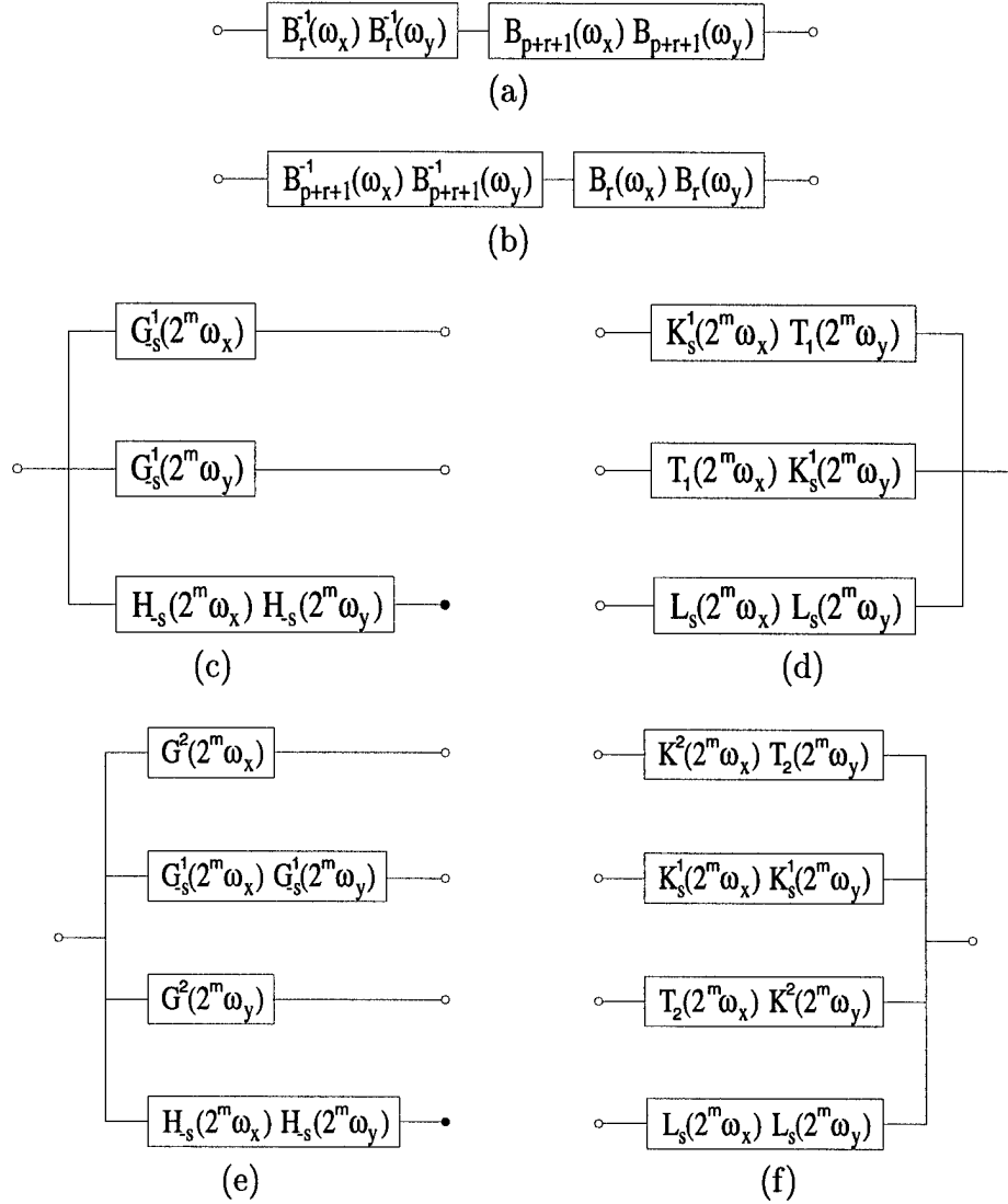
Figure 12: Filter bank implementation of a multiscale spline derivative-based transform for m \in [0, M - 1] : (a) Prefiltering, (b) postfiltering, (c) decomposition and (d) reconstruction modules for d = 1 , and (e) decomposition and (f) reconstruction modules for d = 2 .
