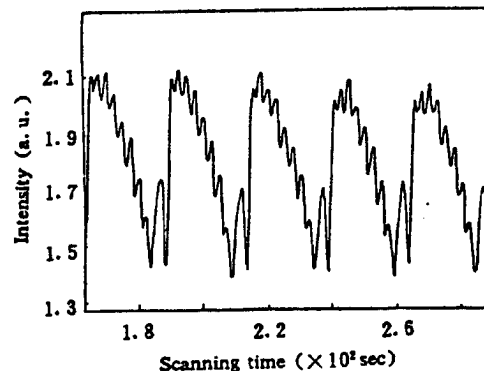
Figure 8. The Stability of Photon-Gated Spectral Hole Burning Was Detected by Repeated Scanning of 3 GHz/25 sec of the Laser Over the Burning Range
