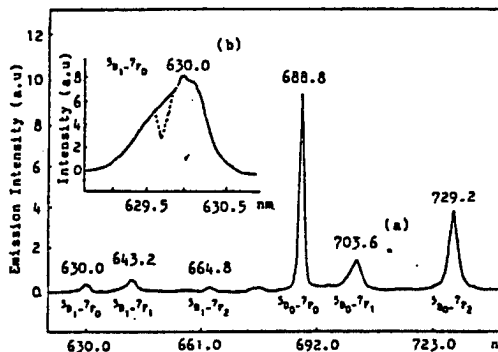
Figure 3. (a) Fluorescence spectra of \text{BaFCl}_{0.5}\text{Br}_{0.5}\text{Sm}^{2+} at 4 K. (b) Excitation spectra of ^7\text{F}_0\text{-}^5\text{D}_1 transition before (solid line) and after (dotted line) gated hole burning with dye laser line width of 7.6 GHz
