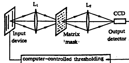
Figure 2. Schematic Drawing of the Optical System Used for Optical Experiments. L_1 and L_2 are imaging lenses.
