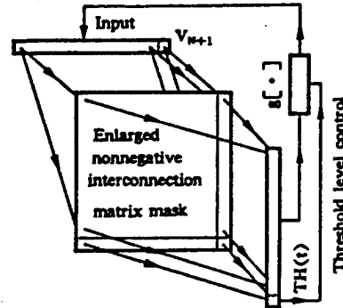
Figure 1. Optical Configuration for the Implementation of a Bipolar Neural Network in a Vector-Matrix Multiplier V_{N+1} Represents the Additional Input Dimension, and the (N+1) th Expected Output, TH(t) , Serves as the Dynamic Threshold Level
