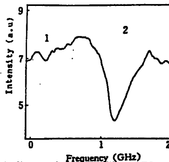
Figure 4. A Comparison of a Single-Photon Burning With Photon-Gated Hole Burning Showing a Gating Ratio of 30
