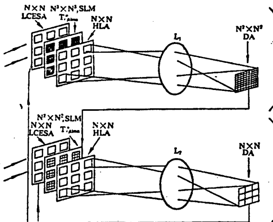
Figure 2. Schematic of Entire System; LCESA = liquid-crystal electro-optical switching array, DA = detector array.
