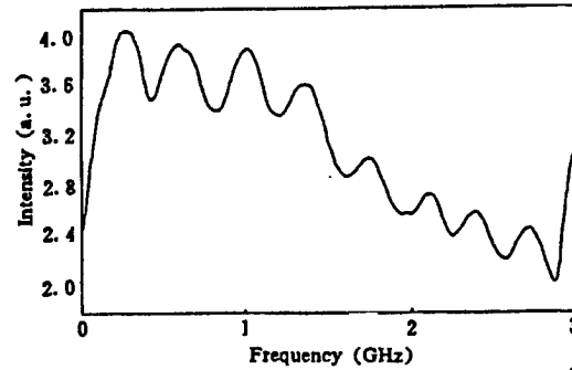
Figure 7. Eight Holes Burned in One of Sides of ^5D_1 - ^7F_0 Transition Profile
