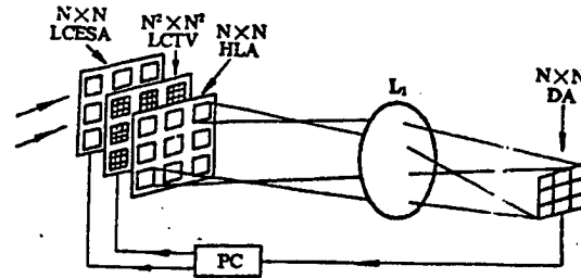
Figure 3. Time-Division Processing Method for System
