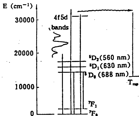
Figure 1. Schematic Energy-Level Diagram for \text{BaFCl}:\text{Sm}^{2+} Showing Hole-Burning Scheme for Some 4f Excited Electronic States and Indicating Scheme Principle Emission Detected During Read-Out for Each
