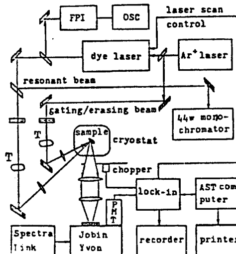
Figure 2. Schematic Illustration of Experimental Arrangement for Hole Burning and Detection
