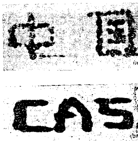
Figure 2. Characters and Designs With Line Width About 10 nm Etched With a Pulse Voltage Amplitude of About -4.5 V and Width of 8 ms. (a) The two etched characters "Zhong Guo," character size: 200 nm x 200 nm. (b) The English letters "CAS," letter size: 60 nm x 60 nm
