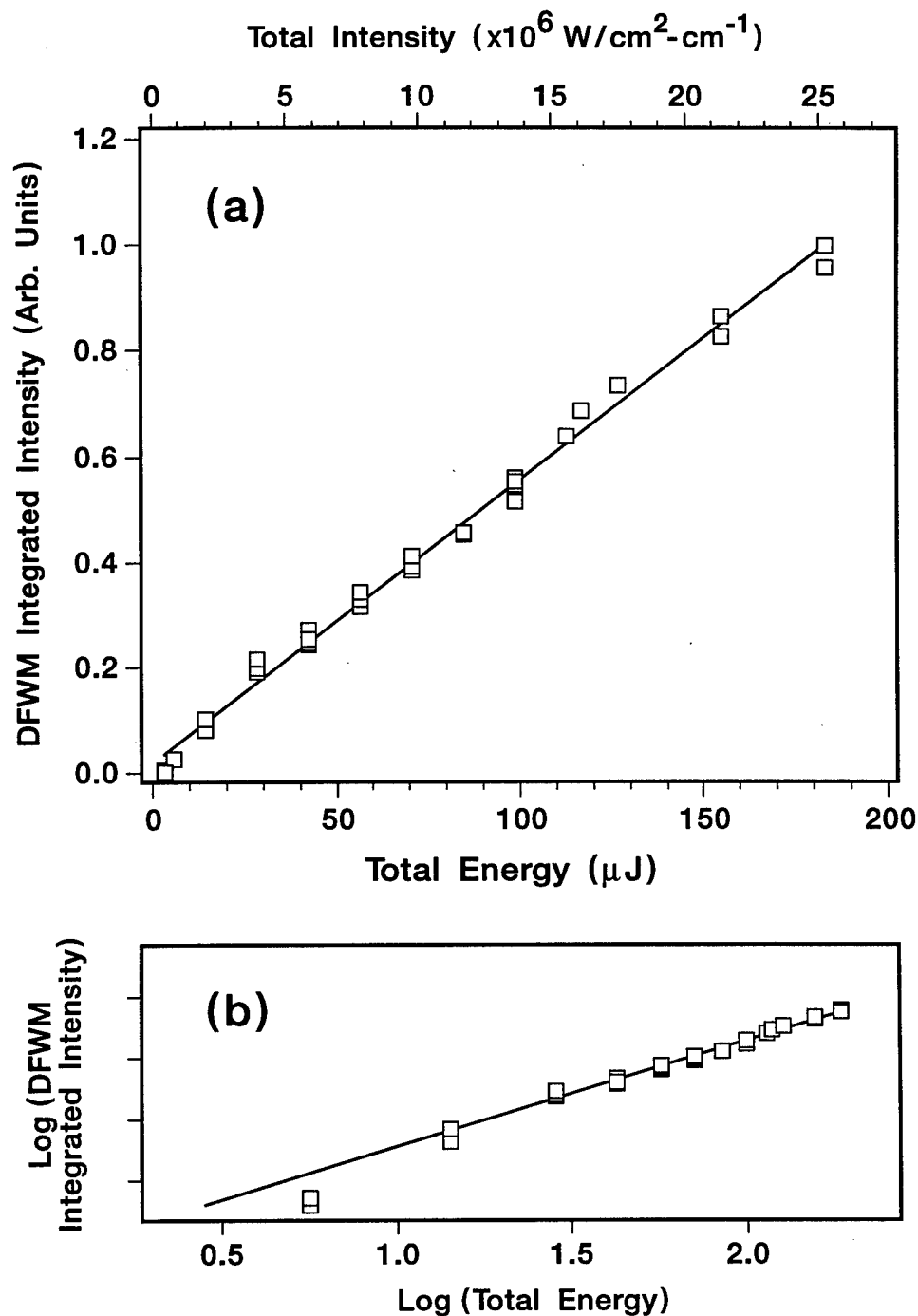
FIG. 2.5. (a) DFWM integrated signal intensity as a function of total laser energy (bottom) and spectral intensity (top), and (b) \text{Log}[\text{DFWM integrated intensity}] vs. \text{Log}[\text{total energy}] . The DFWM integrated signal intensity is linear over a large range of laser energies. The slope of the line in (b) resulting from a linear least squares fit of the data between 28.1 and 154.7 \mu\text{J} ( 3.9 and 21.3 \times 10^6 \text{ W/cm}^2\text{-cm}^{-1} ) is 0.87 \pm 0.07 corresponding to an average power dependence in this region of I_{\text{DFWM}} \propto I^{0.9} .
