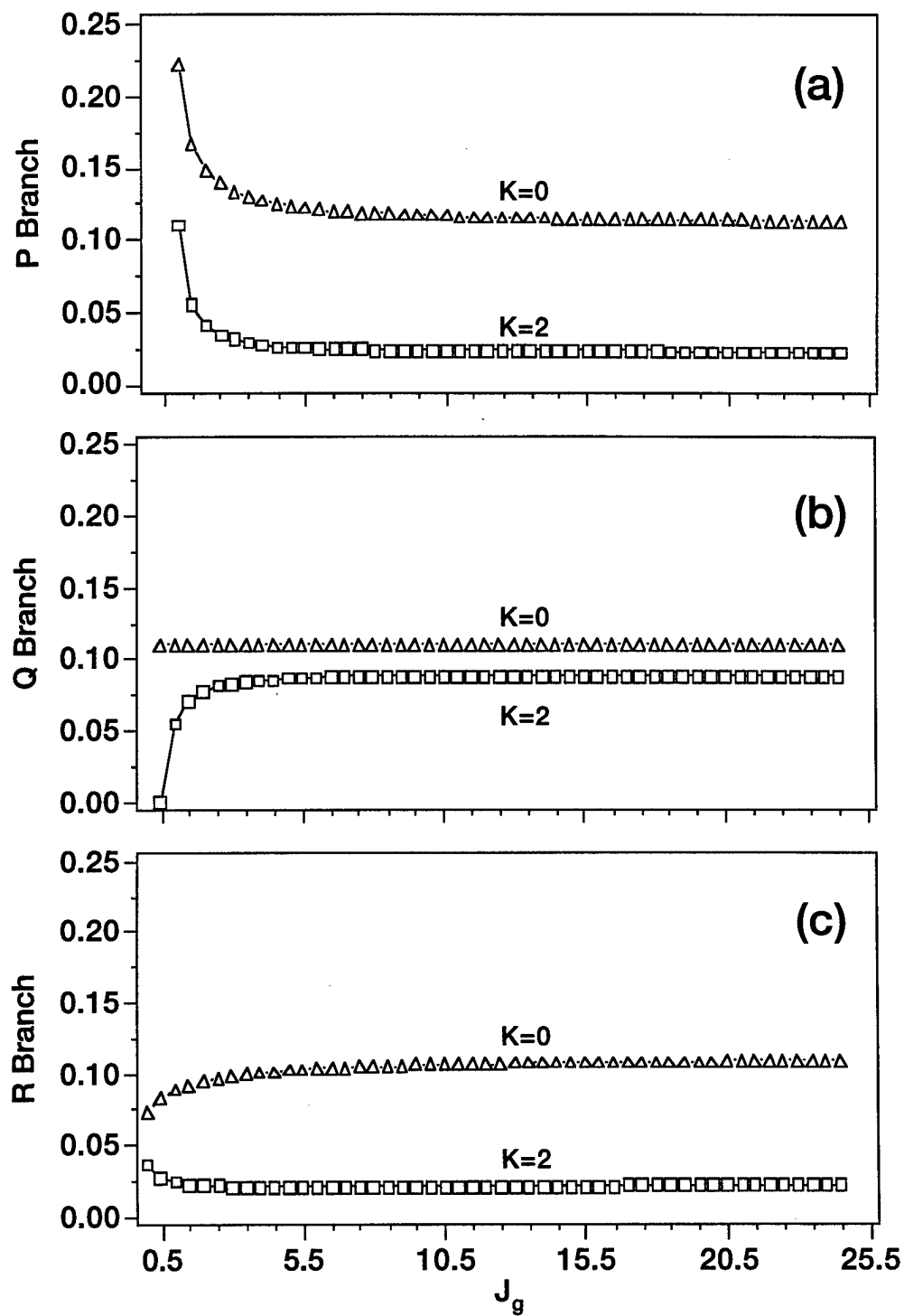
FIG. 3.5. Evaluated G_F^{T(K)}(Y, Y, Y, Y; J_g, J_e; \omega) factors as a function of J_g for (a) P-branch, (b) Q-branch, and (c) R-branch transitions. Permuting X \leftrightarrow Y does not change the plots. In the figure -\Delta- and -\square- correspond to K = 0 and 2, respectively.
