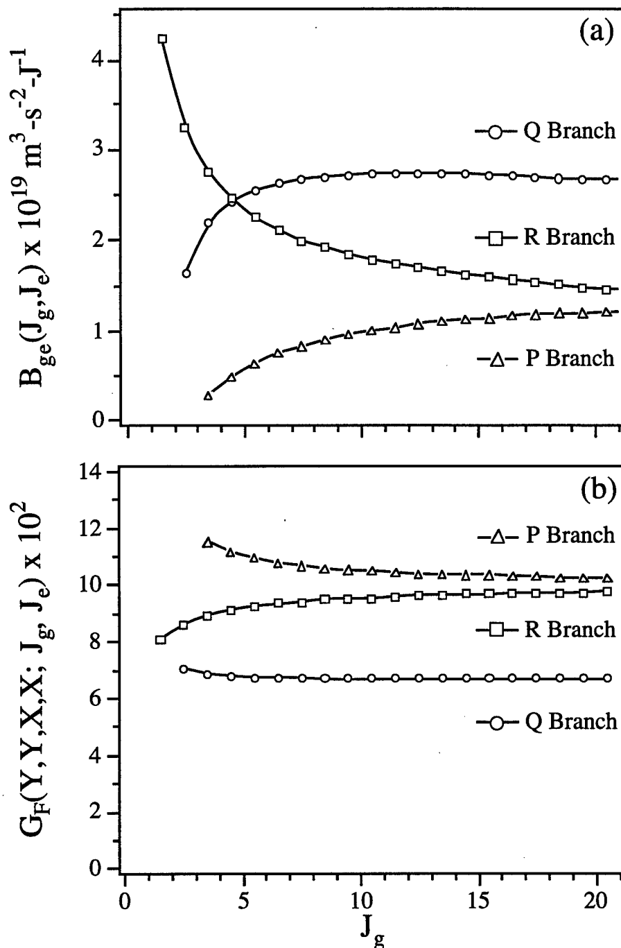
FIG. 4.9. (a) The Einstein absorption coefficients as a function of J_g for the R_1 -, Q_1 -, and P_1 -branch transitions of CH labeled \square -, \circ -, and \triangle -, respectively. The absorption coefficients for the R_2 -, Q_2 -, and P_2 -branch transitions are nearly the same because both the X and A states rapidly approach Hund's case (b) coupling as rotation increases. (b) Total geometric factors of Table 3.2 for the YYXX polarization configuration as a function of J_g with the same conventions as (a).
