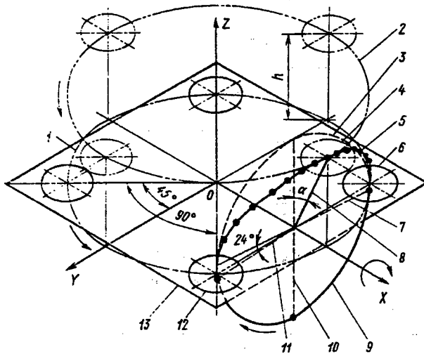
Figure 2. Axonometric Oblique-Angled Projection Drawing of Periodic Mutual-Contact Coupling and Foreshortened Trajectory of Drive's Driving Ball and Separator's Driven Diaphragm
