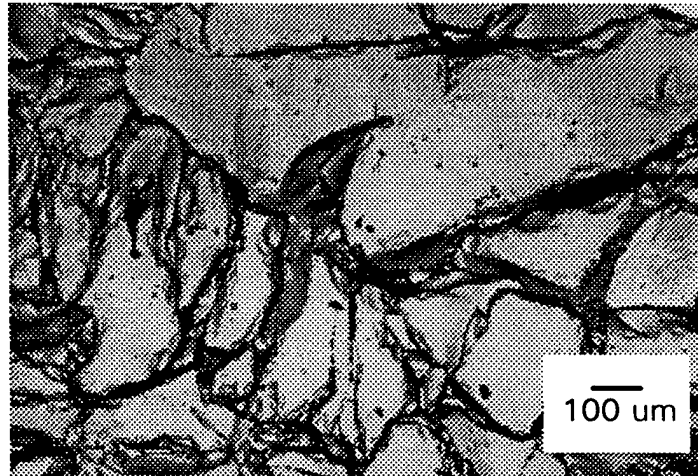
Figure 2: BEI of \text{Ti}_5\text{Si}_3 hot pressed at 1580°C for 4 hours at 34 MPa in vacuum.
