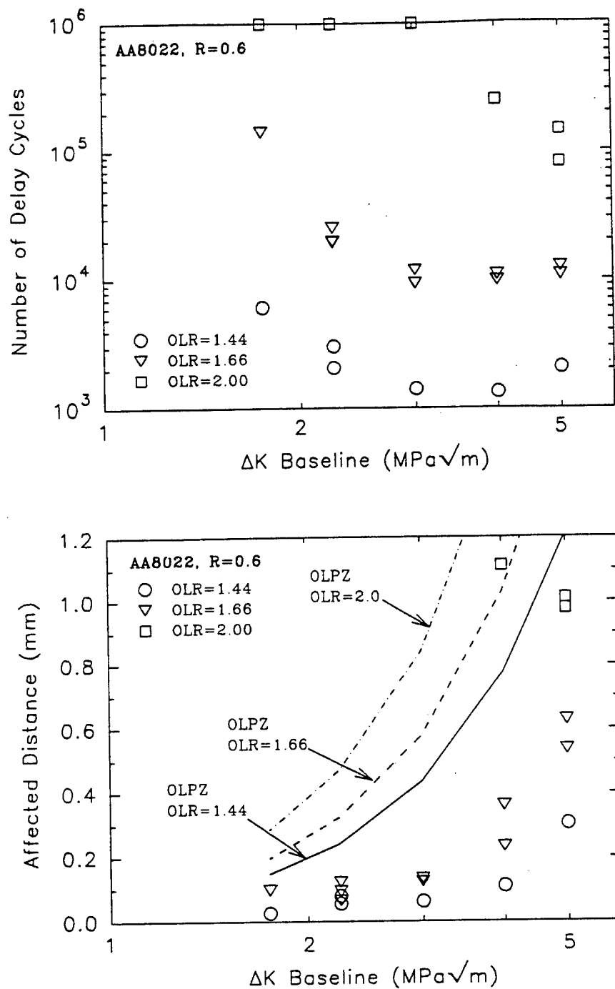
Figure 4.21. Magnitude of crack retardation in AA8022 at R=0.6 as a function of \Delta K_B (OLPZ=calculated overload plastic zone size).
