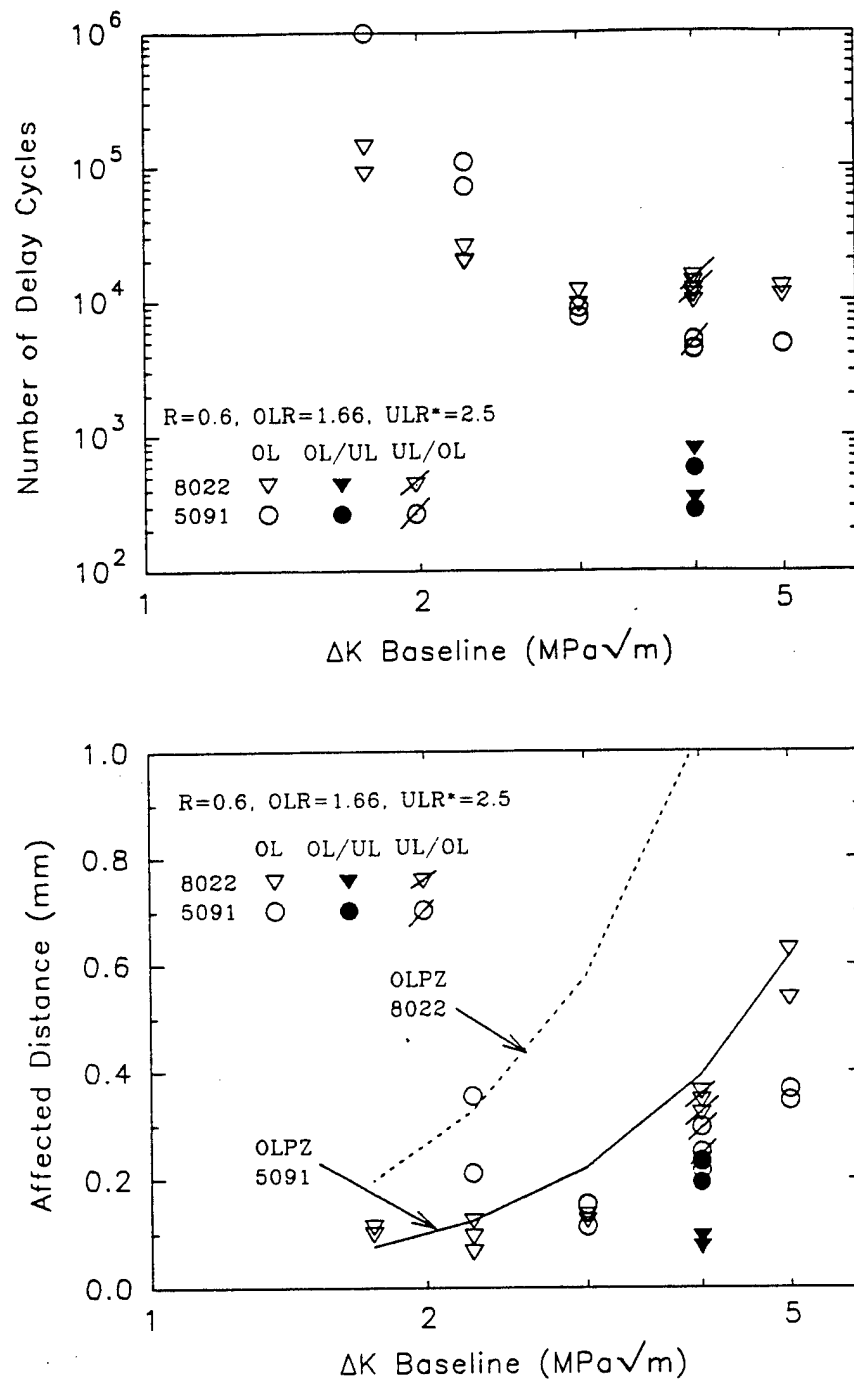
Figure 4.25. Comparison of retardation magnitude ( OLR=1.66 ) in AA5091 and AA8022 at R=0.6 (OLPZ=calculated overload plastic zone size).
