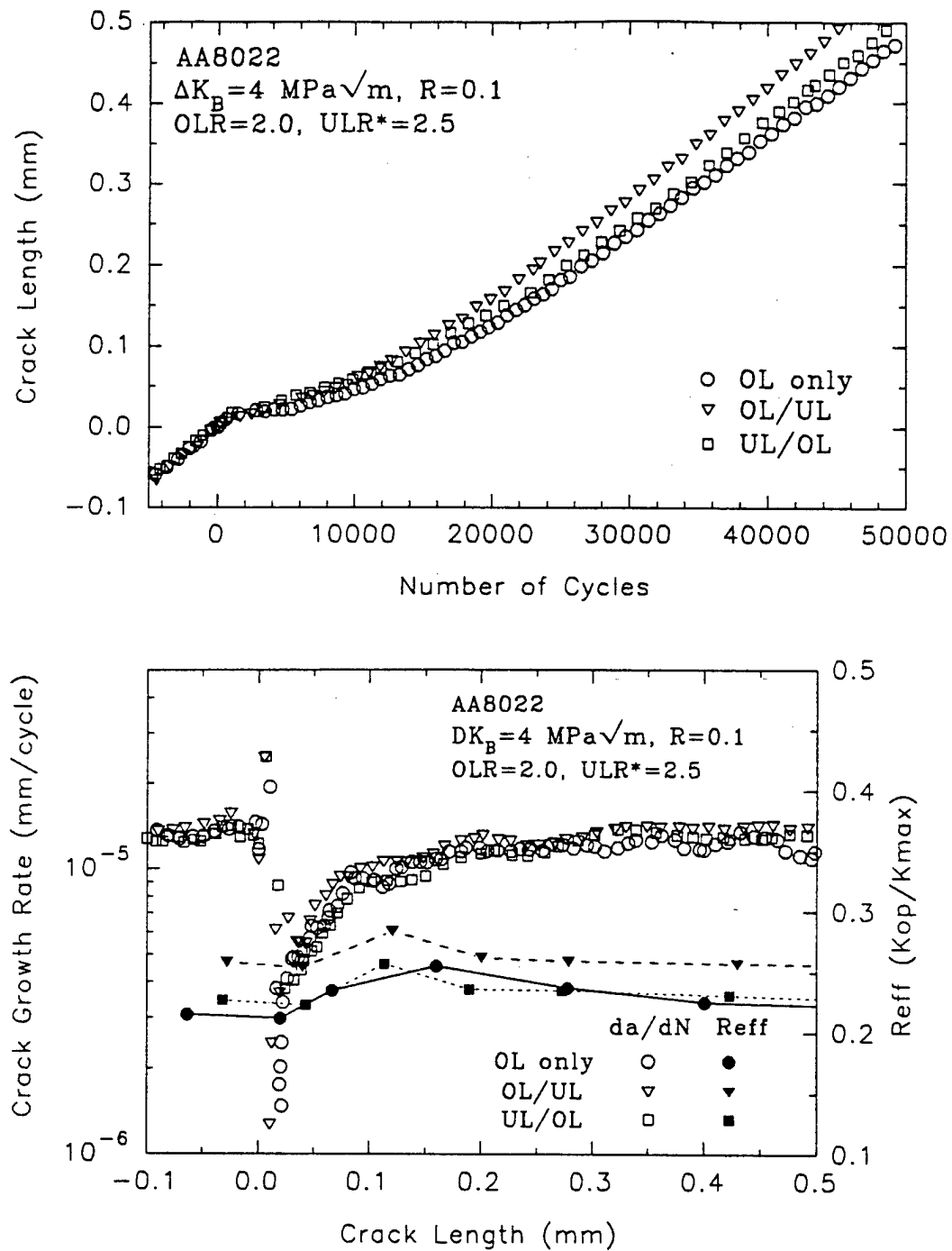
Figure 4.19. Effect of overload/underload combinations ( \text{OLR}=2/\text{ULR}^*=2.5 ) on the overload response of AA8022 at R=0.1 .
