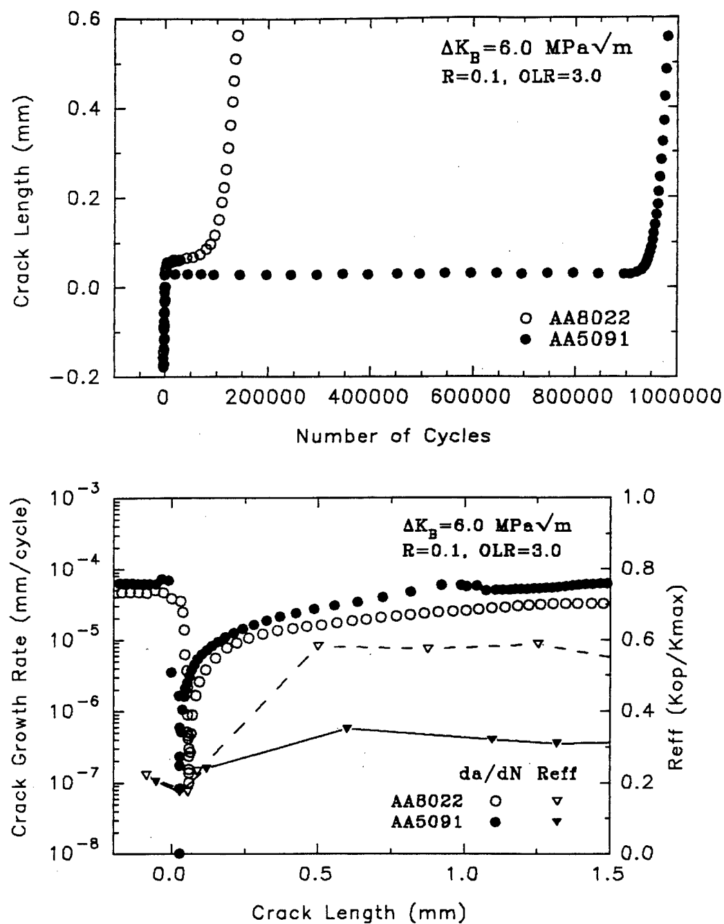
Figure 4.18. Comparison of overload response ( \text{OLR}=3 ) in AA8022 and AA5091 at R=0.1 , \Delta K_B=6.0 \text{ MPa}\sqrt{\text{m}} .
