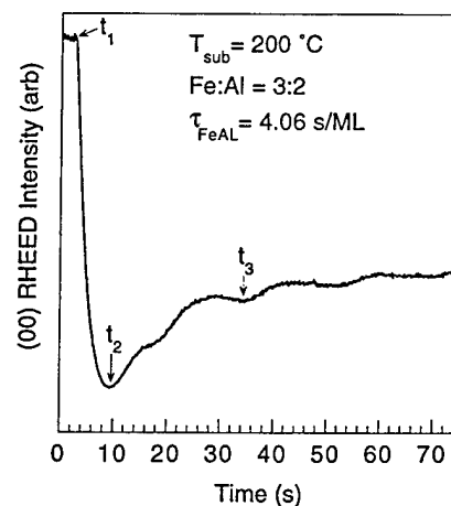
Fig. 2. RHEED intensity of the specular diffraction beam during initial nucleation of \text{Fe}_x\text{Al}_{1-x} on AlAs. The starting pattern at t_1 is an AlAs(3 × 2) pattern. Growth is started at t_1 . At time t_2 , the RHEED pattern is no longer visible. At time t_3 , the intensity recovers to 30% of the original intensity and exhibits a broad and diffused (1 × 1) pattern.
