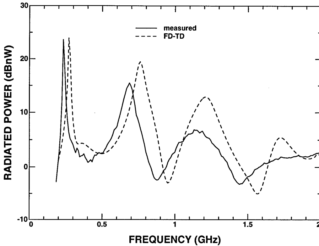
Figure 4.15: Radiated power from two 13.01 cm by 21.43 cm modules over a finite ground plane excited by a single 1 mV voltage source with zero impedance as a function of frequency.
