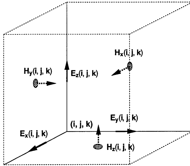
Figure 1.1: Field components in Yee's rectangular grid.
