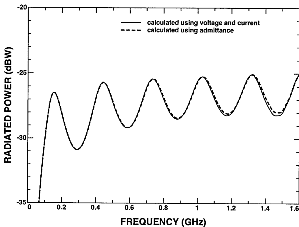
Figure 5.13: Radiated power of a coaxial line fed wire of length 0.5 m and radius 2 mm for the lumped element FD-TD with seven RLC circuits calculated using the admittance vs. calculated using the current and voltage.
