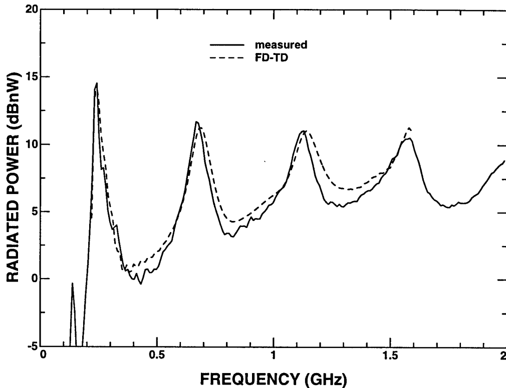
Figure 4.13: Radiated power from a 2.54 cm by 29.21 cm module over a finite ground plane excited by a 1 mV voltage source with zero impedance as a function of frequency.
