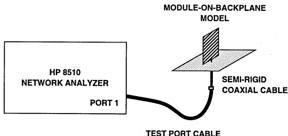
Figure 1.6: Measurement setup for modules-on-backplane configurations.
