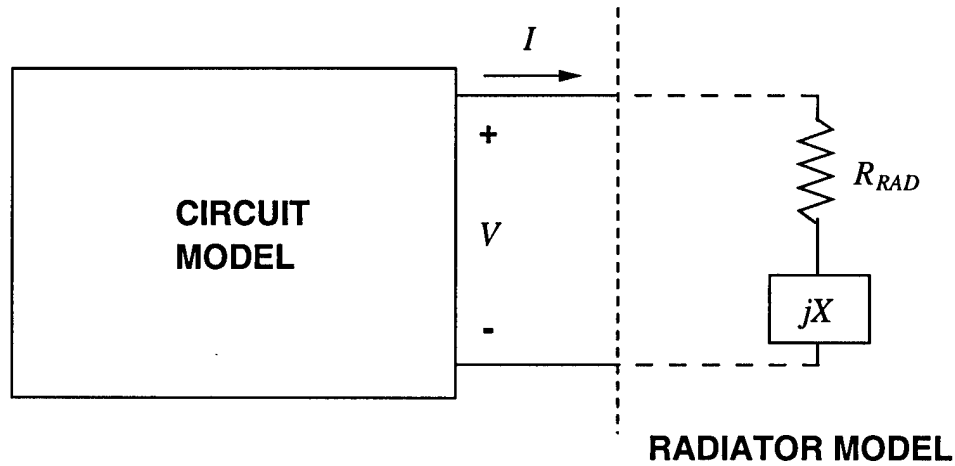
Figure 4.11: Characterization of radiative properties of modules-on-backplane as circuit parameters.
