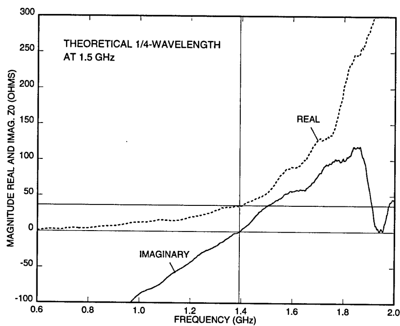
Figure 4.5: Radiation impedance of a 5 cm monopole over a ground plane of dimensions 30.48 cm by 31.75 cm as a function of frequency.
