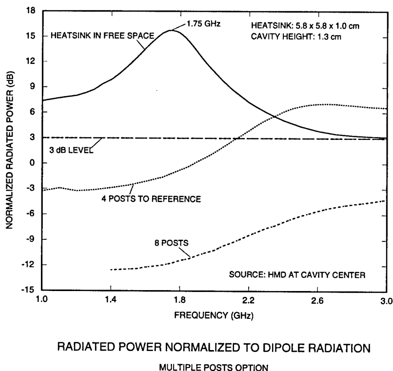
Figure 3.16: Comparison of normalized total radiated power with HMD source for heatsink B with 4 and 8 posts and without posts.
