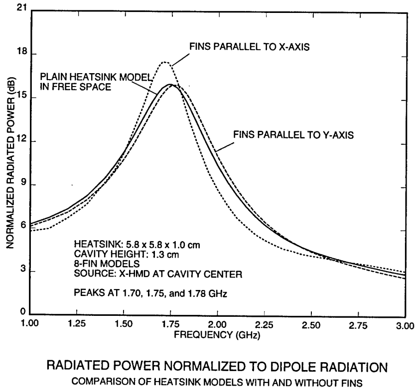
Figure 3.11: Comparison of normalized total radiated power with x -directed HMD source for plain and finned versions of heatsink B .
