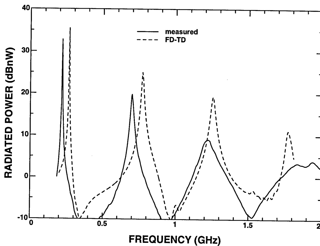
Figure 4.16: Radiated power from three 13.01 cm by 21.43 cm modules over a finite ground plane excited by a single 1 mV voltage source with zero impedance as a function of frequency.
