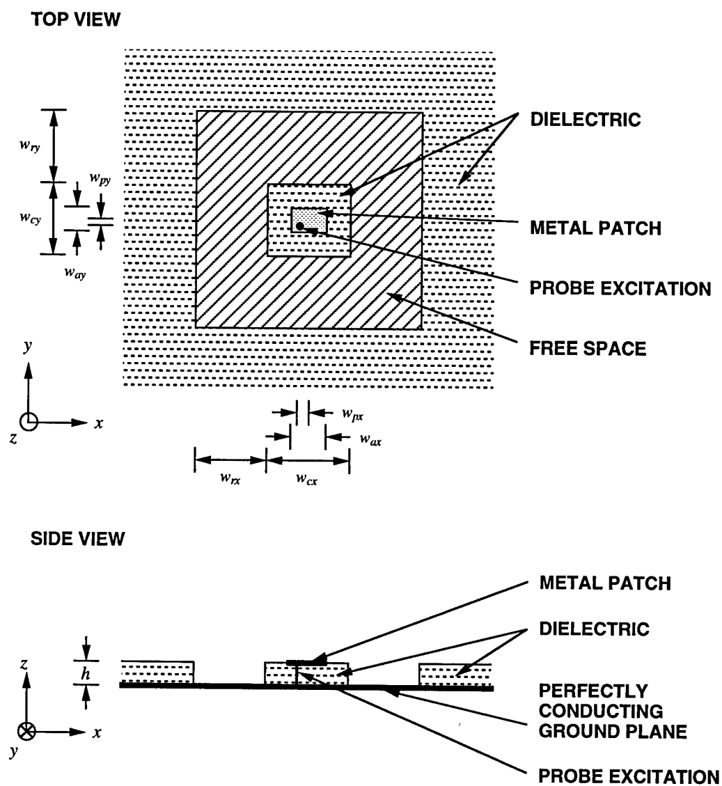
Figure 6.1: Microstrip patch antenna on a non-uniform dielectric substrate.
