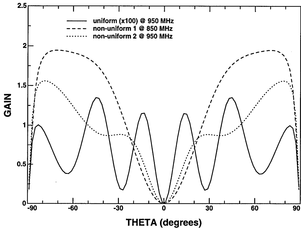
Figure 6.8: Gain pattern for a vertical dipole in a uniform and two non-uniform substrate configurations in the x - z plane for the vertical polarization.
