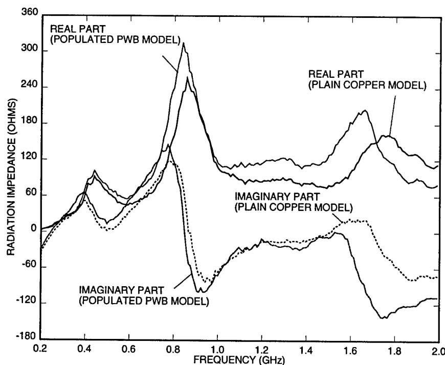
Figure 4.6: Radiation impedance of a populated and a plain copper module of dimension 13.01 cm by 21.43 cm over a finite ground plane as a function of frequency with the source connected to the bottom edge of the left side of the module.
