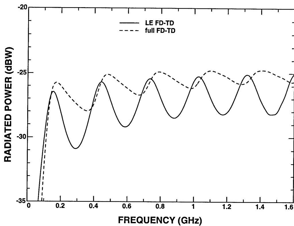
Figure 5.15: Radiated power of a coaxial line fed wire obtained using lumped element FD-TD with seven RLC circuits vs. full FD-TD.
