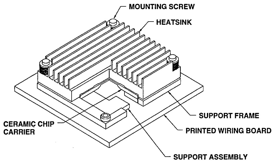
Figure 3.1: Cut away view of a VLSI package/heatsink configuration.
