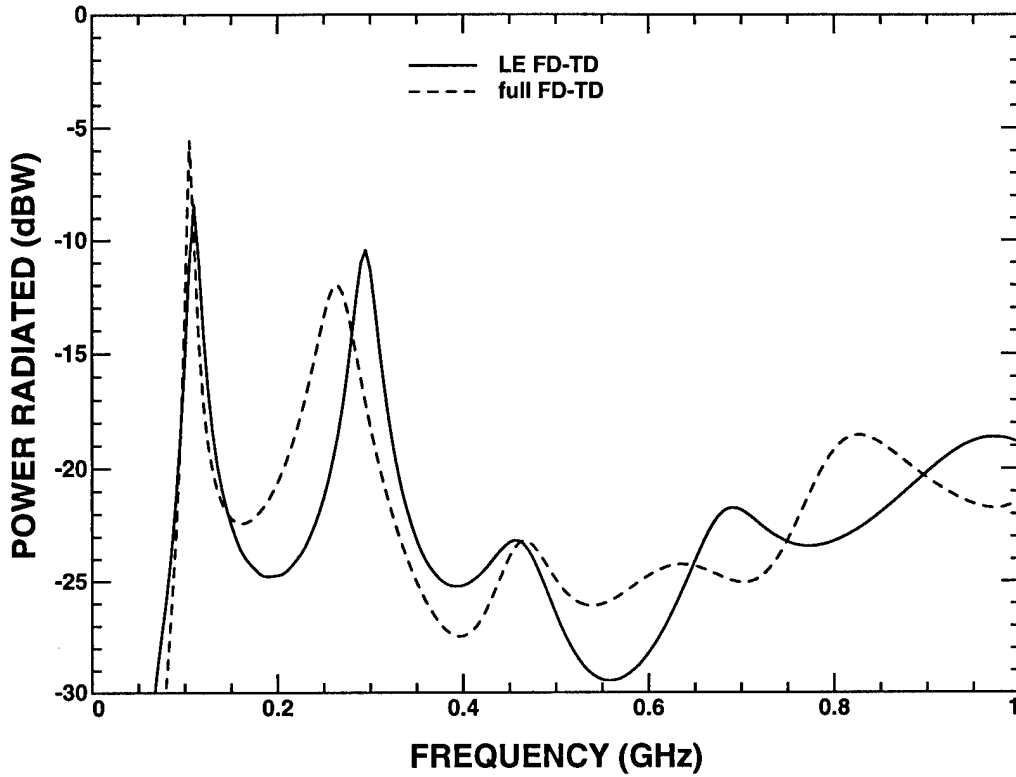
Figure 5.20: Radiated power using a lumped element FD-TD simulation with three RLC circuits and using a full FD-TD simulation of the infinite metal screen configuration B .
