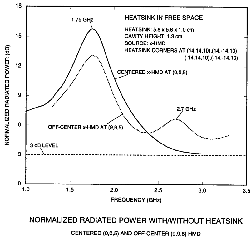
Figure 3.8: Comparison of normalized total radiated power in presence and absence of heatsink B with a centered and an off-center HMD source.
