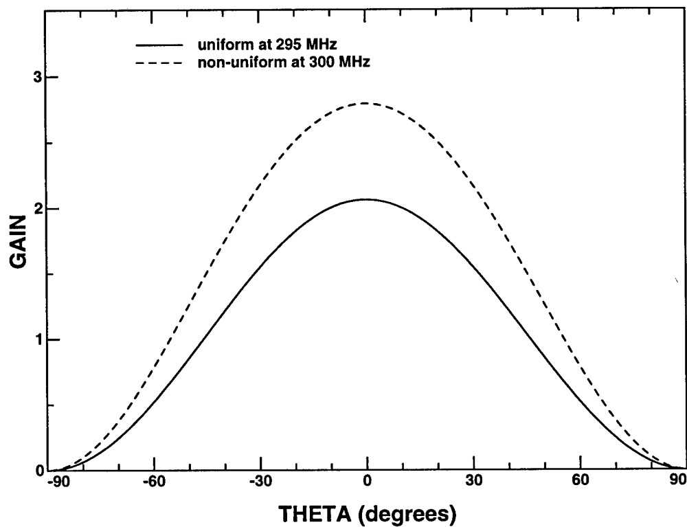
Figure 6.17: Radiation pattern of a microstrip patch antenna over a uniform and over a non-uniform substrate in the y - z plane for the horizontal polarization at the first resonance.
