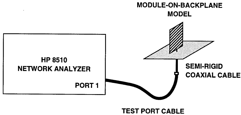
Figure 4.3: Measurement setup.
