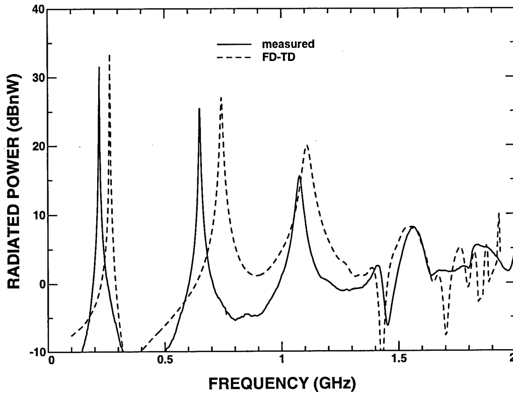
Figure 4.17: Radiated power from a partially enclosed 13.01 cm by 21.43 cm module over a finite ground plane excited by a 1 mV voltage source with zero impedance as a function of frequency.
