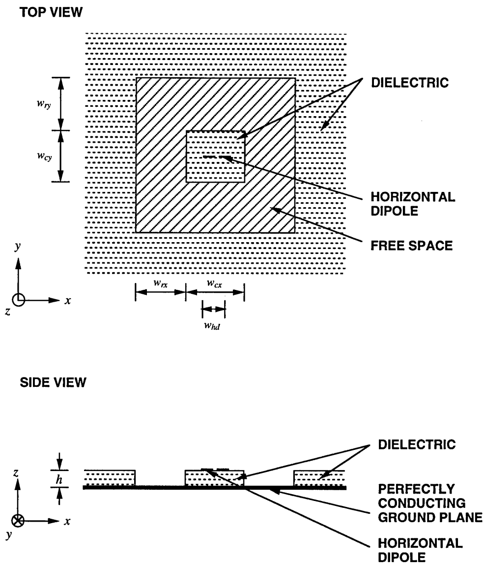
Figure 6.9: Horizontal dipole on a non-uniform dielectric substrate.
