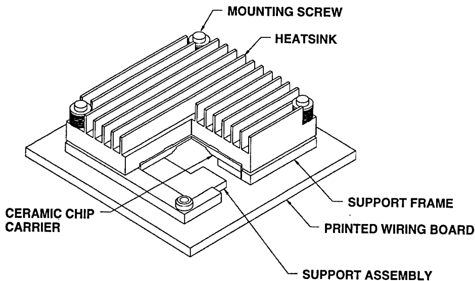
Figure 1.2: Cut away view of a VLSI package/heatsink configuration.
