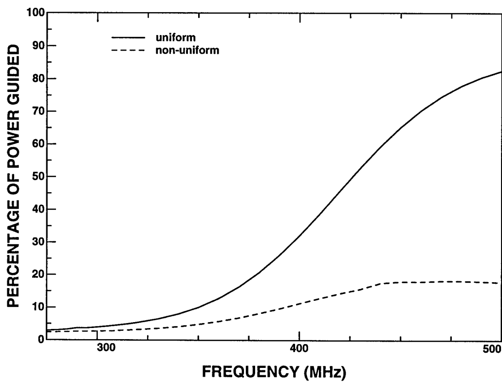
Figure 6.15: Guided power of a microstrip patch antenna over a uniform and over a non-uniform substrate.
