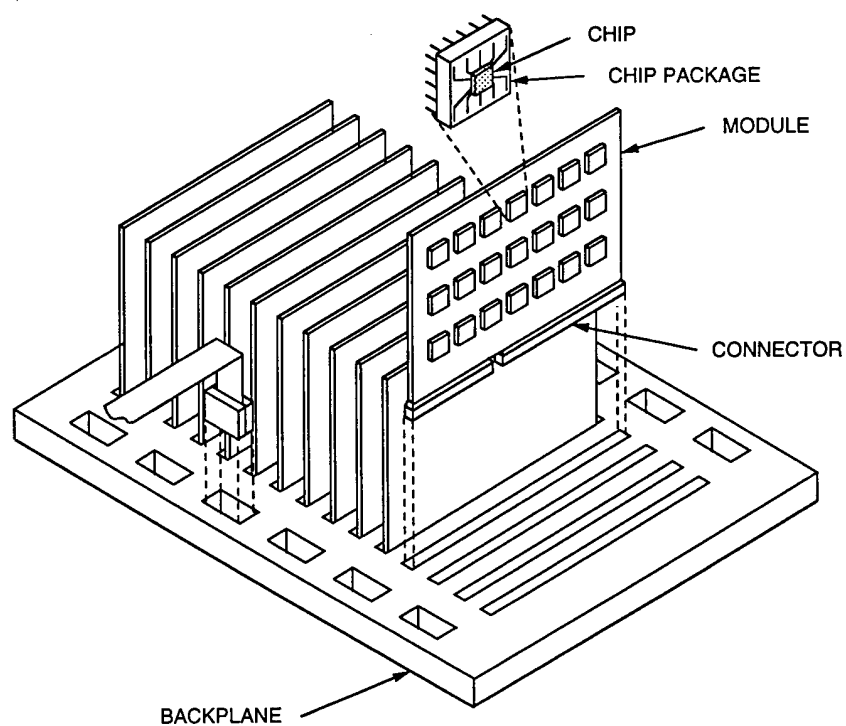
Figure 4.1: A typical modules-on-backplane configuration.
