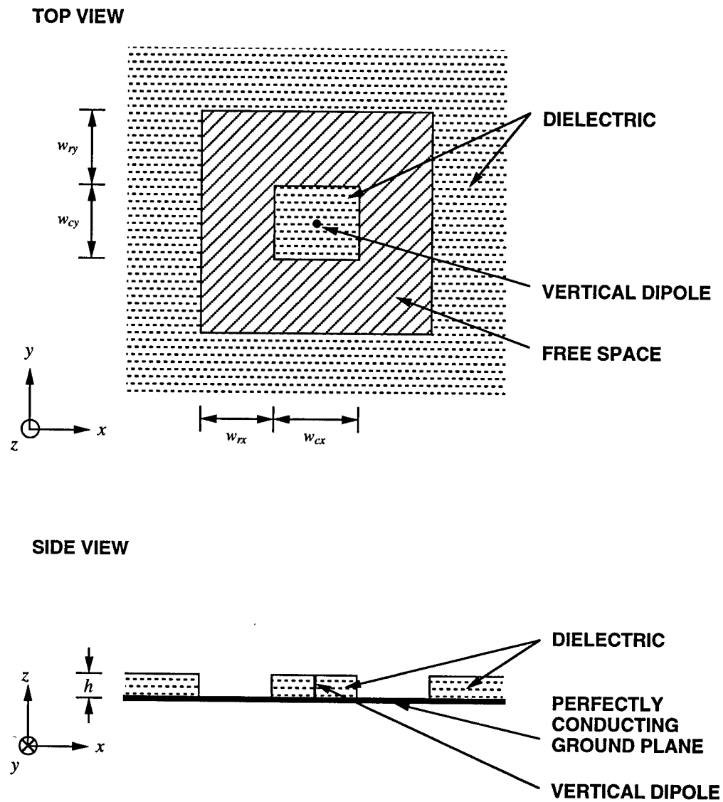
Figure 6.5: Vertical dipole in a non-uniform dielectric substrate.
