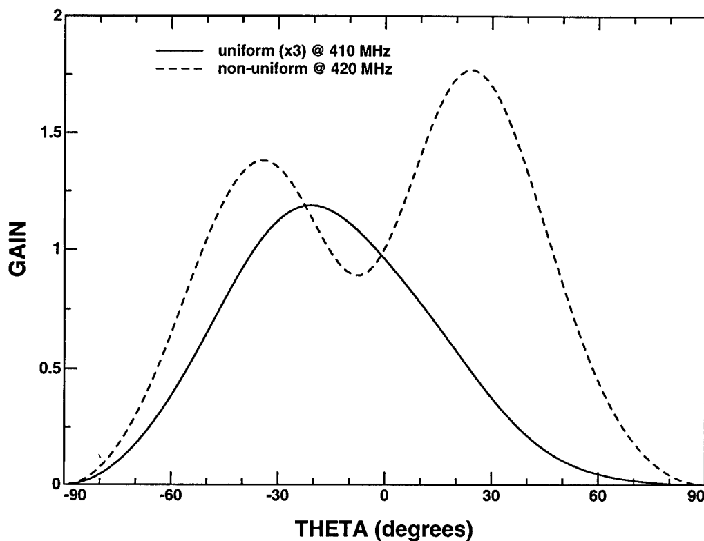
Figure 6.18: Radiation pattern of a microstrip patch antenna over a uniform and over a non-uniform substrate in the x - z plane for the vertical polarization at the second resonance.
