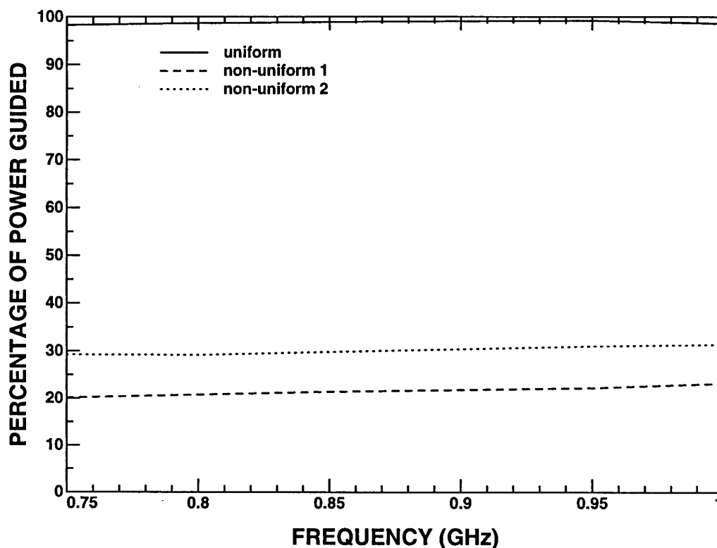
Figure 6.7: Guided power of a vertical dipole in a uniform and two non-uniform substrate configurations.
