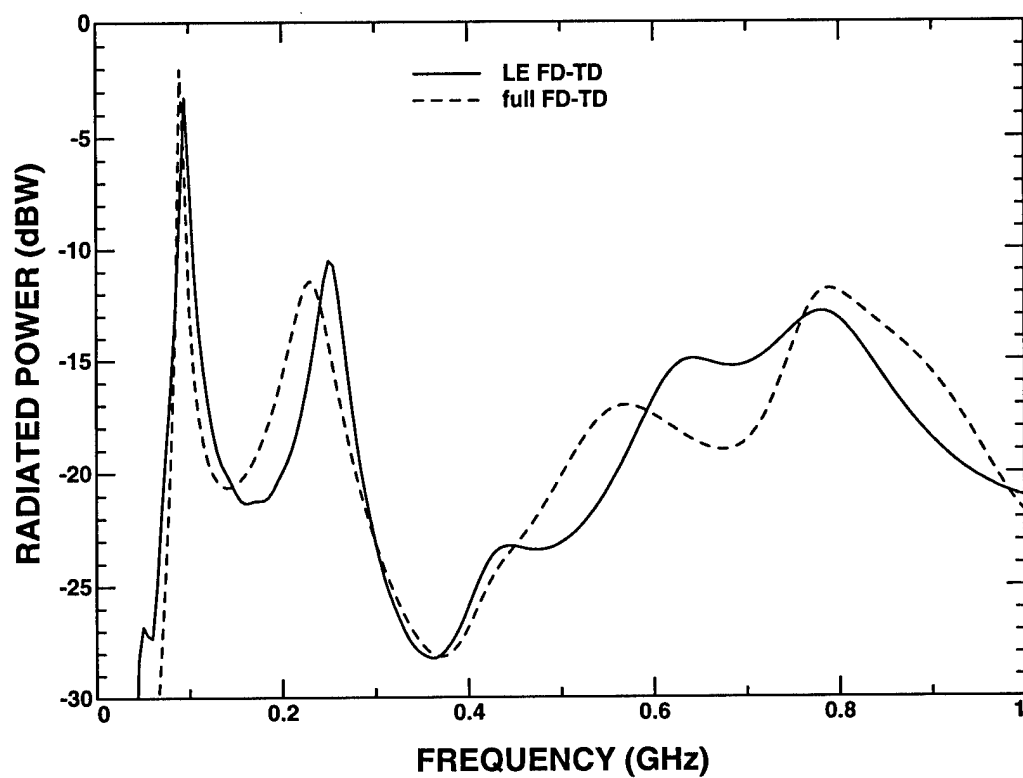
Figure 5.18: Radiated power using a lumped element FD-TD simulation with three RLC circuits and using a full FD-TD simulation of the infinite metal screen configuration A.
