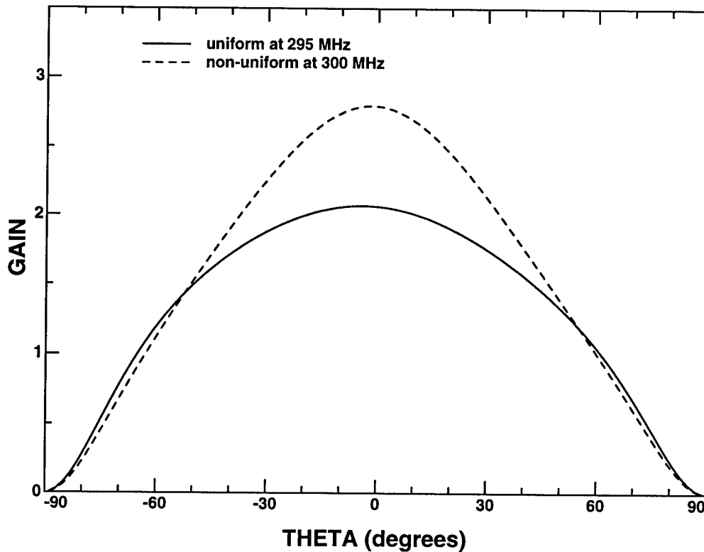
Figure 6.16: Radiation pattern of a microstrip patch antenna over a uniform and over a non-uniform substrate in the x - z plane for the vertical polarization at the first resonance.
