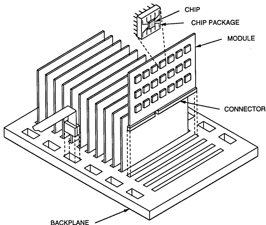
Figure 1.4: A typical modules-on-backplane configuration.
