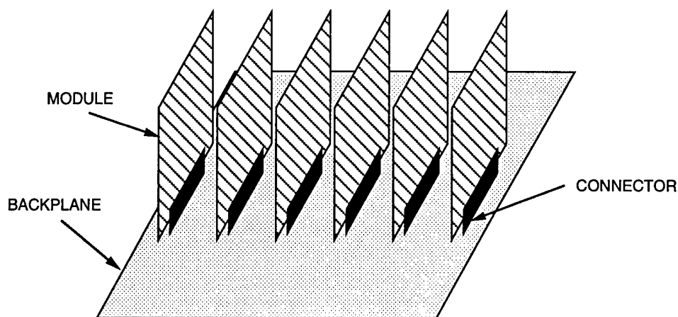
Figure 1.5: Simplified model of the modules-on-backplane configuration.
