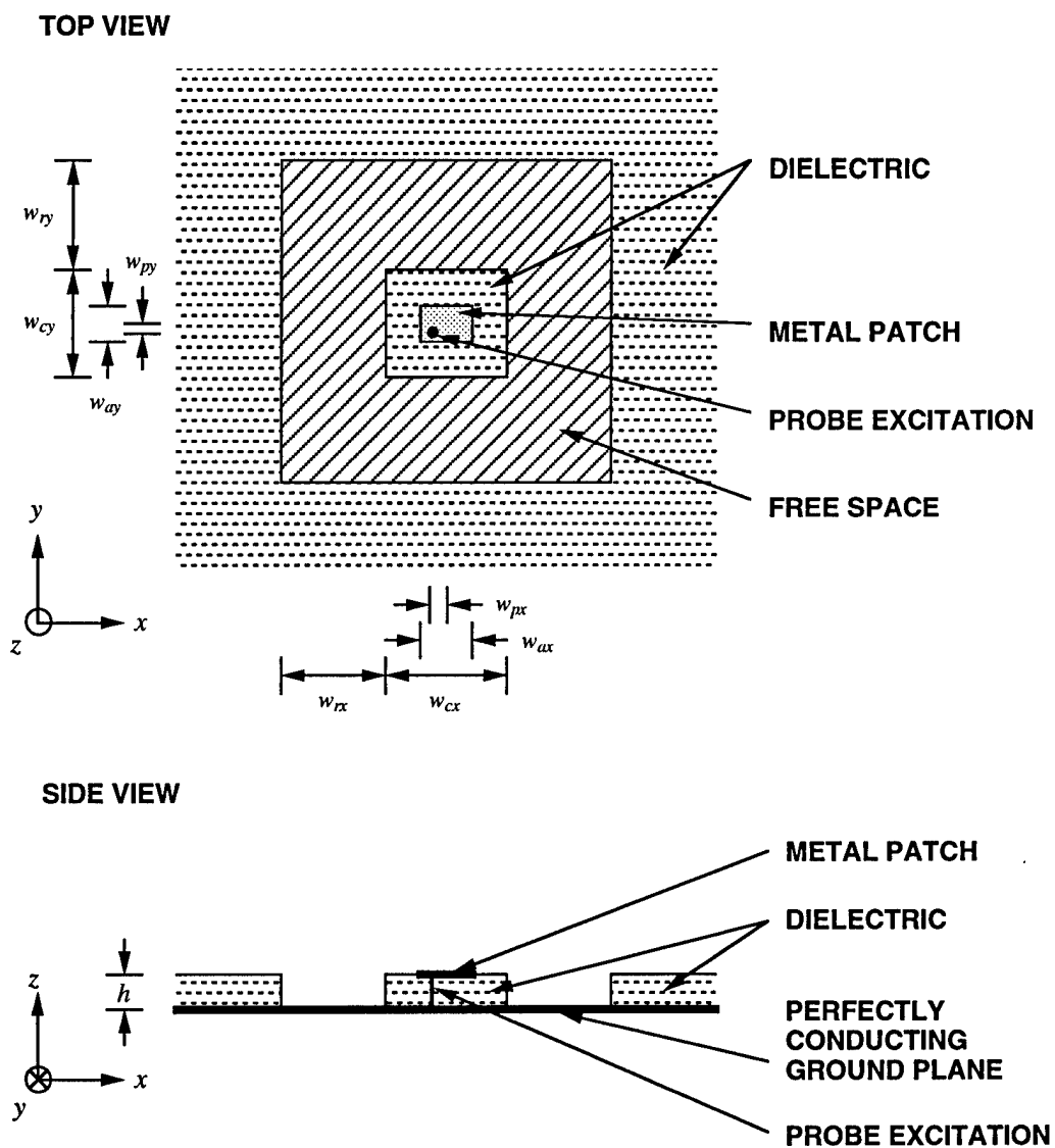
Figure 1.8: Microstrip patch antenna on a non-uniform dielectric substrate.
