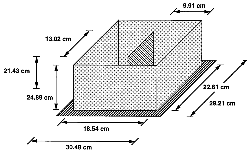
Figure 4.18: Partially enclosed module-on-backplane configuration.
