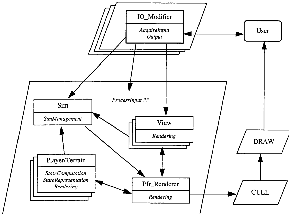
Figure 6 - ObjectSim architecture.
