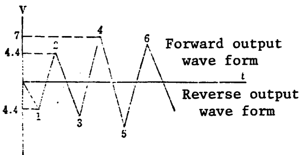
Figure 2. Traveling Wave Directional Detector Wave Form
