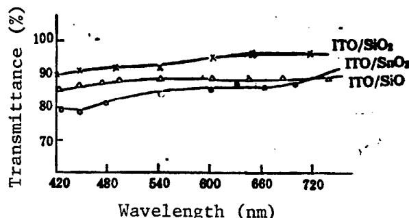
Figure 3. Transmittance of ITO/ \text{SiO}_x , ITO/ \text{SiO} and ITO/ \text{SnO}_2 Films
