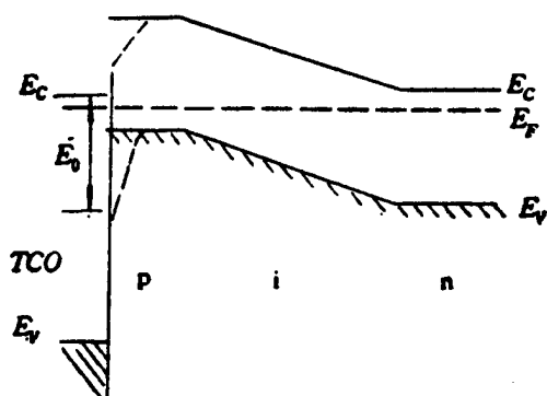
Figure 1. Barrier E_o at the Interface Between TCO and p^+Si:H
