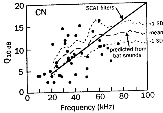
Fig. 11. Sharpness of frequency tuning ( Q_{10\text{dB}} ) in the cochlear nucleus of Eptesicus . (Data-points are from Haplea, Covey, and Casseday 1994; dashed lines are predicted tuning values--mean \pm 1 SD--from Menne 1988; solid sloping line is tuning of SCAT filters measured from frequency-response curves--Saillant et al. 1993.)
