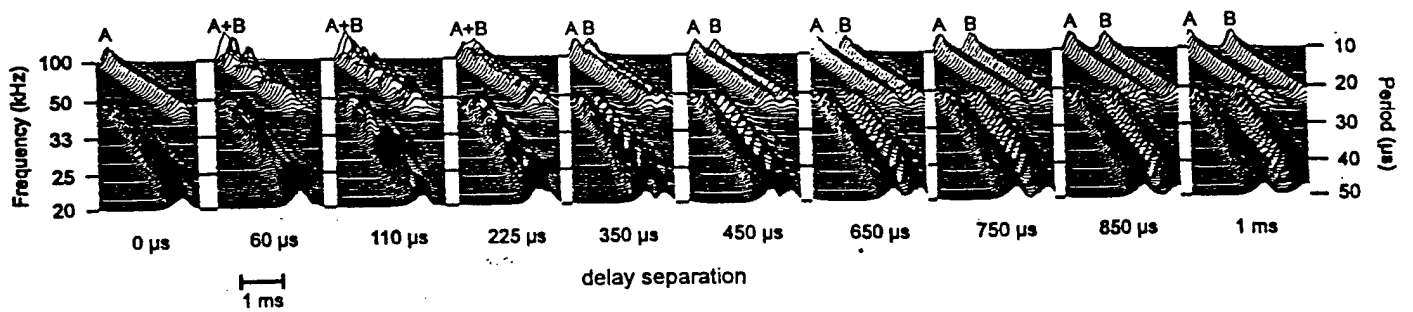
Fig. 6. SCAT (hyperbolic-frequency) spectrograms of pairs of overlapping echoes (A,B from Fig. 5) at different delay separations in relation to their integration-time of 300-400 μs. They appear as separate spectrograms for separations larger than the integration-time, and merge into the same spectrogram for separations that are smaller.
