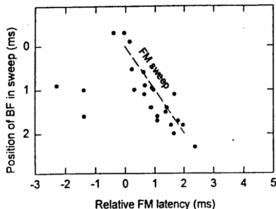
Fig. 22. Relative latencies of on-responses in inferior colliculus neurons tuned to different frequencies reconstruct the location of that tuned frequency along FM sweeps. Latencies of on-responses to tone-bursts at each cell's tuned frequency are subtracted from FM latencies and then corrected for the periodic spacing of responses to tone-bursts relative to FM sweeps. The spectrogram of the sweep is concealed within the dispersed absolute latencies of the responses (Fig. 18). (see also Bodenhamer and Pollak 1981.)
