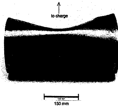
Figure 19. Final state of the scaled 'submarine' cylinder. Axis of the cylinder was perpendicular to the radial direction of the shock wave.
