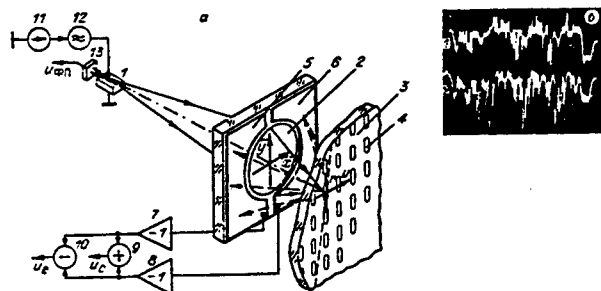
Figure 16. Layout of the Read Head With Diffraction Focusing Lens and Annular Photoreceiver (a) and Oscillograms of the Voltage at the Outputs of the Summer and Subtractor (b)
