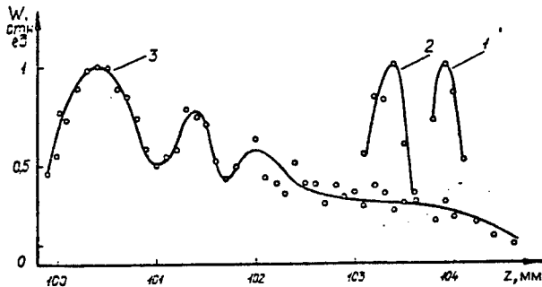
Figure 2. Experimental Curves of the Distribution of the Energy Density W (in Relative Units) Along the Axis of the Focal Segment: 1 - for an objective lens with focal distance z_0=105 mm, 2 - for an aberrant lens ( z_0=105 mm), 3 - for a generalized zone plate ( z_0=100 mm).
