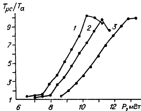
Figure 6. Writing Contrast T_{pc}/T_a as Function of Laser Beam Power (in mW) at Scanning Rates of 49 (1), 82 (2), and 140 cm/s (3).
