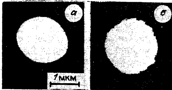
Figure 10. Scatter Circles of a Diffraction Lens (a) and the Series Produced Lens of the Sony KSS-123 Head (b)
