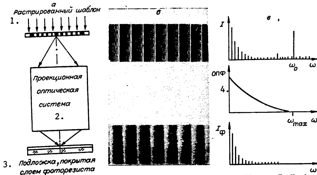
Figure 8. Photoscreening Method of Production of Surface Microrelief of Kinoform Elements. Realization of the Proposed Technique by Means of a Projection Photolithography Device (a); Fragment of the Scanned Photomask ( t_p=6 , l_{min}=1.2 \mu m ) and Distribution of Intensity Reconstructed in Plane of the Photoresist (b); Spectrum of Space Frequencies of Mask ( t=10 , t_p=0.6 \mu m ) and Result of Filtration of Step-and-Repeat Camera by Optical System (c).
