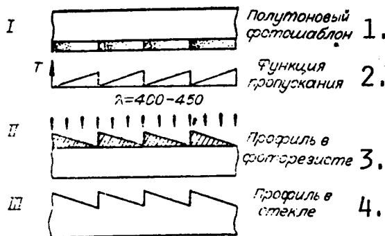
Figure 4. Phase Profile Production Technology Using a Half-Tone Photomask: I - Preparation of Photomask; II - Exposure and Development of Photoresist; III - "Dry" Etching of Glass.
