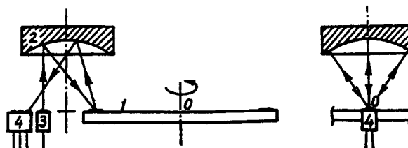
Figure 17. Optical Diagram of an Angle-Code Converter
