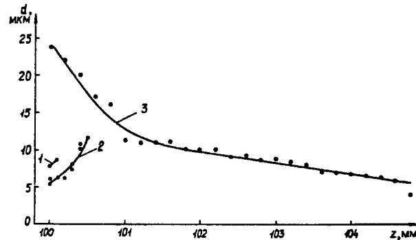
Figure 1. Experimental Relationship for the Change in Diameter d ( \mu\text{m} ) of the Focal Spot Along the Caustic: 1 - for a lens with focal distance z_0=105 mm, 2 - for an aberrant lens ( z_0=105 mm), 3 - for a generalized zone plate ( z_0=100 mm).
