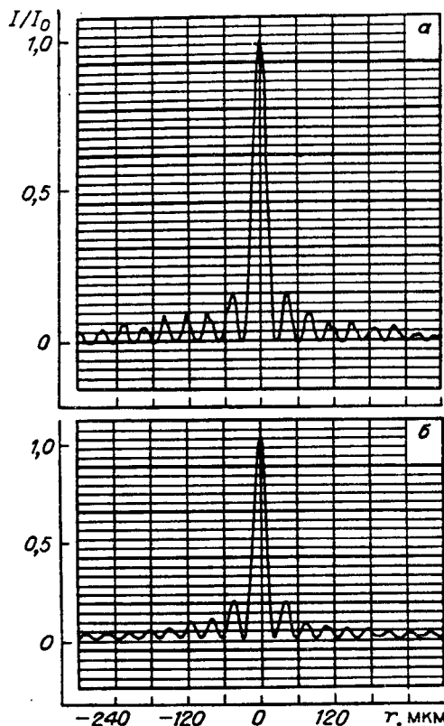
Figure 6. Distribution of Intensity in the Cross Section of the Luminous Line Formed by Lensacons With Parameters: a - f=300 mm, \alpha=10^{-2} , 2R=100 mm, \lambda=0.63 \mu\text{m} ; b - f=200 mm, \alpha=10^{-2} , 2R=40 mm, \lambda=0.67 \mu\text{m} .
