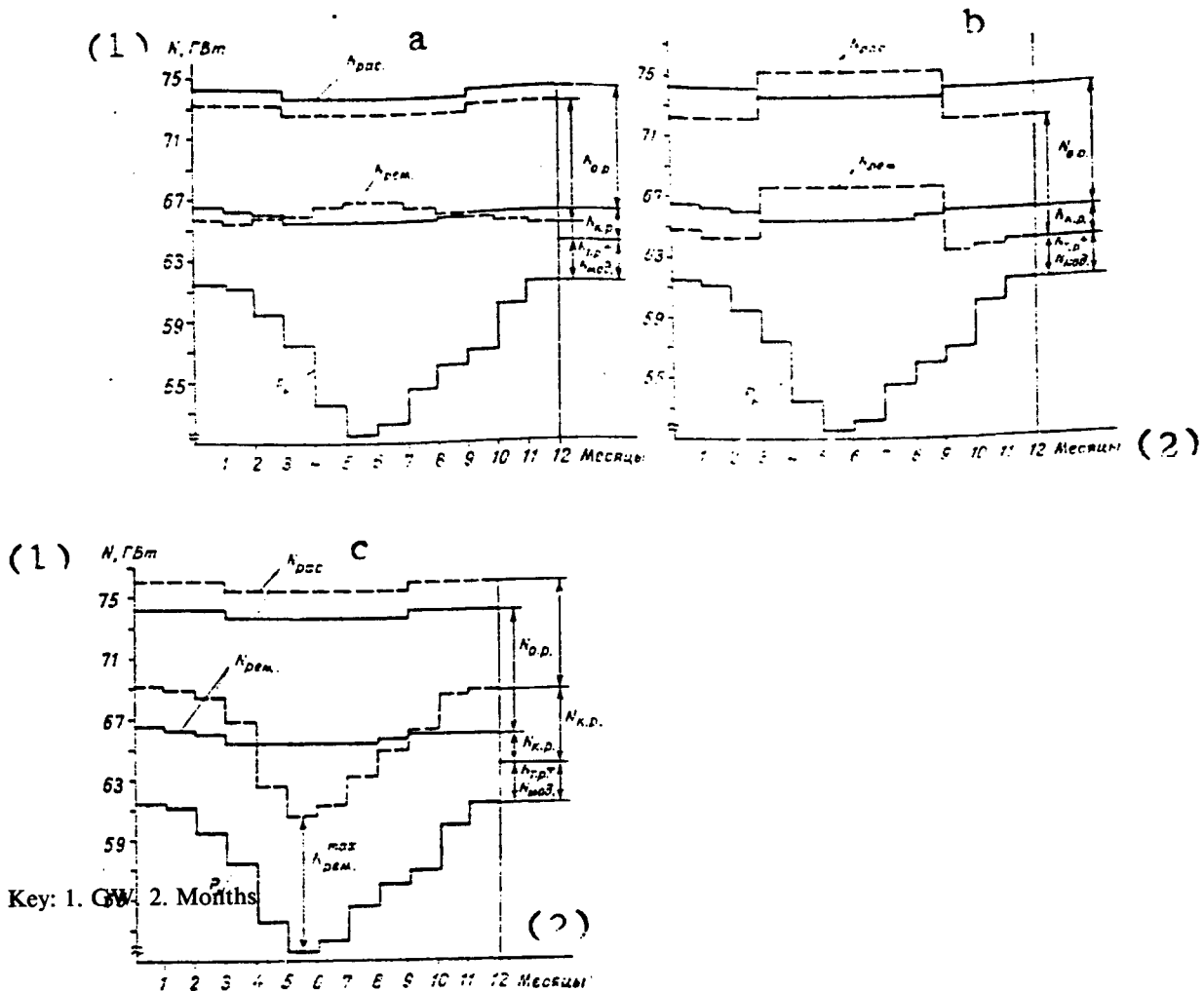
Figure 1. Alternatives of Optimal Repair Areas: a - in an Isolated System; b - Systems Helping Each Other; c - Limit Placed on Maximum Repair Levels; P_H - Monthly Maximum Chart; N_{o.p.} - Operating Reserve; N_{k.p.} - Reserve for Major and Intermediate Repairs; N_{t.p.} + N_{mod.} - Reserve for Current Repairs and Modernization
