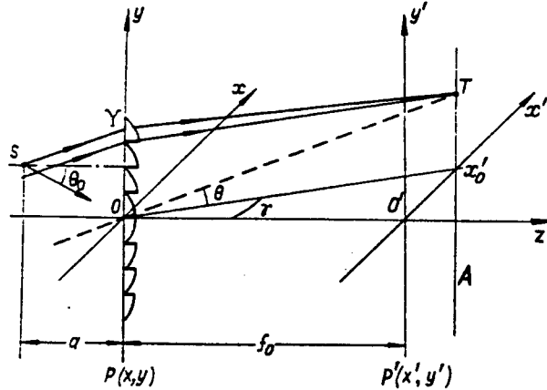
Figure 7. Geometry of Arrangement of an f\theta -Zone Plate and the Scanning Line
