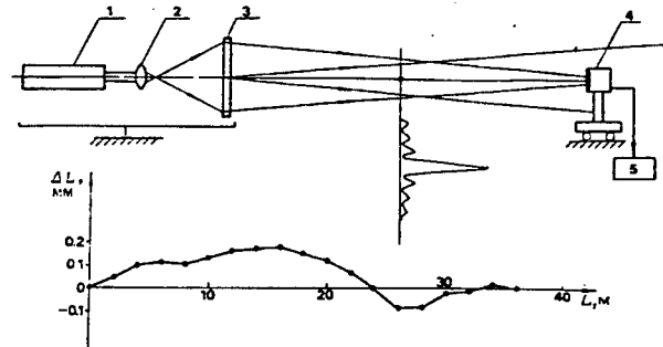
Figure 15. Optical Schematic of the Laser Slide Wire
