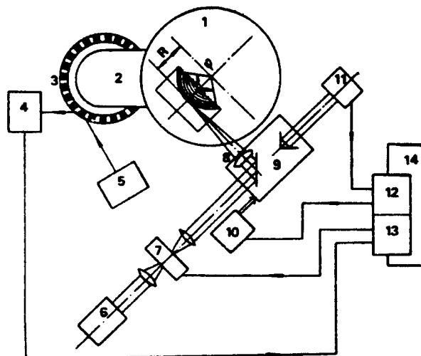
Figure 1. Block Diagram of the Laser Photoplotter
