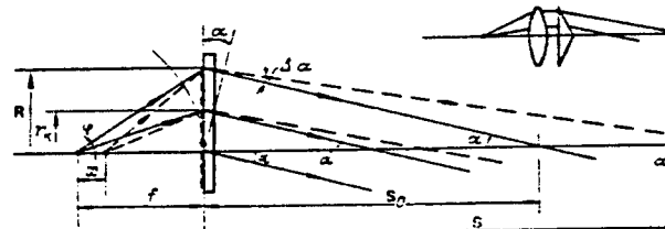
Figure 5. Transformation of a Spherical Into a Conical Wave With Constant Angle of Inclination of the Beams to the Axis \alpha by the Lensacon
