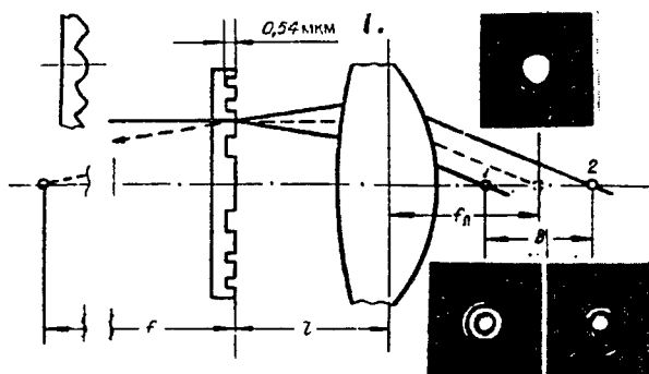
Figure 13. Optical Layout of a Bifocus System in the Return Path of the Rays
