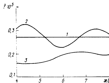
Figure 1. Dependence of Radiative Forces on Parameter x l at \kappa a = 1.0
