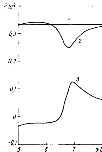
Figure 2. Dependence of Radiative Forces on Parameter \alpha l at \alpha a = 2.0
