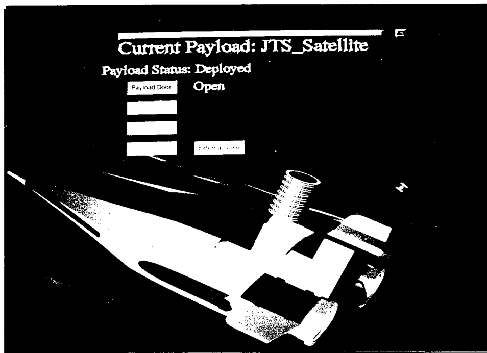
Figure 41: Mission Panel
