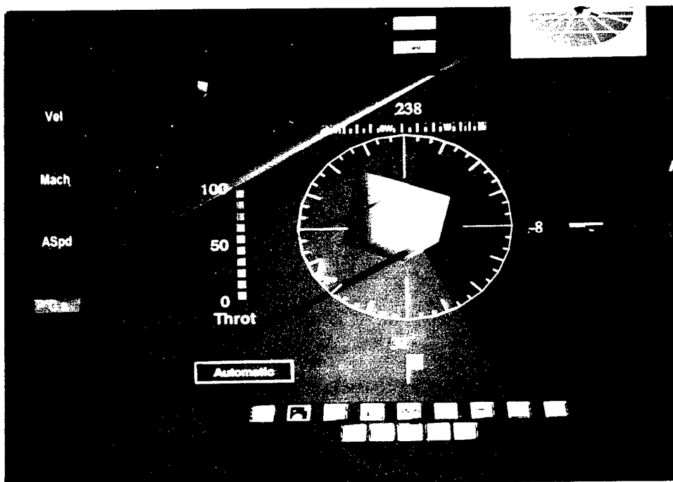
Figure 24: Waypoints
