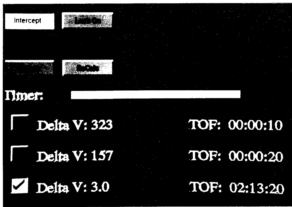
Figure 45: Time Slider
