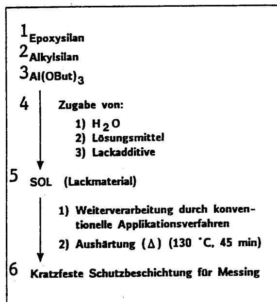
Figure 1: Flow Chart for the Production of a Mechanically Stable Protective Coating for Brass Surfaces
