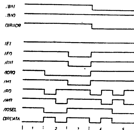
Figure 3: Most Important Bus Control States (1 inactive, 2 normal I-O operation or DMA access from the outside, 3 INT Acknowledge, 4 DMA access to the inside, 5 DMA access to the outside)
