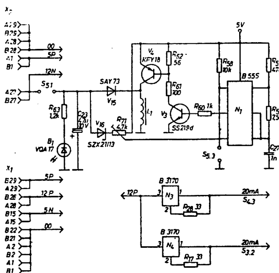
Figure 7: Transverter -12V
