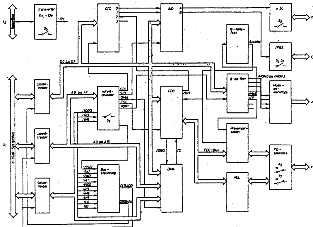
Figure 1: Wiring Diagram of the Floppy Disk Controller
