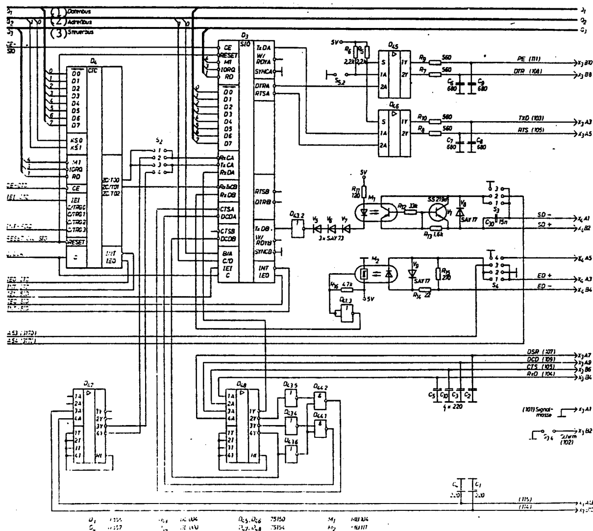
Figure 4: Serial Interfaces
