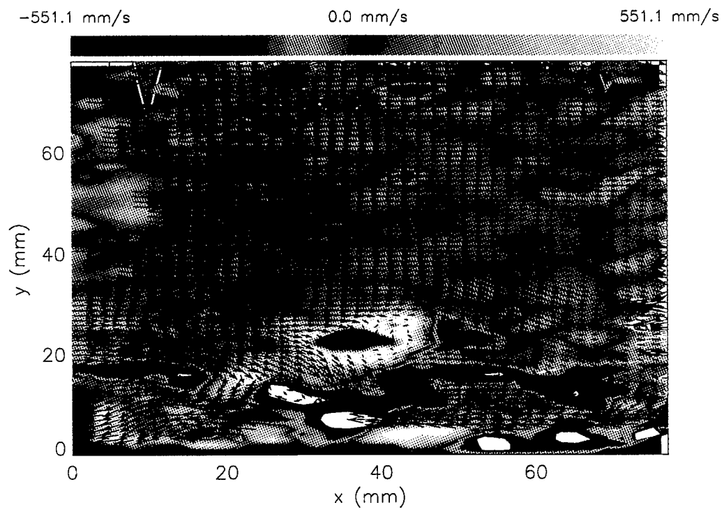
Figure 9 Instantaneous u, v, and w velocity fluctuations.
