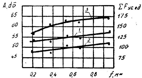
Figure 2. Amplitude of the Signal A_i (1, 2) and Area of the Acoustic Emission Spectra F (3) as a Function of the Wear Face f ; Frequency, kHz: 1, 35-70; 2, 70-100
