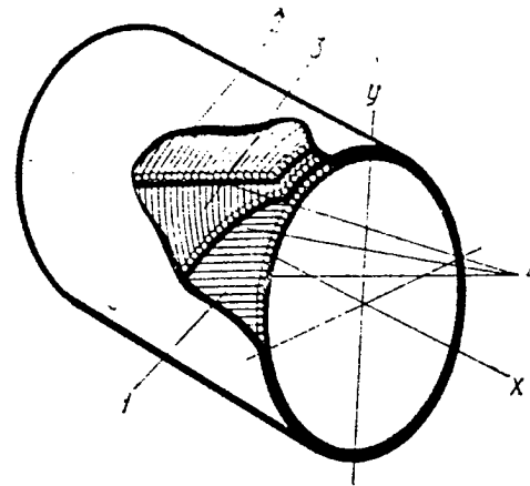
Figure 1. Block Diagram of the Arrangement of Fibers in a Composite Tube for a Gimbal Drive
