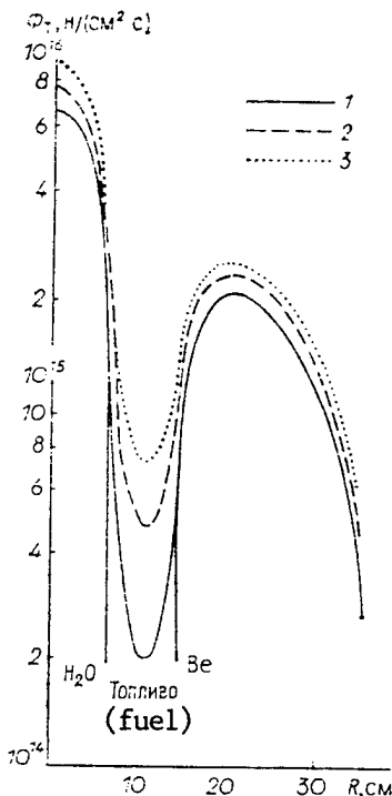
Figure 1. Radial Distribution of the Flux Density of Thermal Neutrons as a Function of the Load of Uranium 235: 1. 13.1 kg, K_{ef} = 1.16 ; 2. 6.5 kg, K_{ef} = 1.085 ; and 3. 4.5 kg, K_{ef} = 1.03 .
