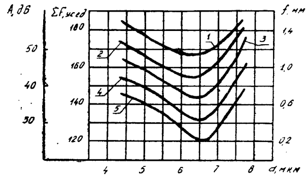
Figure 3. Amplitude of the Signal A_i (1, 2, 3) of the Area of the Spectra F (4) and Wear Face f (5) as a Function of the Thickness of the Coating d : Frequency, kHz: 1, 70-100; 2, 110-150; 3, 150-200. ( F is plotted in arbitrary units, and d is plotted in \mu\text{m} .)
