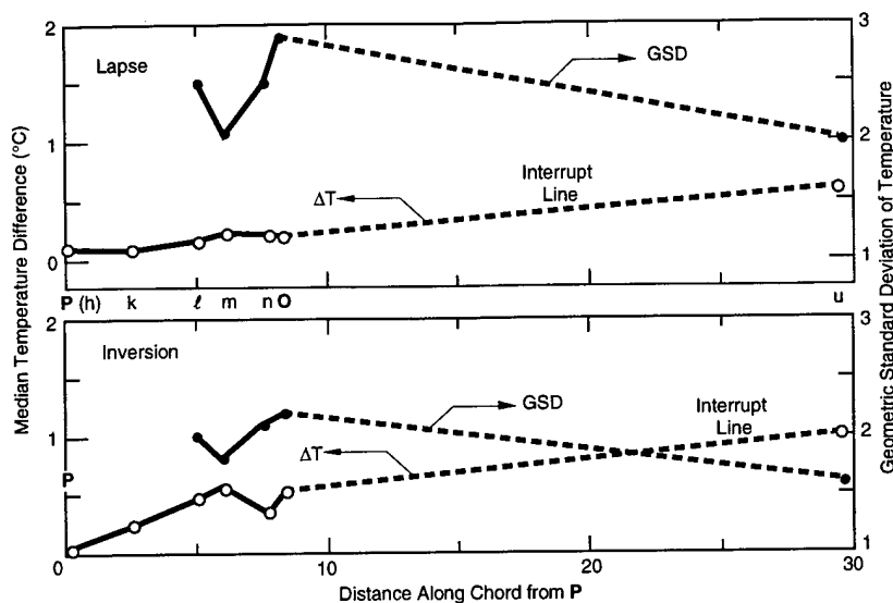
Figure 7. Median temperature difference and the geometric standard deviation of temperature difference measured along the river under lapse and inversion conditions. The letters coordinate the location of observing points with Figure 3.
