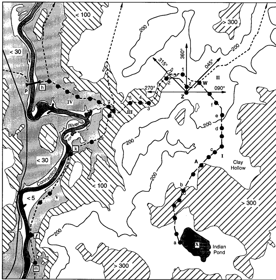
Figure 9. Enlarged map section showing topography (from USGS 7.5-minute quadrangle) of the area where large morning air temperature differences were observed. The symbols coordinate this figure with those in Parts I and III. The stippled layer lies 5 to 30 m above river level, the hatched layer 30 to 100 m above river level, and the alternate hatched layer 300 m above river level.
