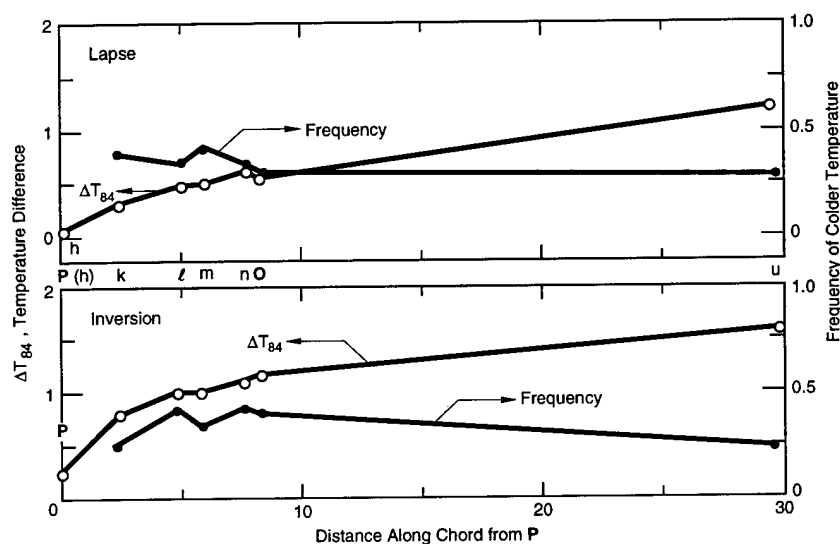
Figure 8. Eighty-fourth percentile of temperature difference, and the frequency of colder air temperature than at P, the reference point.
