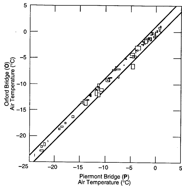
Figure 6. Temperature differences measured on two bridges 9 km apart along the Connecticut River. The plotted boxes enclose the range of temperatures observed on each bridge.
