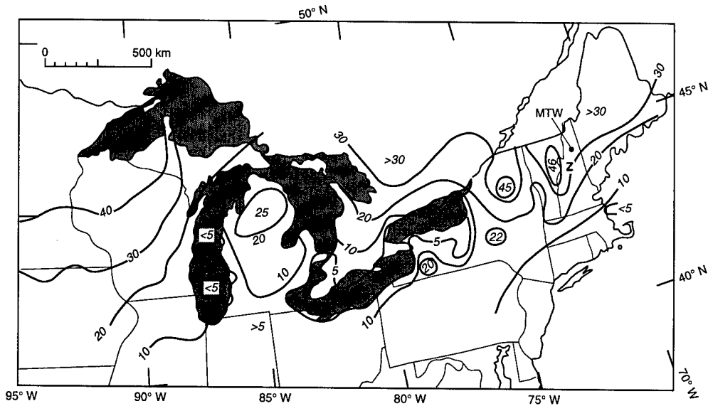
Figure 1. Mean annual number of subzero ( \leq -17.8^{\circ}\text{C} ) days occurring during the period 1951-80, from NOAA (1982). The Canadian data were provided by D. Phillips, AES, Downsview, Ontario. The study area of Figure 3 lies along the Connecticut River near Z.
