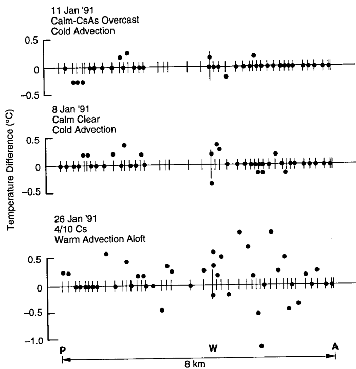
Figure 5. Magnitude of difference of repetitive air temperature measurements (solid circles), accompanying a direction reversal, over a 3- to 12-minute period. Observed differences of less than 0.1^{\circ}\text{C} are plotted along the zero axes.
