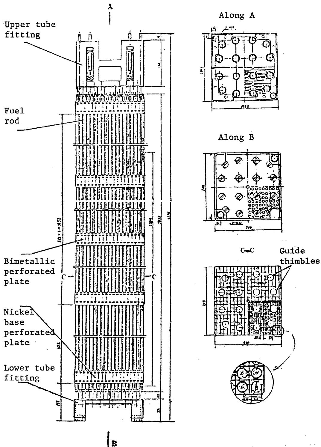
Figure 2. Fuel Assembly
