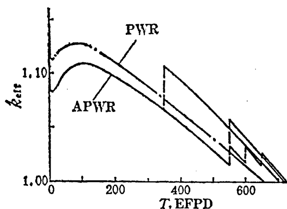
Figure 10. Effects of Pattern in Which Compressed-Water Rods Are Lifted on Fuel-Cycle Length
