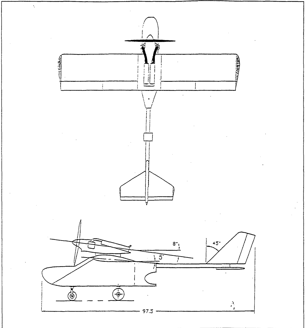
Figure 5 - FOG-R Drawings [After Ref. 14:p. 2]
