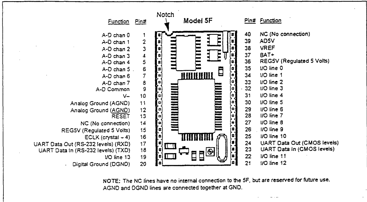
Figure 3 - Model 5F Pin Functions [After Ref. 12:p. 6-264]
