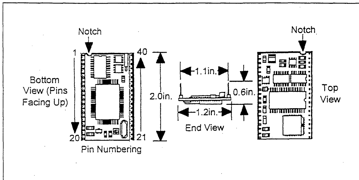
Figure 1 - Tattletale Model 5F [After Ref. 12:p. 6-263]
