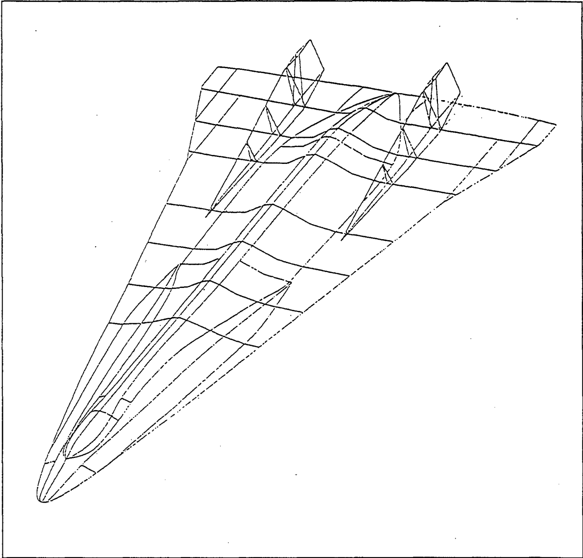
Figure 8 - LoFlyte Drawing [After Ref. 16]
