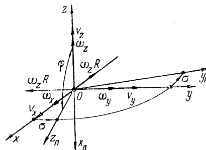
Figure 6.18. Coordinate System of AFA
