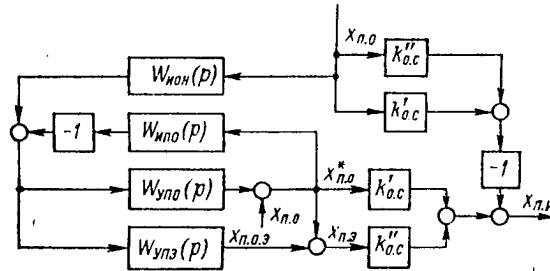
Figure 2.6. Block Diagram of Optical Device With Sensor of Parameters of Displacement of Observation Object
