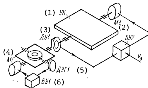
Figure 6.4. Layout of One-Axis Gyro-Stabilized Platform
