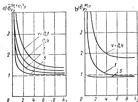
Figure 5.6. Dependence of Mean Square Estimates of Deviations of Coordinates of Two-Channel System: a--for master action; b--for perturbing action
