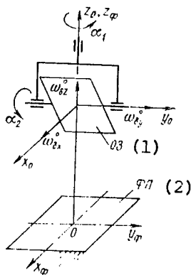
Figure 3.7. Stabilization Device With Flat Mirror (Rotational Axis of Mirror Is Fixed)
