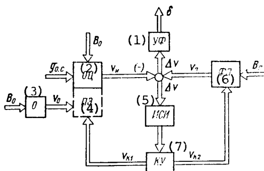
Figure 2.2. Generalized Functional Diagram of Optical Device With Image Misalignment Sensor
