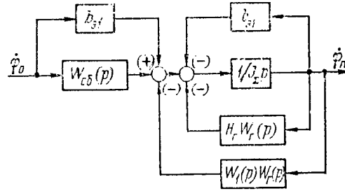
Figure 6.10. Transformed Block Diagram of One-Axis Gyro Stabilizer
