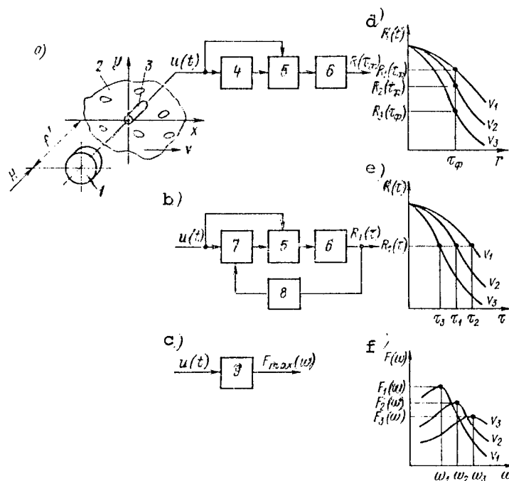
Figure 4.8. Autocorrelation SKSI: a--fixed delay; b--regulated delay; c--spectral analyzing; d, e, f--form of autocorrelation functions; 1--objective; 2--image; 3--photoelement; 4--constant delay module; 5-- multiplication module; 6--integrator; 7--regulated delay module; 8--regulator; 9--frequency spectrum analyzer
