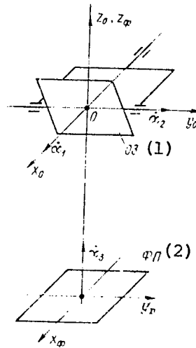
Figure 3.11. Stabilization Device With Flat Mirror in Gimbal Suspension (Axis y Coincides With Plane of Mirror)
