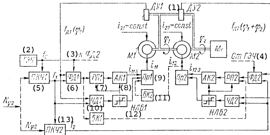
Figure 5.3. Functional Diagram of Two-Channel Electric Drive for Angular Displacements
