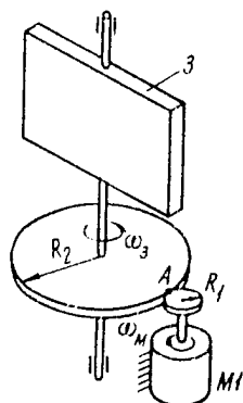
Figure 6.24. Scanner With Reducer Drive
