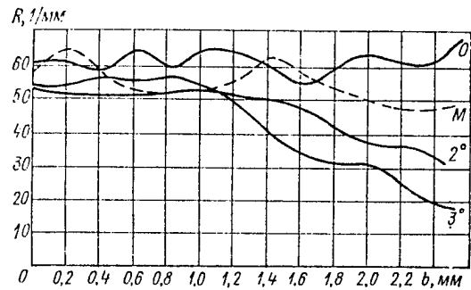
Figure 3.26. Measurement of Resolution of Tair-3 Objective Upon Decentering of Pair of Lenses
