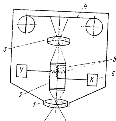
Figure 3.32. Layout of Device With Electronic Image Stabilization Systems:
