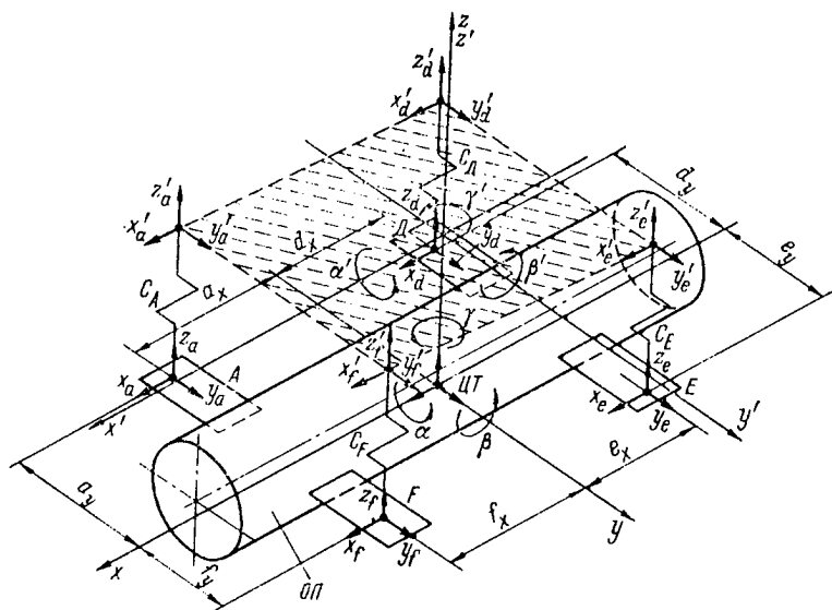
Figure 6.27. Layout of Cushioning System of Optical Device
