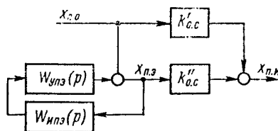
Figure 2.5. Block Diagram of Optical Device With Control Circuit of Position of Elements of Optical System
