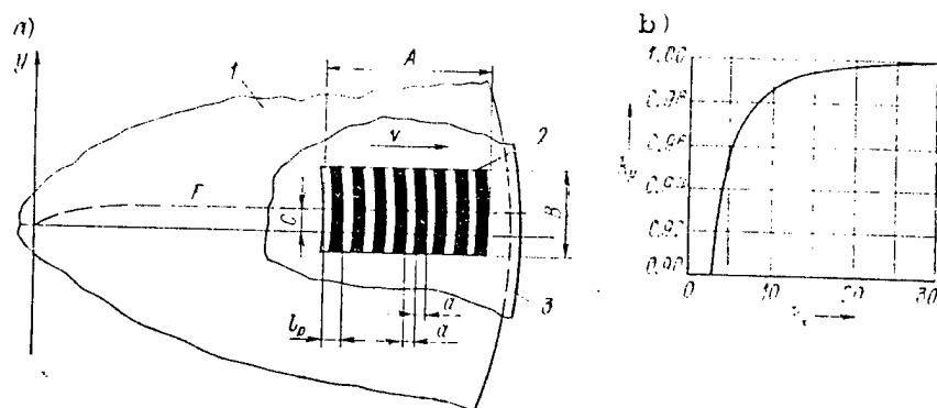
Figure 4.23. Working Segment of Modulator With Spiral Pattern: a--shape and arrangement of working segment; b--graph of function that determines position of line \Gamma ; 1--modulator disk; 2--working segment of pattern in diaphragm window; 3--fixed diaphragm
