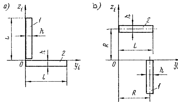
Figure 6.16. Variants of Arranging Mask Gates of Image Misalignment Sensor:
