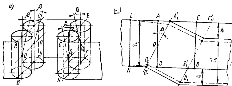
Figure 3.31. Diagram of Rotation of Guide Rollers (a) and Film Shifting Rollers (b)
