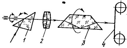
Figure 3.15. Layout of Camera With Image Stabilization: 1--rectangular prism; 2--objective; 3--Dove prism; 4--photographic film
