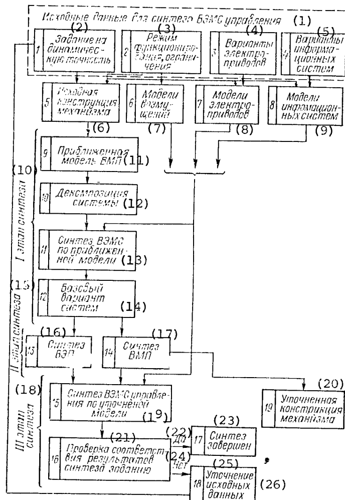
Figure 5.2. Diagram of Algorithm for Design of VEMP
