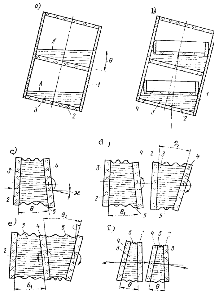
Figure 3.3. Layouts of Stabilization Devices With Liquid Optical Devices: a, b--liquid inertial wedges; c--single liquid wedge; d, e, f--pair of liquid wedges; 1--cylindrical vessel 2--planoparallel glass plate; 3--liquid; 4--movable planoparallel glass plate; 5--elastic corrugation
