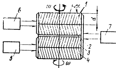
Figure 3.22. Layout of Stabilization Device With Planoparallel Fiber Optic Elements: 1, 2, 3, 4--planoparallel fiber optic element; 5--drive for mutual rotation of elements 3 and 4; 6--drive for mutual rotation of elements 1 and 2; 7--drive of stabilization system
