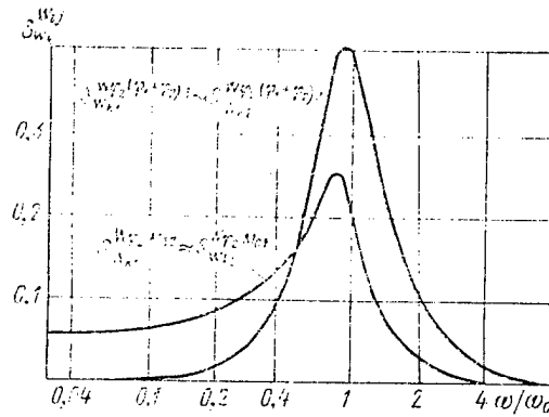
Figure 5.7. Function of Relative Sensitivity of System
