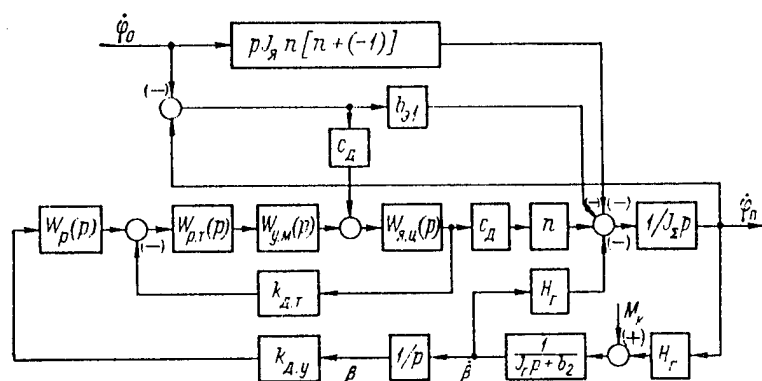
Figure 6.9. Block Diagram of One-Axis Gyro Stabilizer
