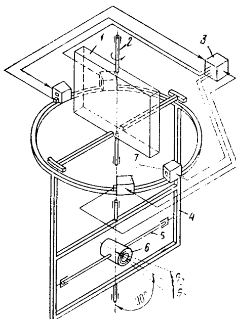
Figure 6.26. Scanner With Gyro Compensator of Reactive Moment on Base:
