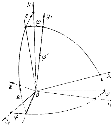
Figure 4.2. Coordinate Systems of Base and of Axes of Sensitivity of Laser Gyroscopes
