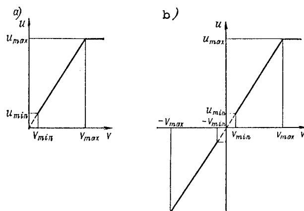
Figure 4.5. Static Characteristics of SKSI: a--nonreversible; b--reversible
