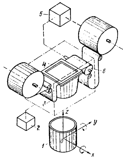
Figure 3.28. Layout of AFA in Which Objective With Spherical Field Is Used: 1--objective; 2, 5--drives; 3--photographic film; 4--leveling table; 6--measuring roller
