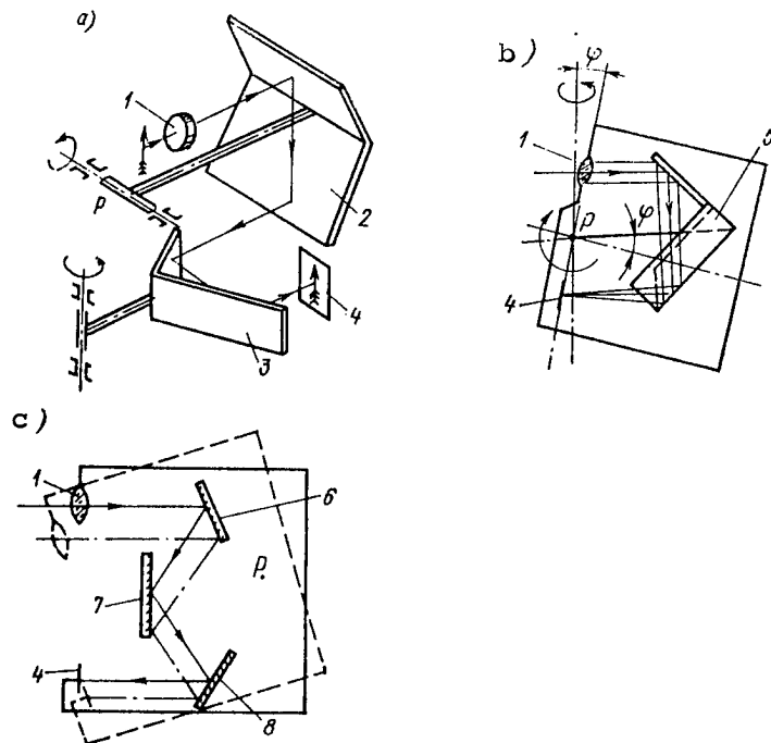
Figure 3.12. Diagrams of Stabilization Devices With Mirrors in Convergent Bundles of Beams: a--with two angular mirrors; b--with corner mirror; c--with three flat mirrors; 1--objective; 2, 3--angular reflectors; 4--detector; 5--corner mirror; 6, 7, 8--flat mirrors
