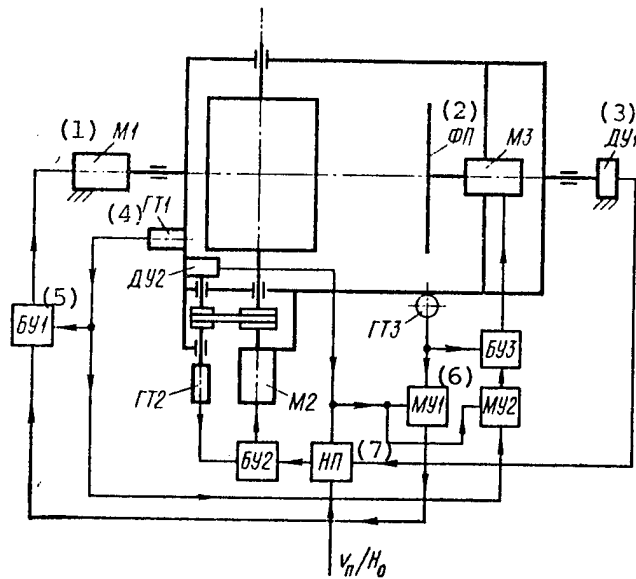
Figure 6.12. Functional Diagram of Image Stabilization System of AFA (Version I)
