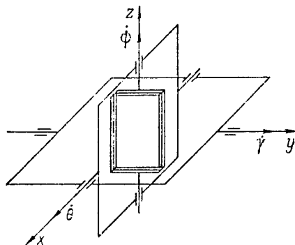
Figure 6.1. Layout of Three-Axis Gimbal Suspension of Stabilized Platform
