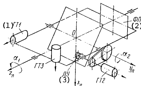
Figure 6.11. Kinematic Layout of AFA
