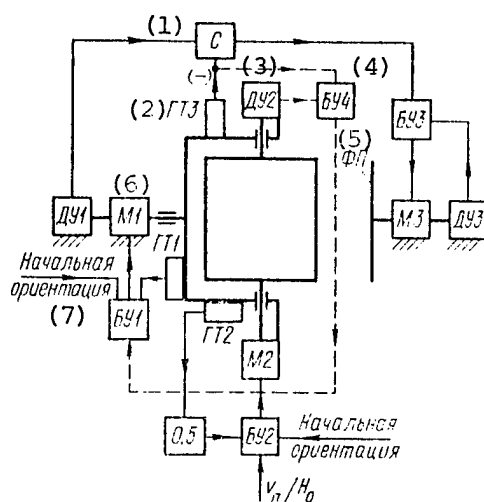
Figure 6.13. Functional Diagram of Image Stabilization System of AFA (Version II)
