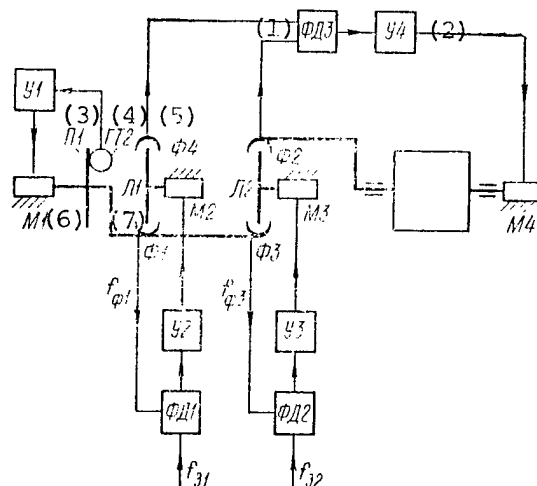
Figure 6.15. Functional Diagram of Inner Gimbal Axis Stabilization System
