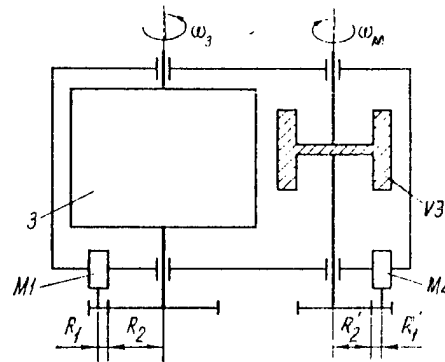
Figure 6.25. Scanner With Compensation of Reactive Moment on Base
