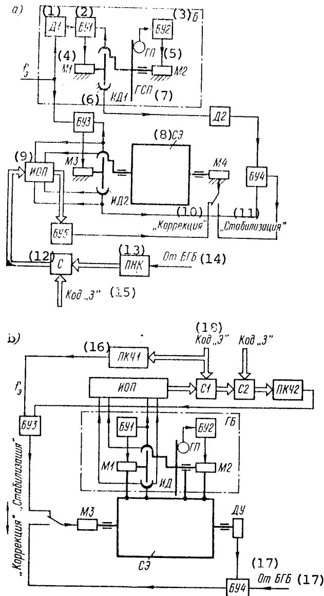
Figure 6.19. functional Diagrams of One-Coordinate Reorientation Systems: a--with arrangement of the gyro unit on base; b--with arrangement of gyro unit on element to be stabilized
