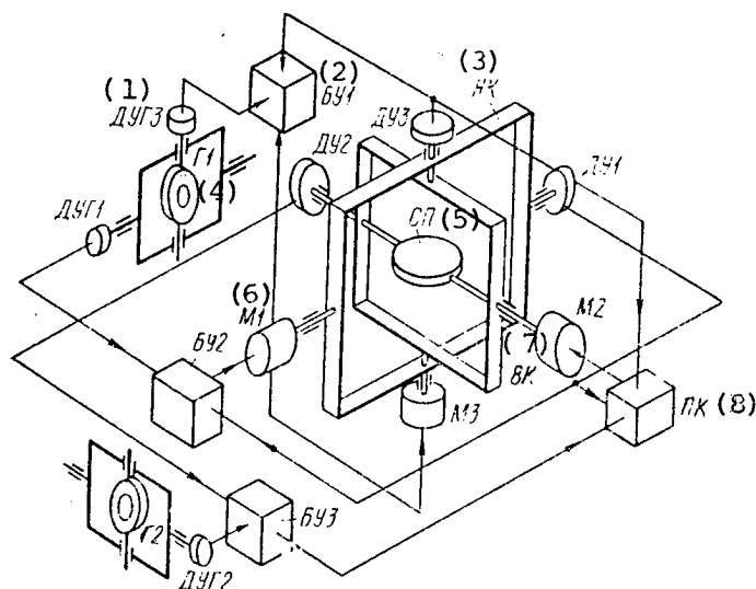
Figure 6.3. Layout of Three-Axis Gyro-Stabilized Platform
