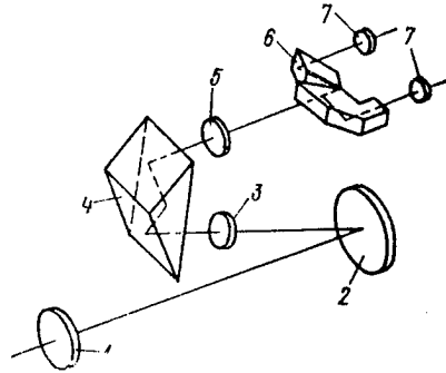
Figure 3.14. Optical Layout of Binoculars: 1--objective; 2--mirror; 3--inversion system; 4--stabilizing prism; 5--additional objective; 6--splitting prisms; 7--eyepieces
