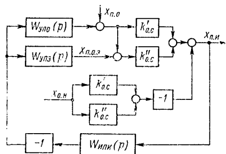
Figure 2.7. Block Diagram of Optical Device With Image Displacement Sensor
