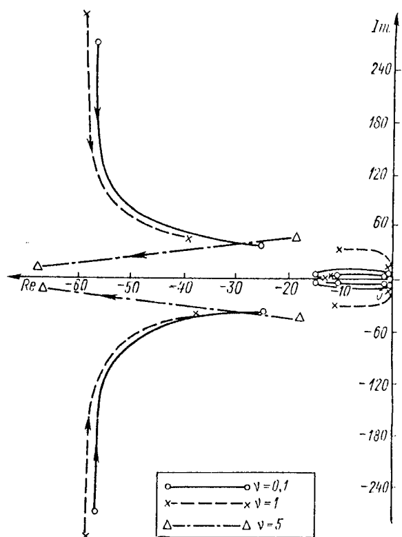
Figure 5.4. Root Hodograph of Two-Channel Control System
