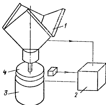
Figure 4.1. Diagram of Laser Gyroscope Array: 1--laser gyroscope array; 2--computer module; 3--drive; 4--relative angular position sensor
