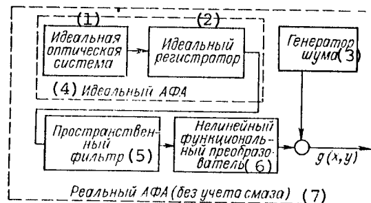
Figure 1.3. Diagram of Shaping of Image in AFA
