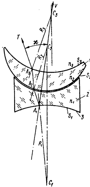
Figure 3.16. Optical Wedge Compensator: 1--movable lens; 2--fixed lens; 3--reflecting surface; n_1, n_2, n_3 --refractive indices of corresponding media; R_1, R_2, R_3 --radii of curvature of surfaces of lenses
