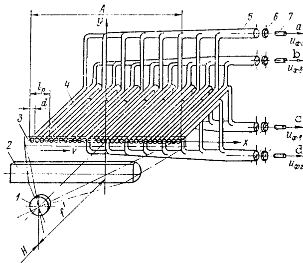
Figure 4.16. Working Principle of Detecting Part of SKSI on Fiber Optic Light Guides: 1--objective; 2--cylindrical lens; 3--image; 4--fiber light guides; 5--bundle of light guides; 6--collecting lens; 7--photoelement
