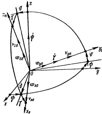
Figure 1.5. Coordinate System of Moving Base
