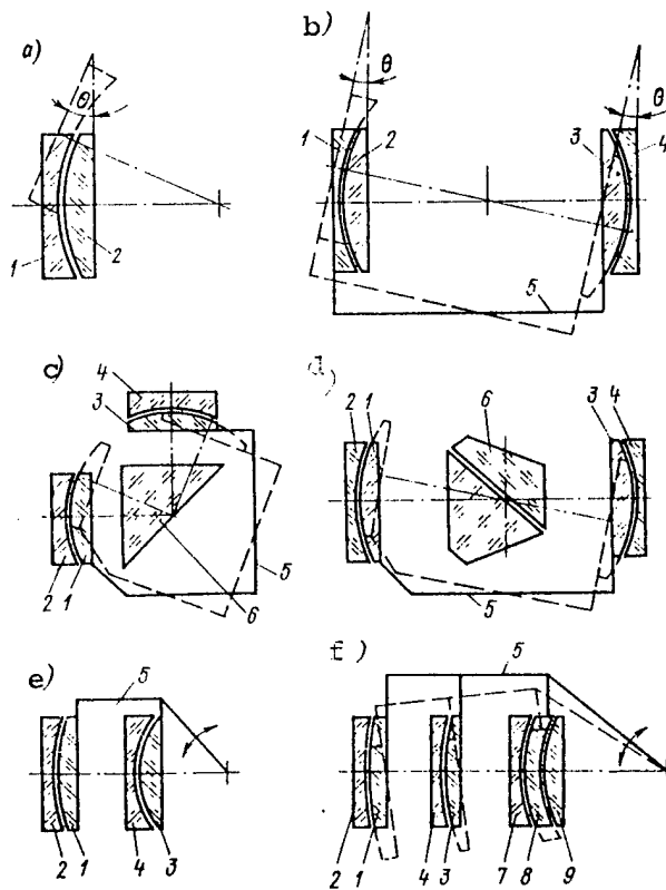
Figure 3.2. Layouts of Stabilization Devices With Optical Wedges, Formed: a--by one pair of lenses; b, c, d, e--by two pairs of lenses; f--by three pair of lenses; 1, 3, 8--movable lenses; 2, 4, 7, 9--fixed lenses; 5--mechanical coupling; 6--rotating element
