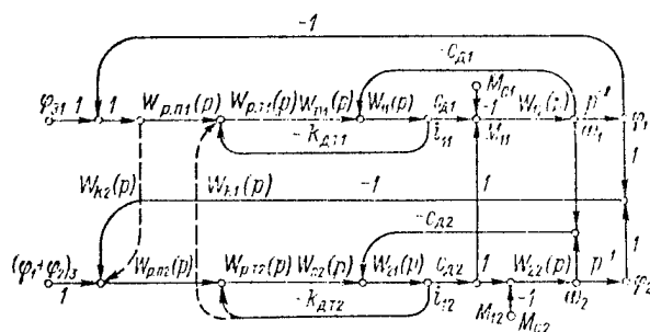
Figure 5.5. Normalized Signal Graph of Two-Channel Control System
