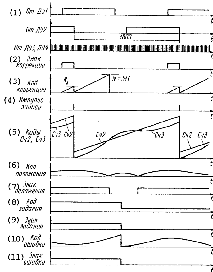
Figure 6.22. Graphs of Time Processes in System
