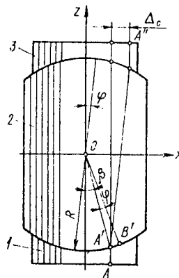
Figure 3.20. Stabilization Device With Three Combined Fiber Optic Lenses: 1, 2, 3--fiber optic lenses
