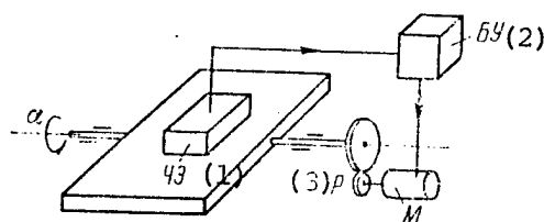
Figure 6.7. Layout of One-Axis Indicating Gyro Stabilizer
