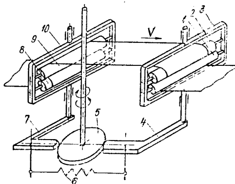
Figure 3.30. Film Displacement Assembly: 1, 2, 8, 9--rollers; 3, 10--frames; 4, 7--levers; 5--eccentric, 6--spring
