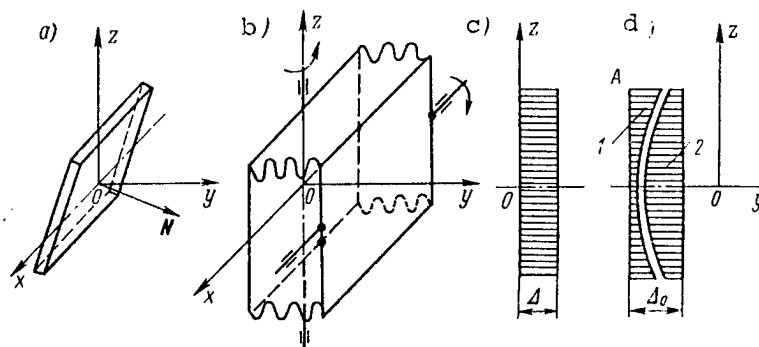
Figure 2.8. Layouts of Main Image Misalignment Compensation Devices: a--coordinate system of flat mirror; b--wedge with variable refracting angle; c--planoparallel fiber optic element (VOE); d--image misalignment compensator using VOE; 1, 2--parts of compensator
