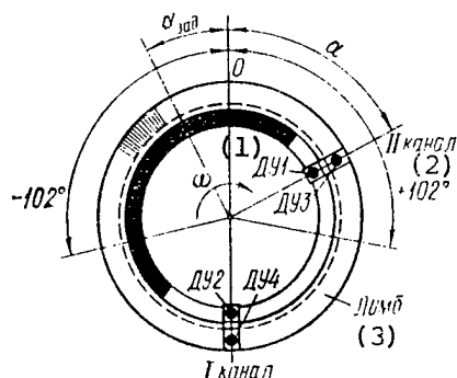
Figure 6.20. Pulse Sensor of Angular Position of Mirror
