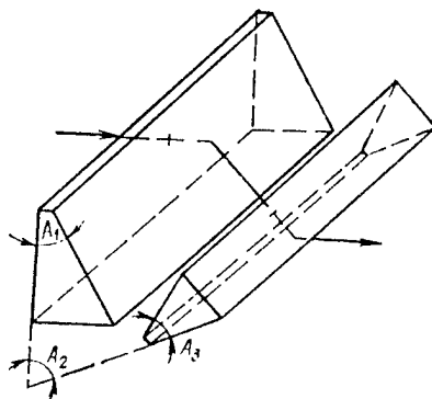
Figure 3.18. Layout of Brewster-Amichi Prism: A_1 and A_3 --angles at vertex of prisms; A_2 --total angle
