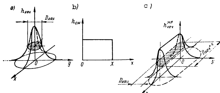
Figure 1.4. Characteristics of Image Blurring: a--equivalent scattering function of point in AFA; b--function of blurring point along one coordinate; c--spatial function of blurring of point
