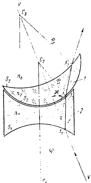
Figure 3.1. Optical Wedge Formed by Two Lenses: 1--moving; 2--fixed
