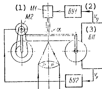
Figure 6.17. Layout of AFA With Two-Coordinate Image Shift Rate Sensor
