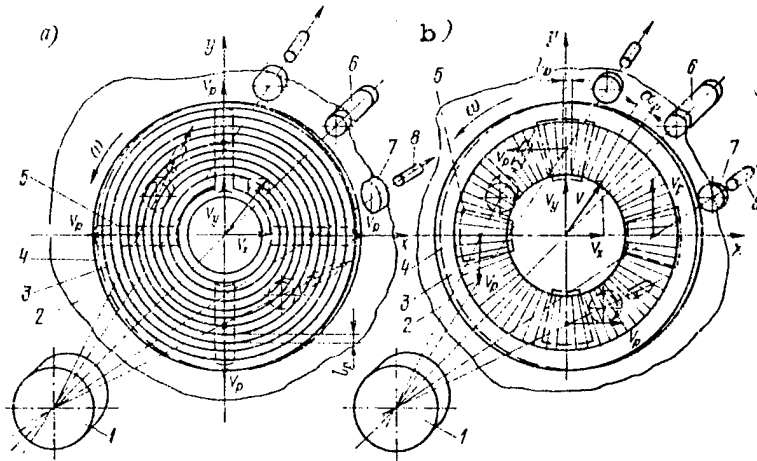
Figure 4.17. Working Principle of Photodetector Part of SKSI With Spatially Fixed Optical-Mechanical Modulator: a--with helical pattern array; b--with radial pattern array; 1--objective; 2--image; 3--modulator disk; 4--diaphragm; 5--diaphragm window; 6--electric motor; 7--collecting lens; 8--photoelement
