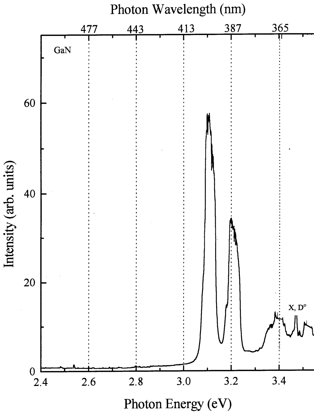
Figure IV-2. PL spectrum of as-grown GaN excited with the 333.6-363.8 nm multiline and sample temperature of 2 K. X represents the exciton and D° is the neutral donor.
