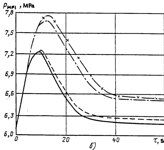
Figure 3. Calculated Curves of Variation in Pressure in Pressurizer (a) and Main Feedwater Inlet (b) in the Closed SRK Regime Using ALR: 1- Start of a refueling cycle, all steam dumps operating; 2-End of a refueling cycle, all steam dumps operating; 3-Start of a refueling cycle, minus four of the BRU-K steam dumps; 4- end of a refueling cycle, minus four BRU-K steam dumps
