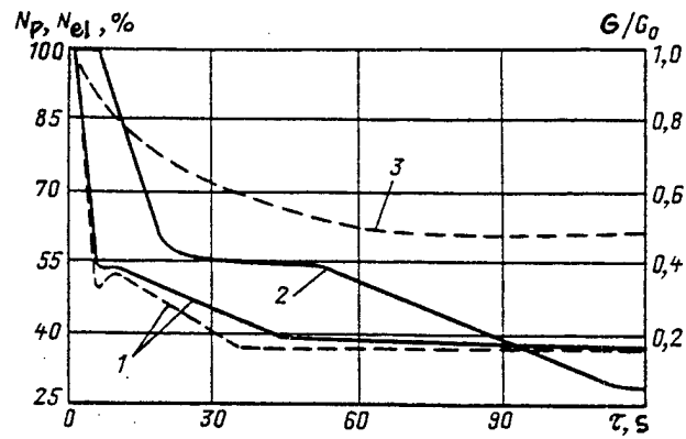
Figure 6. Graph of Variation in Parameters in the Regime Where Two Main Circulating Pumps are Disconnected at the Zaporozhe AES: 1 and 2- Electrical and neutron power; 3-Flowrate through the core; 4 and 5-pressure in the pressurizer and the main feedwater inlet (solid line is experiment, dashed line is calculated)
