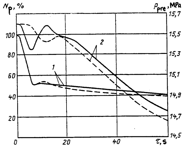
Figure 1. Graph of Variation in Parameters in the Load Shedding Regime Down to No-Load at the Zaporozhe AES: 1-Neutron power; 2 and 3-pressure in main feedwater inlet and pressurizer; 4-temperature on the cold and hot sides; 6-mean temperature in the primary loop (solid line is experiment, dashed line is calculation)
