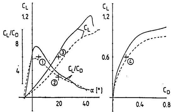
RECTANGULAR WING - CLARK Y Aerofoil Section
