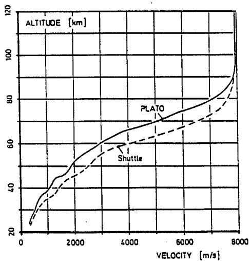
Fig 11 Re-entry profile
