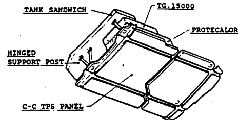
DETAIL OF THERMAL PROTECTION SHIELD PANEL
