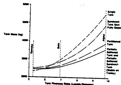
HOTOL Liquid Hydrogen Tank Skin Mass Sensitivity to Fineness Ratio
