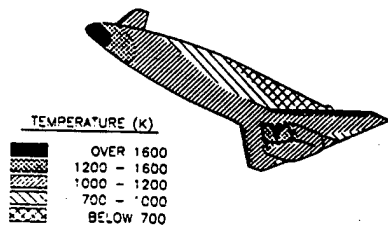
Peak Radiation Equilibrium Temperature Contours for the -0°C vehicle during re-entry.
