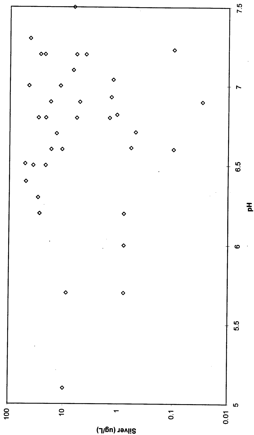
Silver vs pH Scatter Plot
