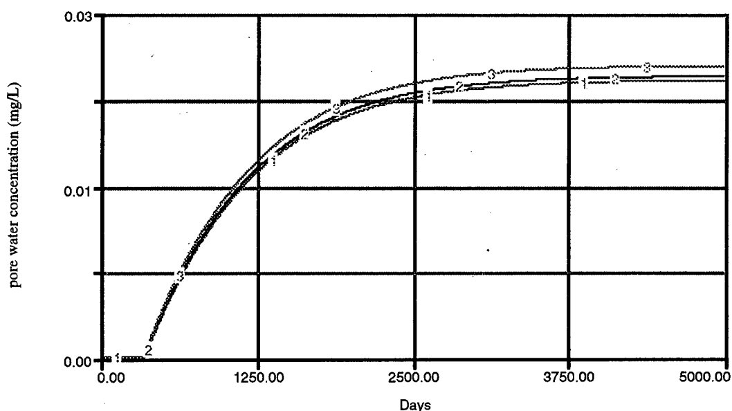
Figure 14. Pore Water Pb Concentration at Transfer Rate = .001, .01, and .1 days -1
