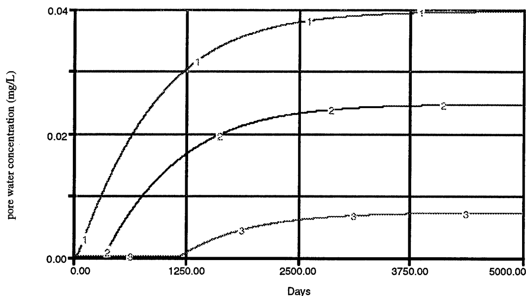
Figure 31. Pore Water Pb Concentration at AVS = 0, 6.25, and 15 \mu\text{mol/g}
