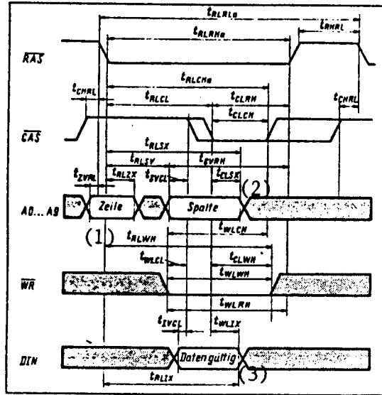
Figure 5. Early Write Cycle (gray areas: level undefined)
