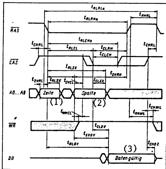
Figure 6. Read Cycle (gray areas: level undefined)
