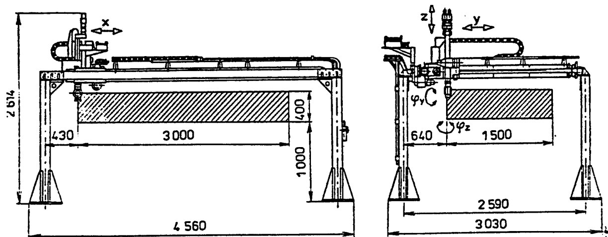
Figure 6. APR 2.5-04 Industrial Robot
