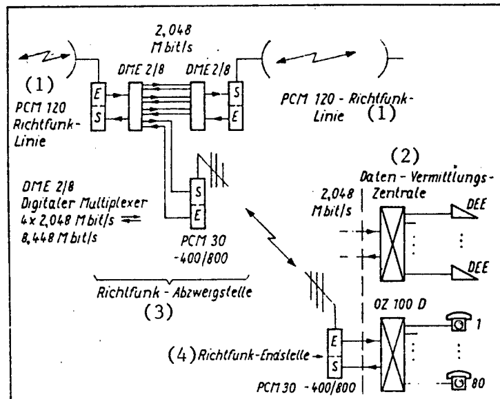
Figure 6. PCM 30-400/800 as transmission path for network spurs in telephone and data networks (example)
