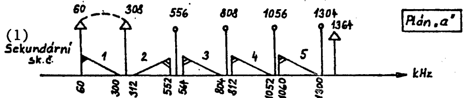
Figure 5. Arrangement of line frequencies involved in the 1.3-MHz system for small coaxial cables—variations involving five secondary groups. Key:—1. Secondary group number.
