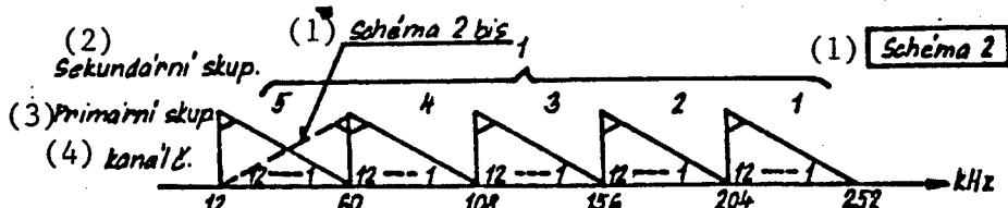
Figure 4. Arrangement of line frequencies for 60-channel carrier frequency telephone systems. Key:—1. Schematic—2. Secondary group—3. Primary group—4. Channel number.
