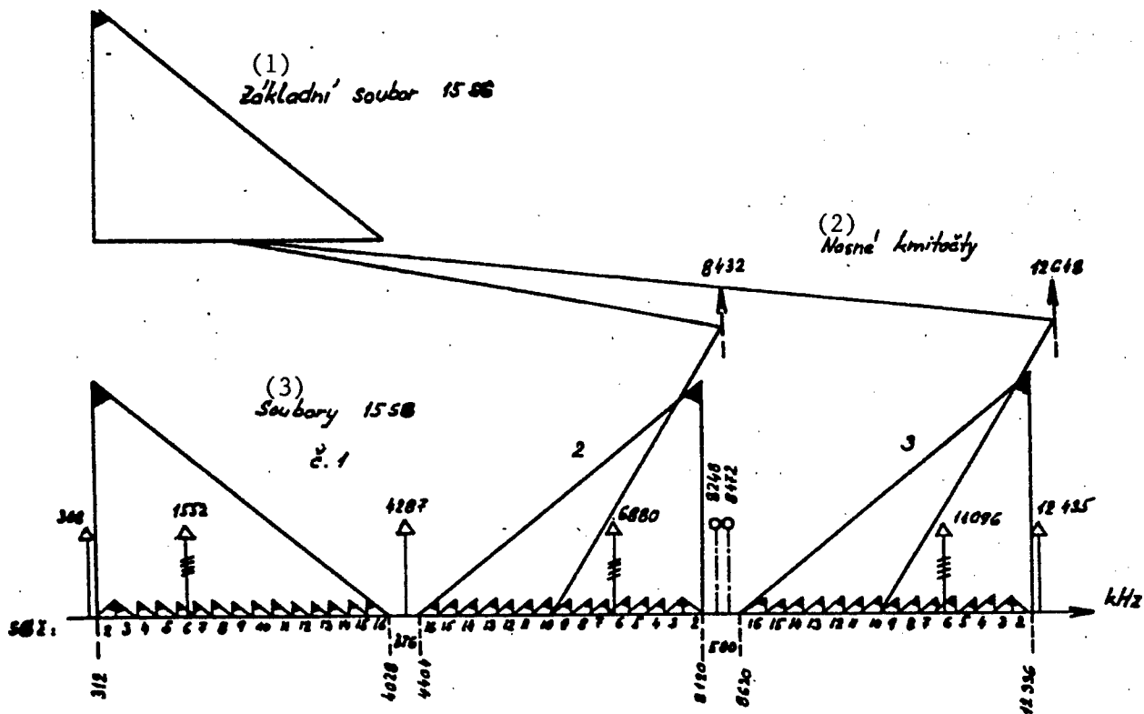
Figure 8. Arrangement of line frequencies for the 12-MHz system.
