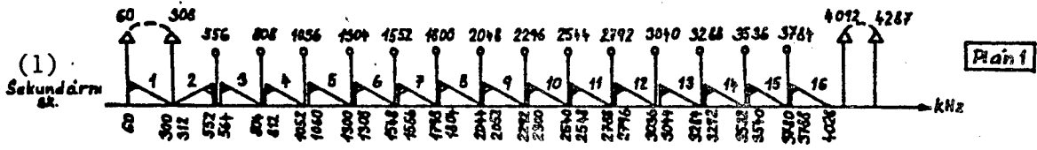
Figure 6. Arrangement of line frequencies involved in the 4-MHz system for small coaxial cables—variation involving 16 secondary groups. Key:—1. Secondary group.
