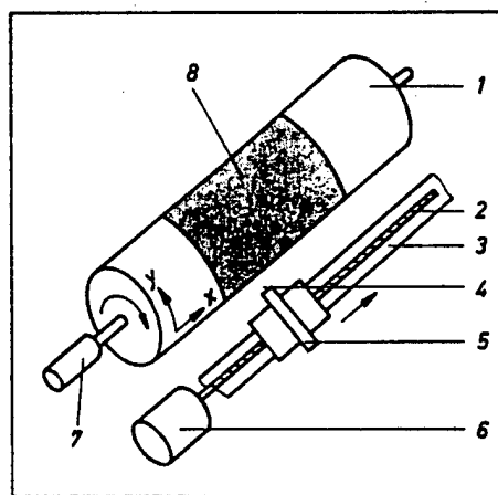
Figure 3. Operating Principle
