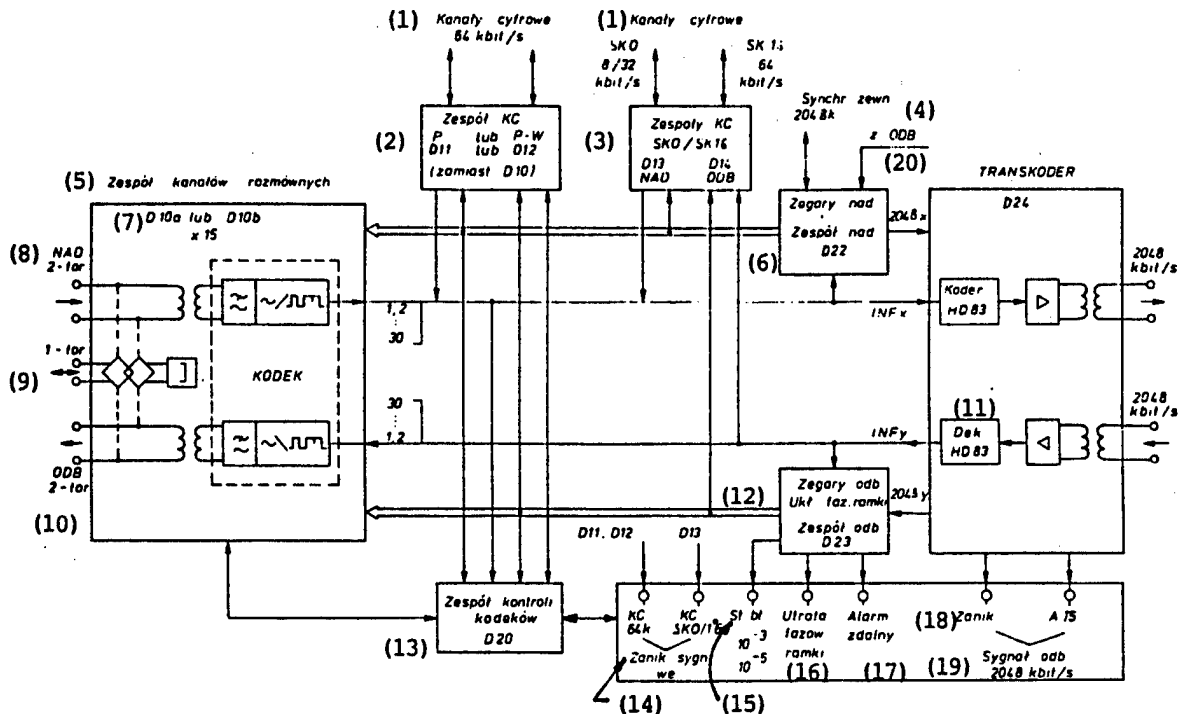
Figure 1. Block Diagram of BK1-TCK30G Multiplexer
