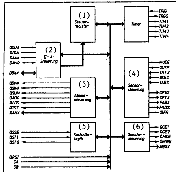
Figure 2. Schematic
