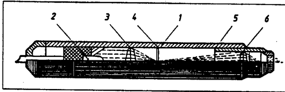
Figure 4. Flash-Unit Attachment
