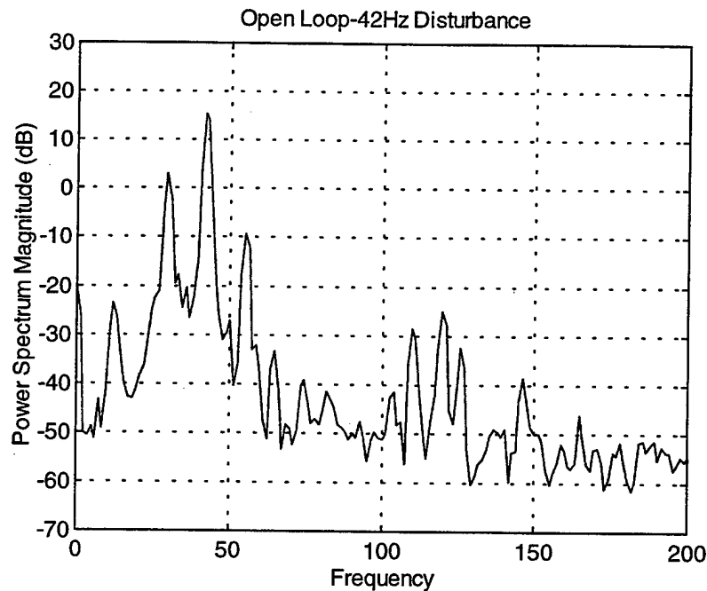
Figure 4.10 Ambient PSD (0-200Hz)
