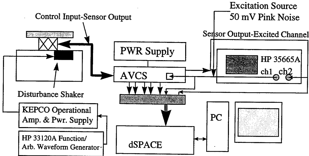
Figure 3.4 Experimental Setup
