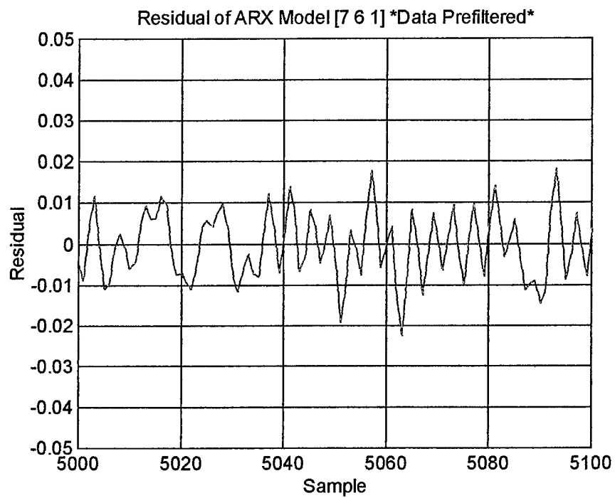
Figure C.6 Residual Vs. Sample
