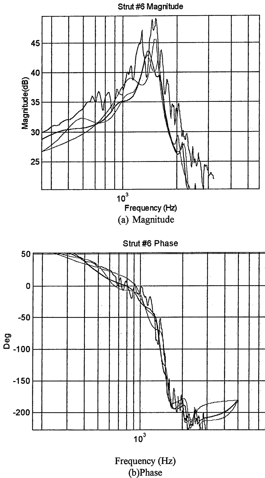
Figure 3.37 ARX Model Frequency Response Comparison Blue=Actuator #6, Red=[7 6 1], Magenta=[15 15 1], Black=[12 12 1]
