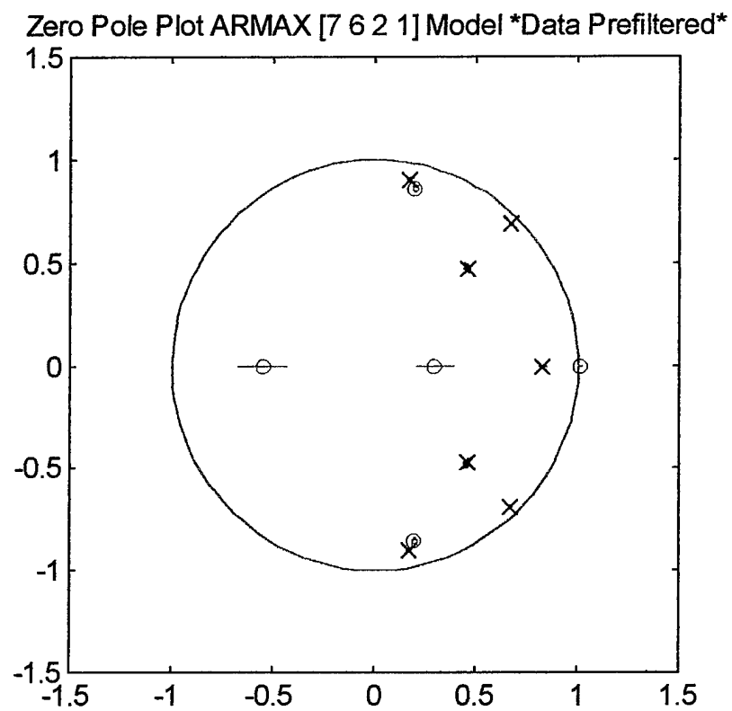
Figure E.6 Zero-Pole Plot
