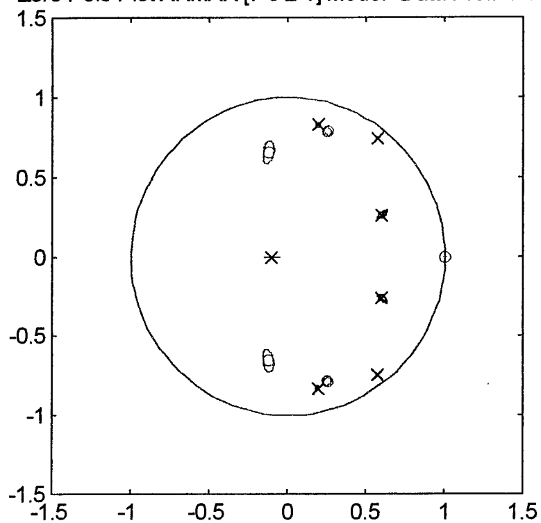
Figure F.6 Zero Pole Plot
