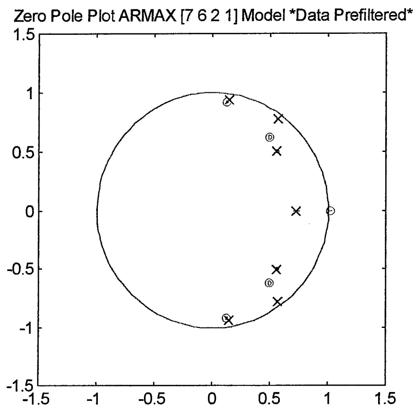
Figure C.6 Zero-Pole Plot
