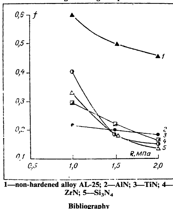
Figure 3. Variation of Friction Coefficient of Like Coatings with Contact Zone Pressure for Coatings Obtained by Electric-Spark Hardening of the Aluminum Alloy With High-Melting Compounds
