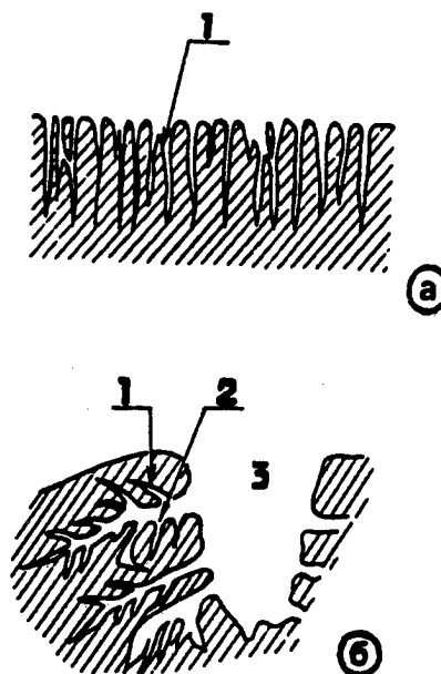
Models of Porous Structures of Carbon Fiber Adsorbents (a) and Granular Active Carbons (b)
