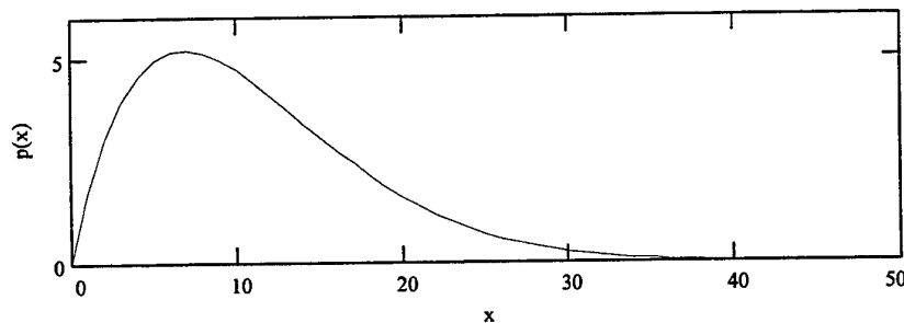
Figure A.5 An example of the Rician function
