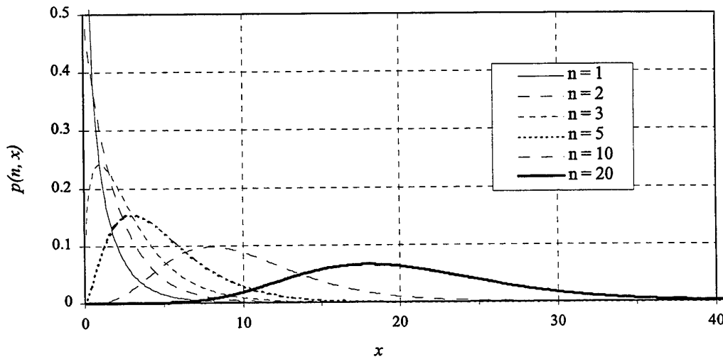
Figure A.6 Examples of the \chi^2 function
