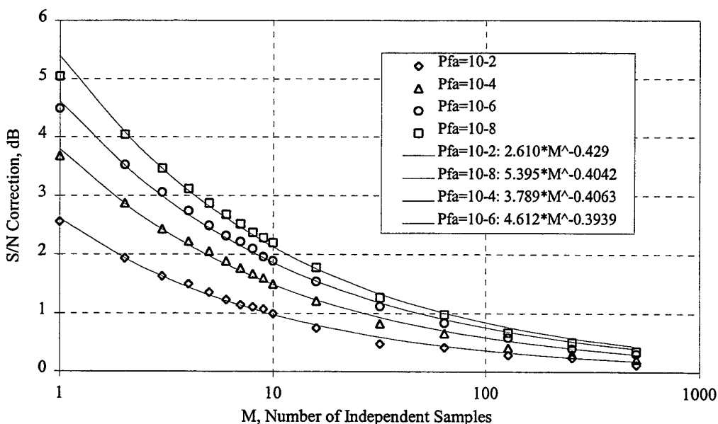
Figure C.2 Finite wt+1 correction to Gaussian approximation of DT for power detection of a sinusoid in Gaussian noise, P_{fa}=10^{-8}, 10^{-6}, 10^{-4} and 10^{-2} with P_d=50\% , with curve fits.
