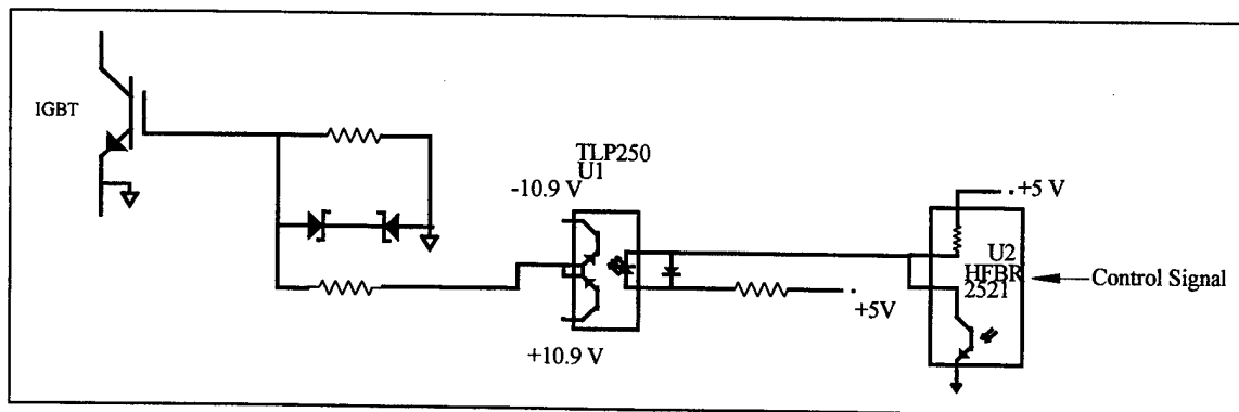
Figure 2-4, Simplified IGBT driver circuit.
