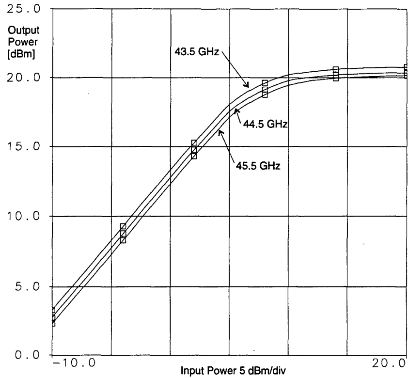
Figure 39: Large signal saturation performance of the amplifier with interconnects (after EM optimization).
