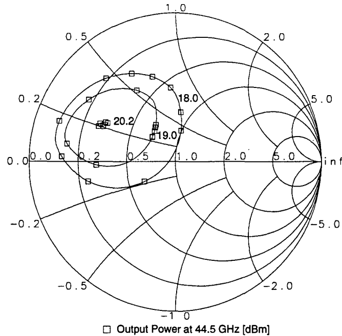
Figure 5: Load pull contours of 300 \mu\text{m} device (12 dBm input power).
