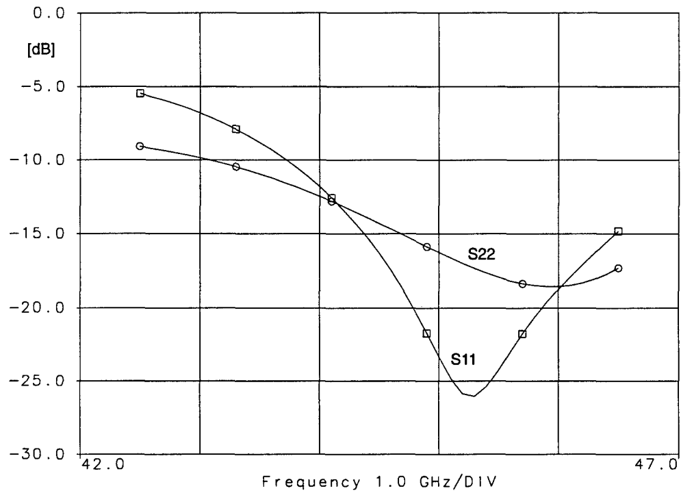
Figure 24: Input and output match of the two-stage amplifier.
