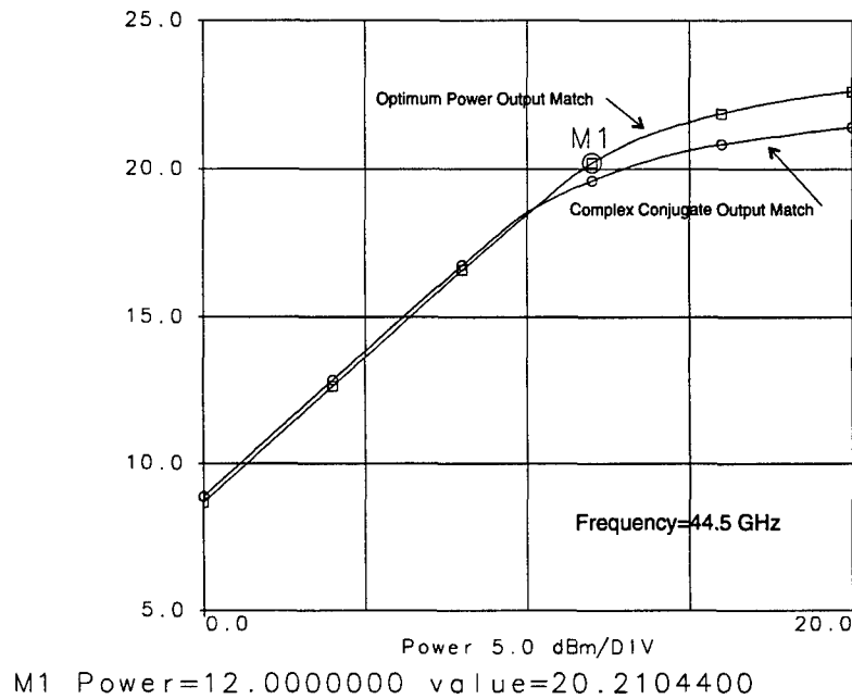
Figure 6: Comparison of output power for optimum power load and conjugately matched load for a 300 \mu\text{m} device.
