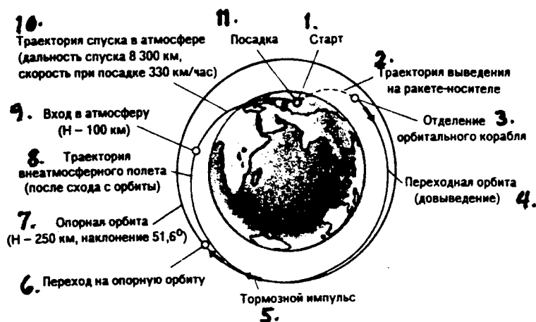
Ballistics of Buran flight
