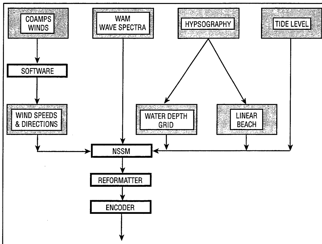
Fig. 27 — Basic NSSM modeling flow adopted for SE4
