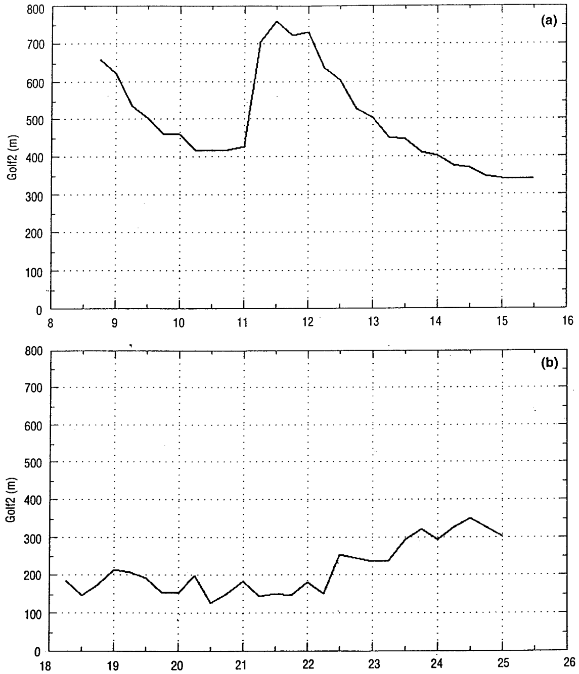
Fig. 24 — NSSM surf zone width for (a) January 1995 and (b) August 1995
