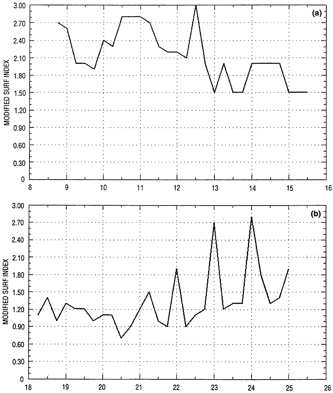
Fig. 25 — NSSM Modified Surf Index for (a) January and (b) August 1995
