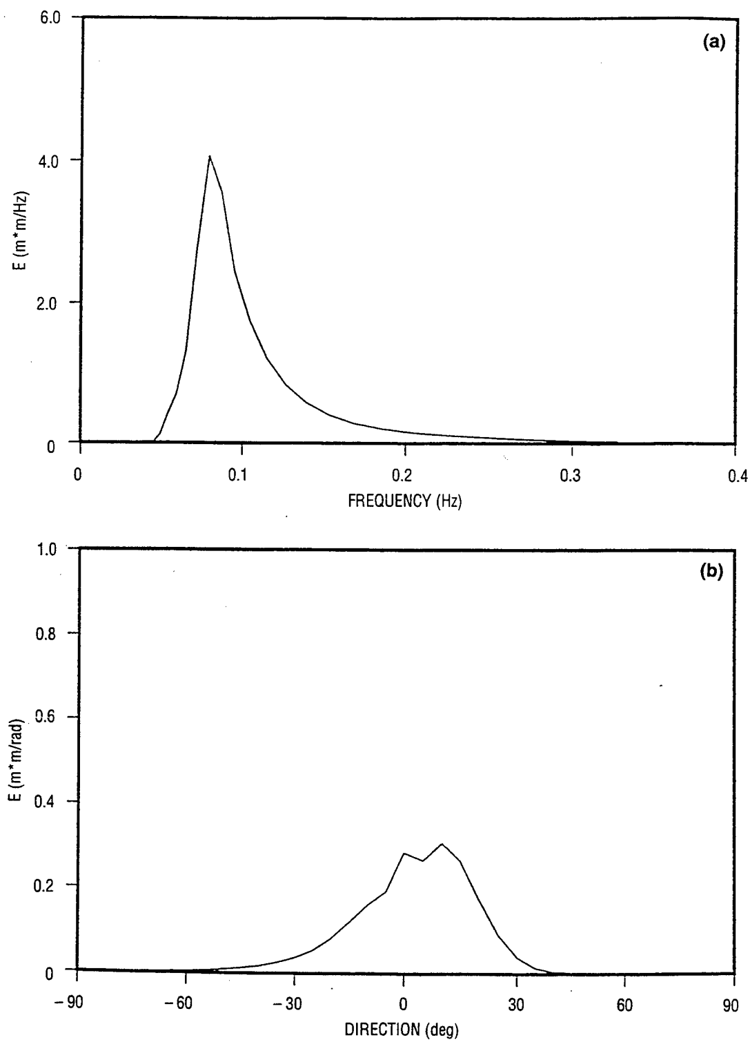
Fig. 15 — Transformed STWAVE distribution of energy at 9-m depth, (a) frequency and (b) directional
