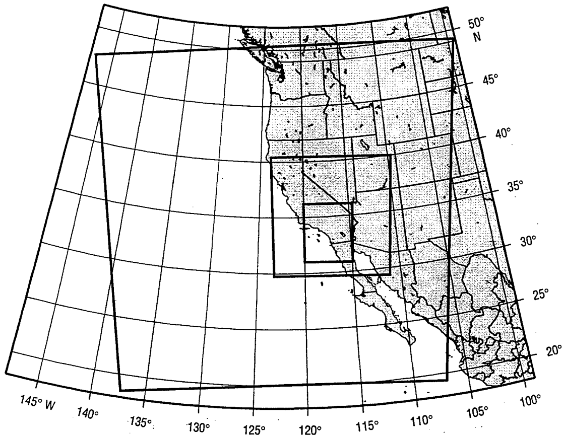
Fig. 1 — COAMPS triple-nested grid with resolutions of 45/15/5 km
