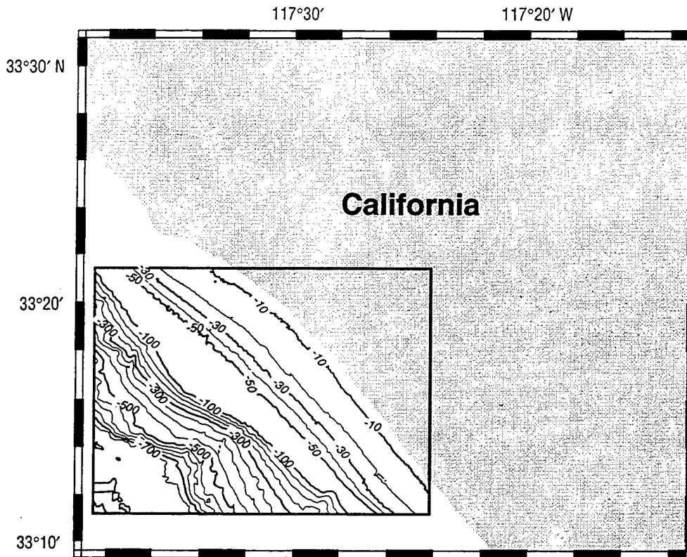
Fig. 9 — Southern California coast with inset Synthetic Environment 4 (SE4) demonstration area
