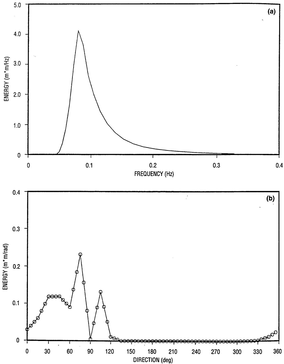
Fig. 13 — WAM distributions of wave energy for 8 Jan 1995, (a) frequency and (b) directional
