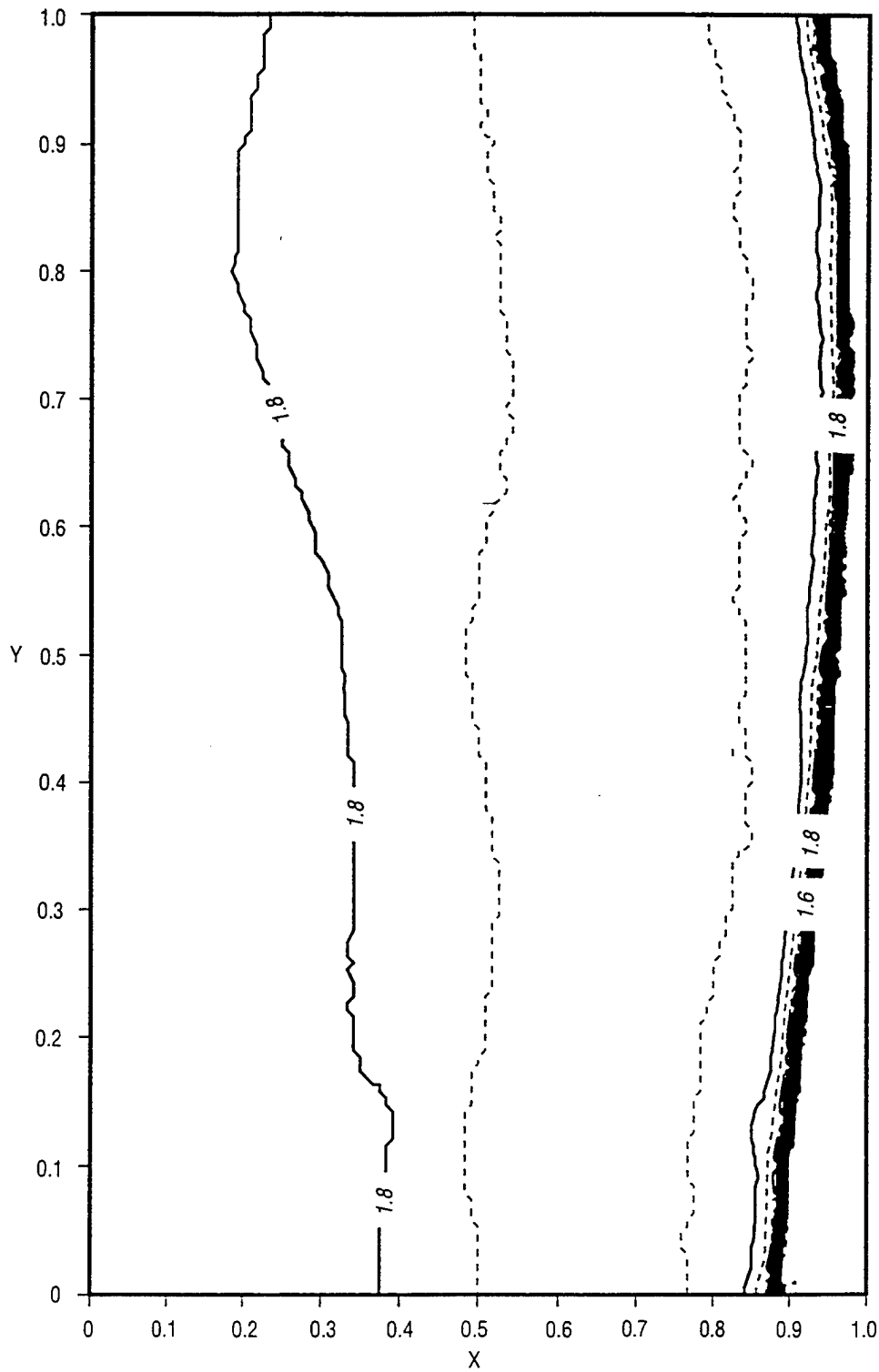
Fig. 19 — Wave height contours (m) for 8 Jan 1995 18Z
