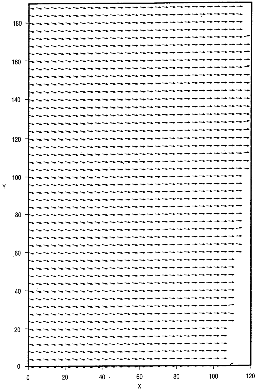
Fig. 20 — Wave direction vectors for 8 Jan 1995 18Z
