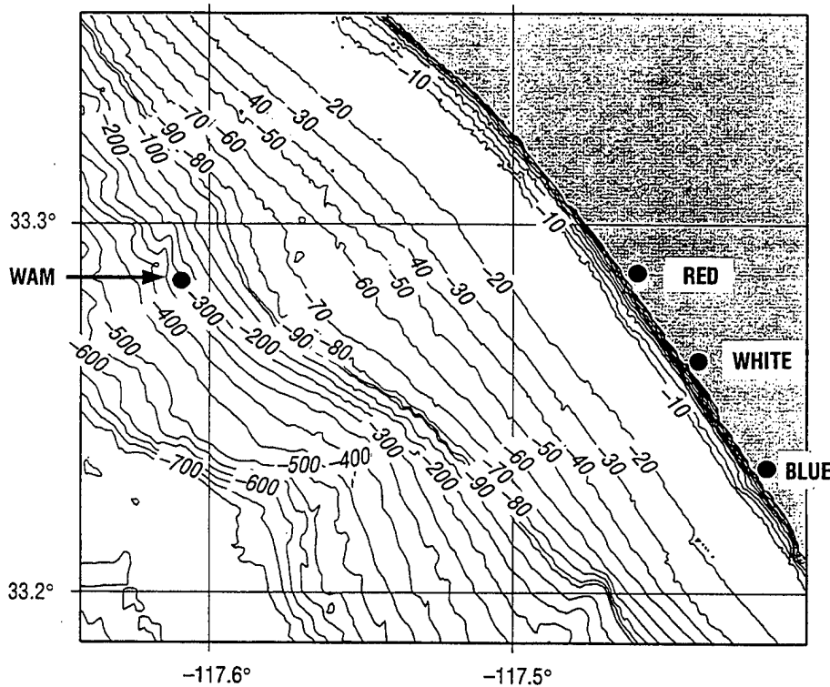
Fig. 10 — Camp Pendleton bathymetry used in JDSZEM modeling. Bathymetry has a horizontal resolution ( dx = dy ) of 100 m
