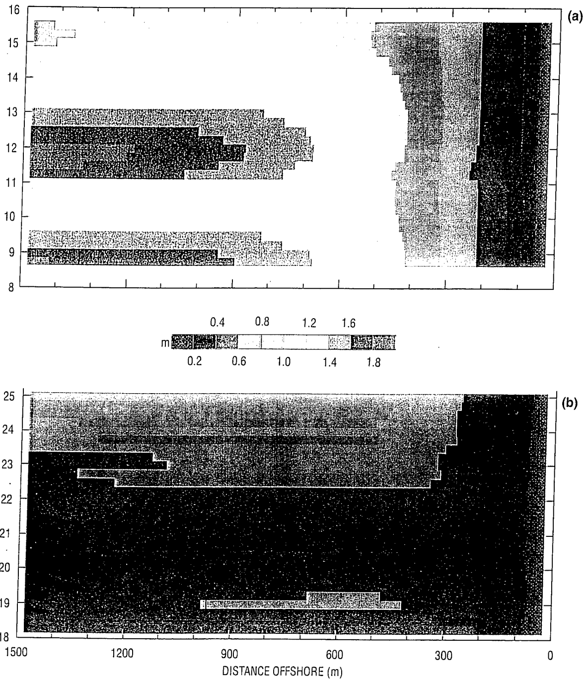
Fig. 21 — Navy Standard Surf Model (NSSM) significant breaker height for (a) January and (b) August 1995
