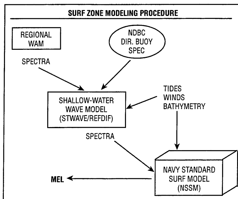
Fig. 28 — Proposed JDSZEM modeling flow for FY97 effort
