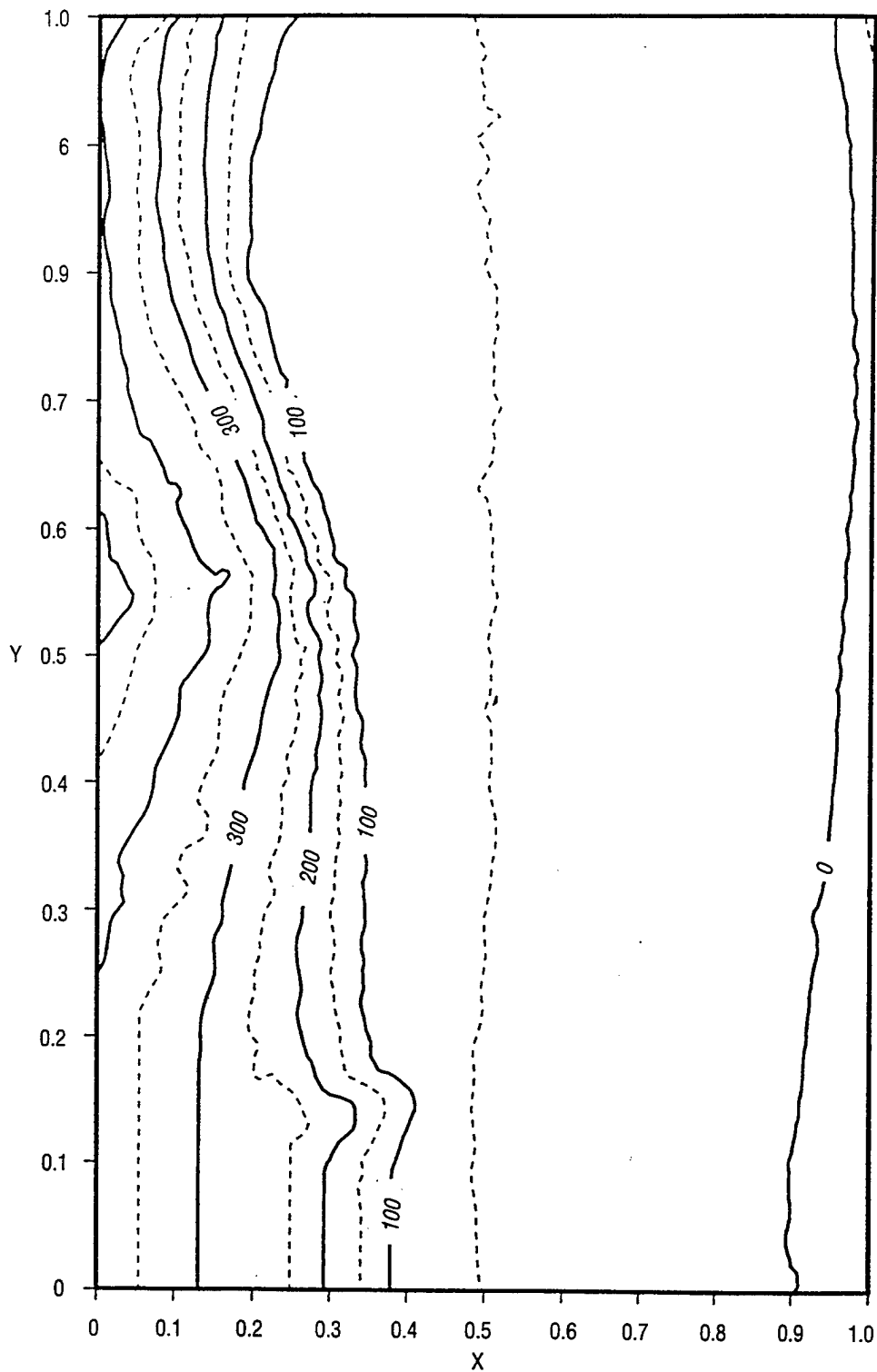
Fig. 12 — Camp Pendleton bathymetry used in STWAVE grid. Solid lines denote contours at 100-m intervals. The 0-m isobath represents the shoreline.
