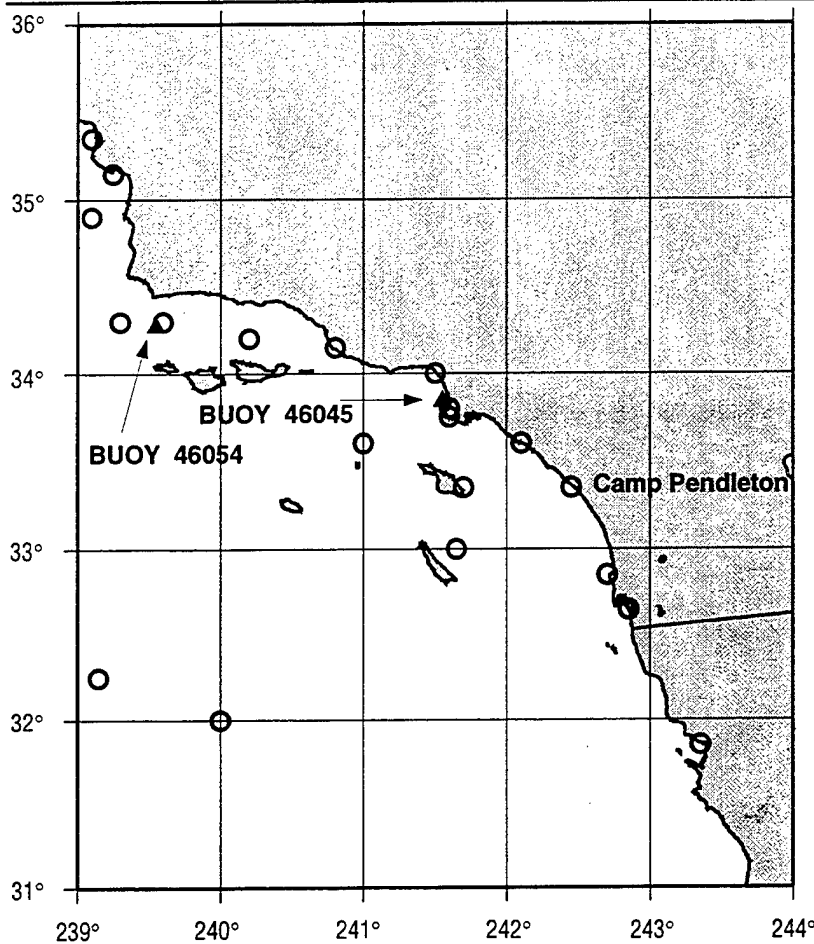
Fig. 5 — Southern California regional WAM domain. Model resolution is 0.05^\circ ; open circles denote locations where WAM spectra were saved; solid triangles denote buoy locations.
