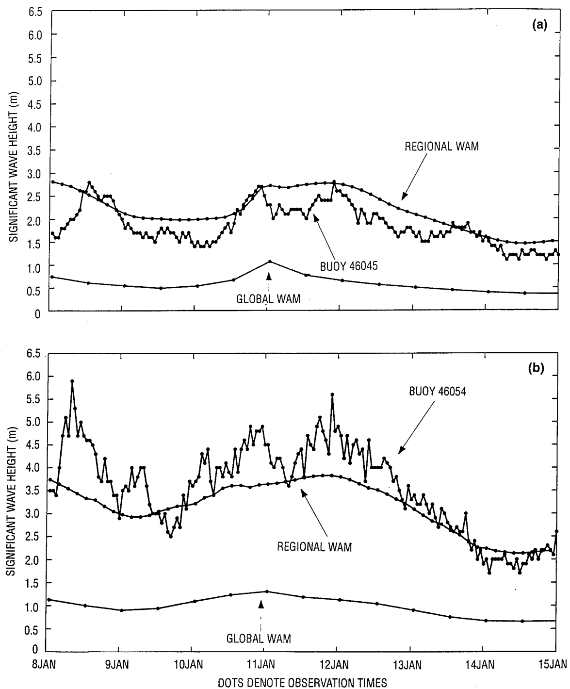
Fig. 6 — Comparison of significant wave height for 1.25° global WAM (12-hourly), regional WAM (6-hourly), and NDBC (hourly), (a) 33.84° N, -118.45° E and (b) 34.27° N, -120.45° E
