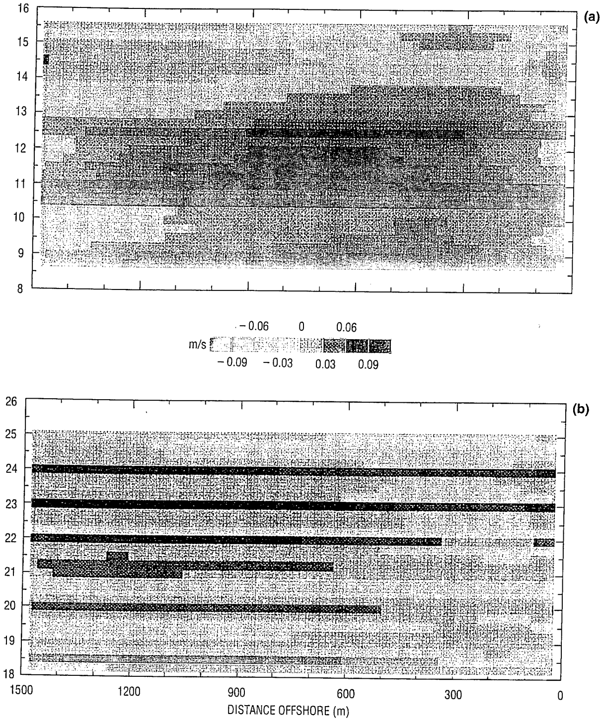
Fig. 23 — NSSM longshore current for (a) January and (b) August 1995
