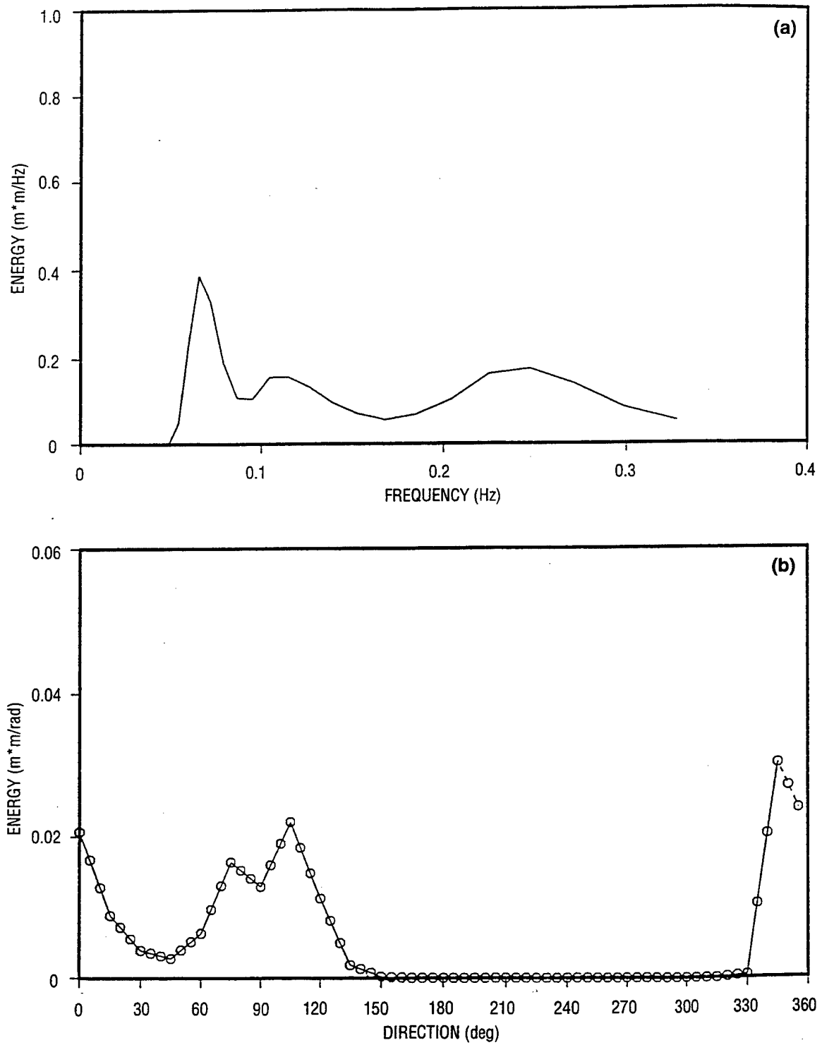
Fig. 14 — WAM distributions of wave energy for 22 Aug 1995, (a) frequency and (b) directional
