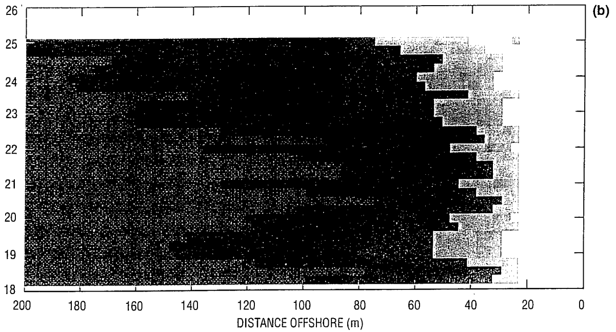
Fig. 22 — NSSM percent breaking waves for (a) January and (b) August 1995
