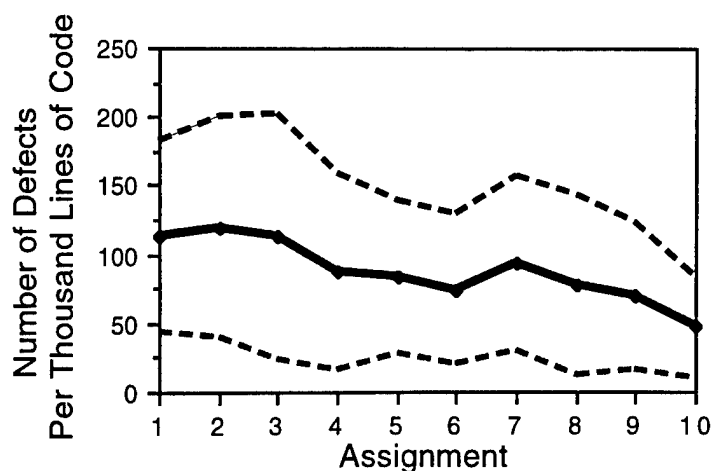
Figure A-3: Average Defect Density
