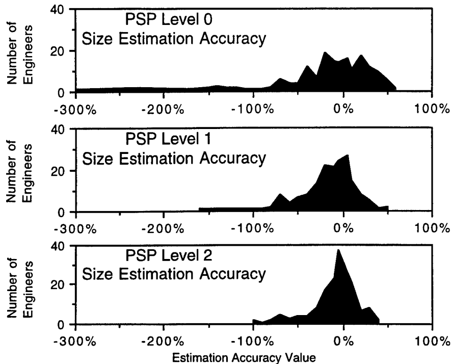
Figure 4-1: Distributions of Size Estimation Accuracy by PSP Level
