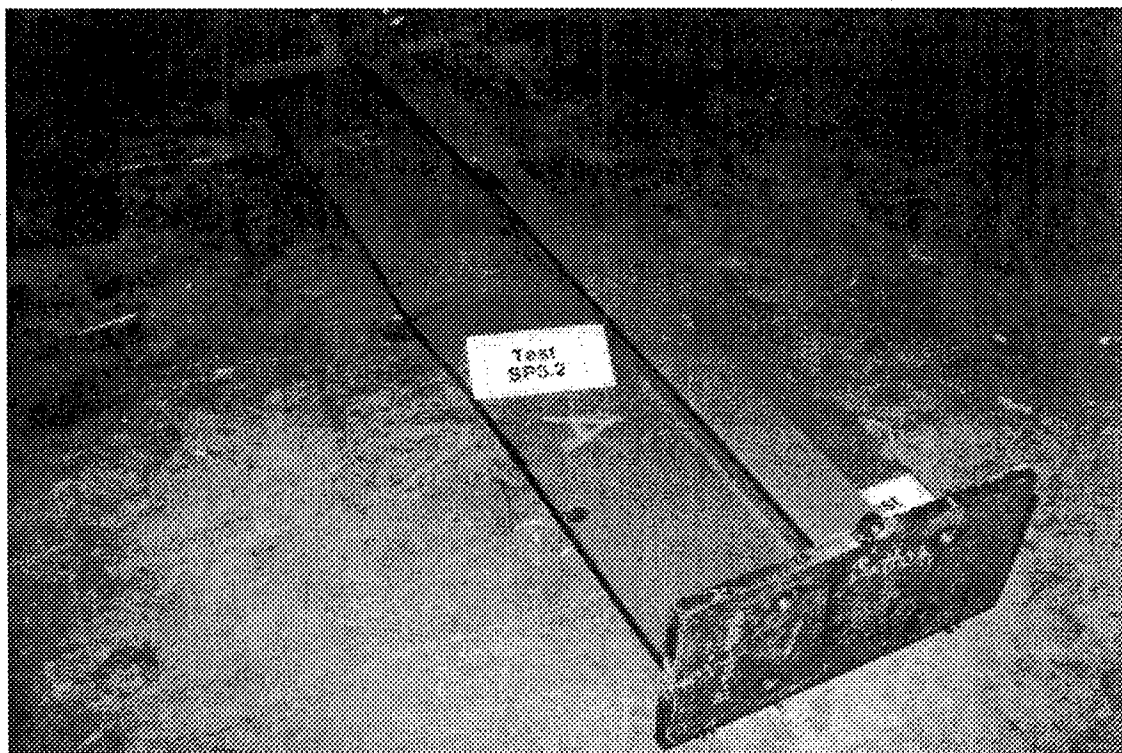
Figure 16: Final deformed shapes of SP3.2
