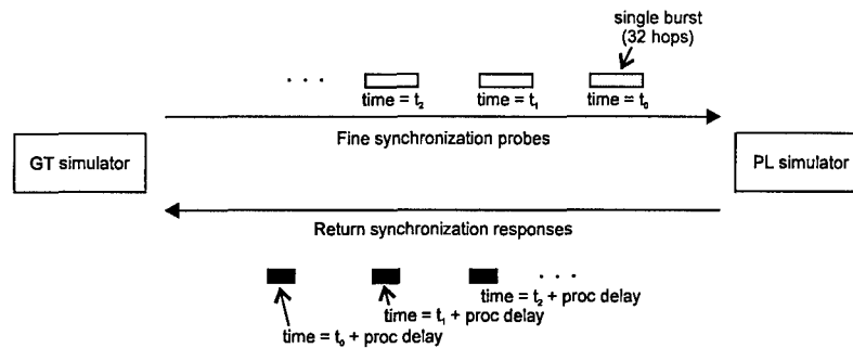
Fig. 1.4 Data flow of the fine synchronization process
