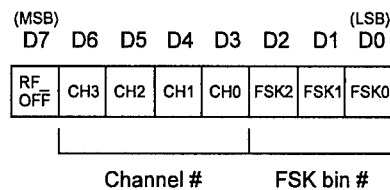
Fig. A1. Format of transmit data interface
